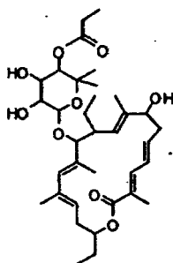
Compound 107, RRT ratio 1.39
