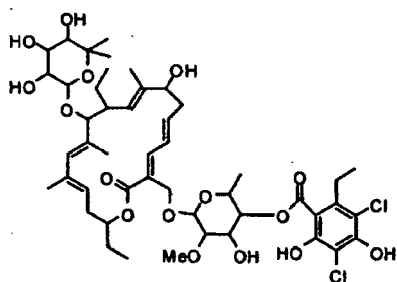
Compound 102, RRT ratio 0.81
