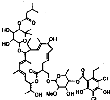
Compound 105, RRT ratio 1.19
