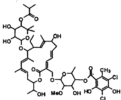
Compound 109, RRT ratio 0.89
