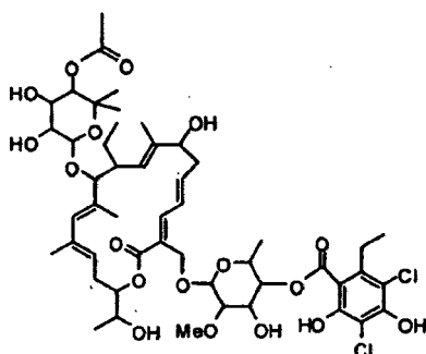
Compound 101, RRT ratio 0.71
