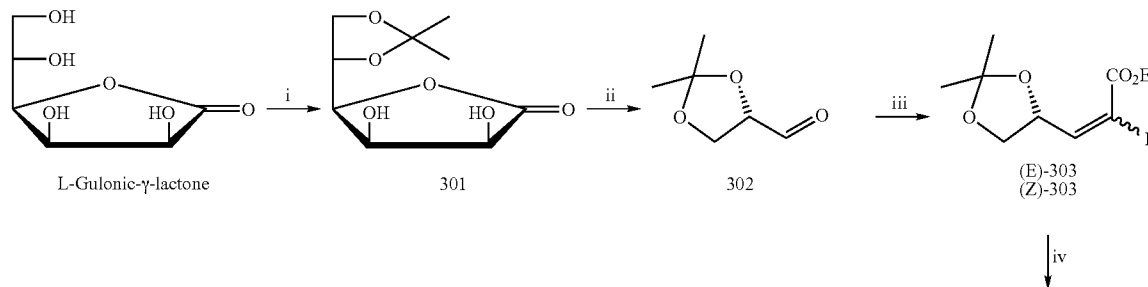
Scheme 9
