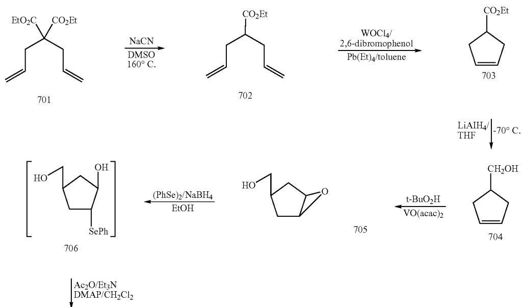
Scheme 11
