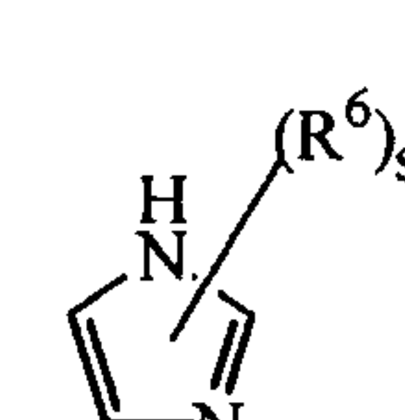
(a-14)
