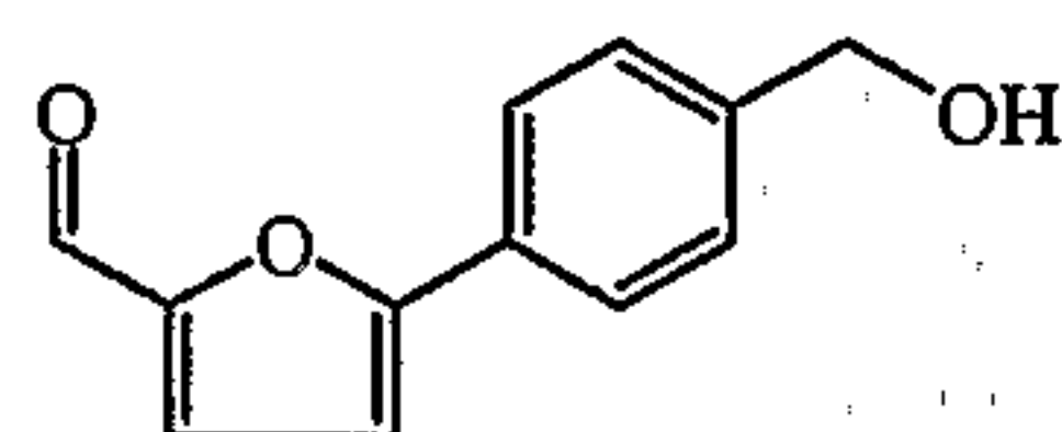
intermediate 16
