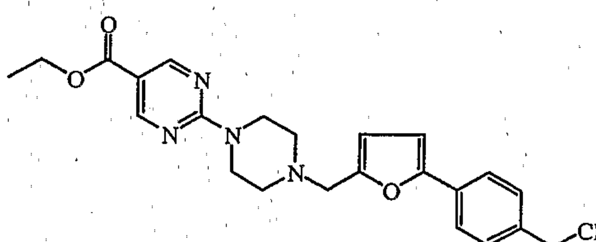
intermediate 20
