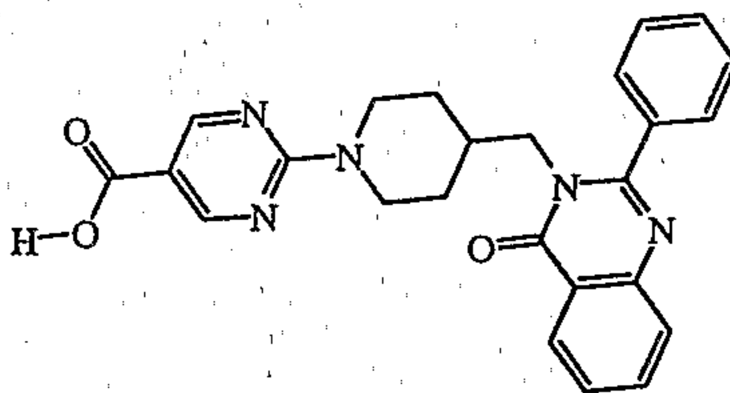
intermediate 22
