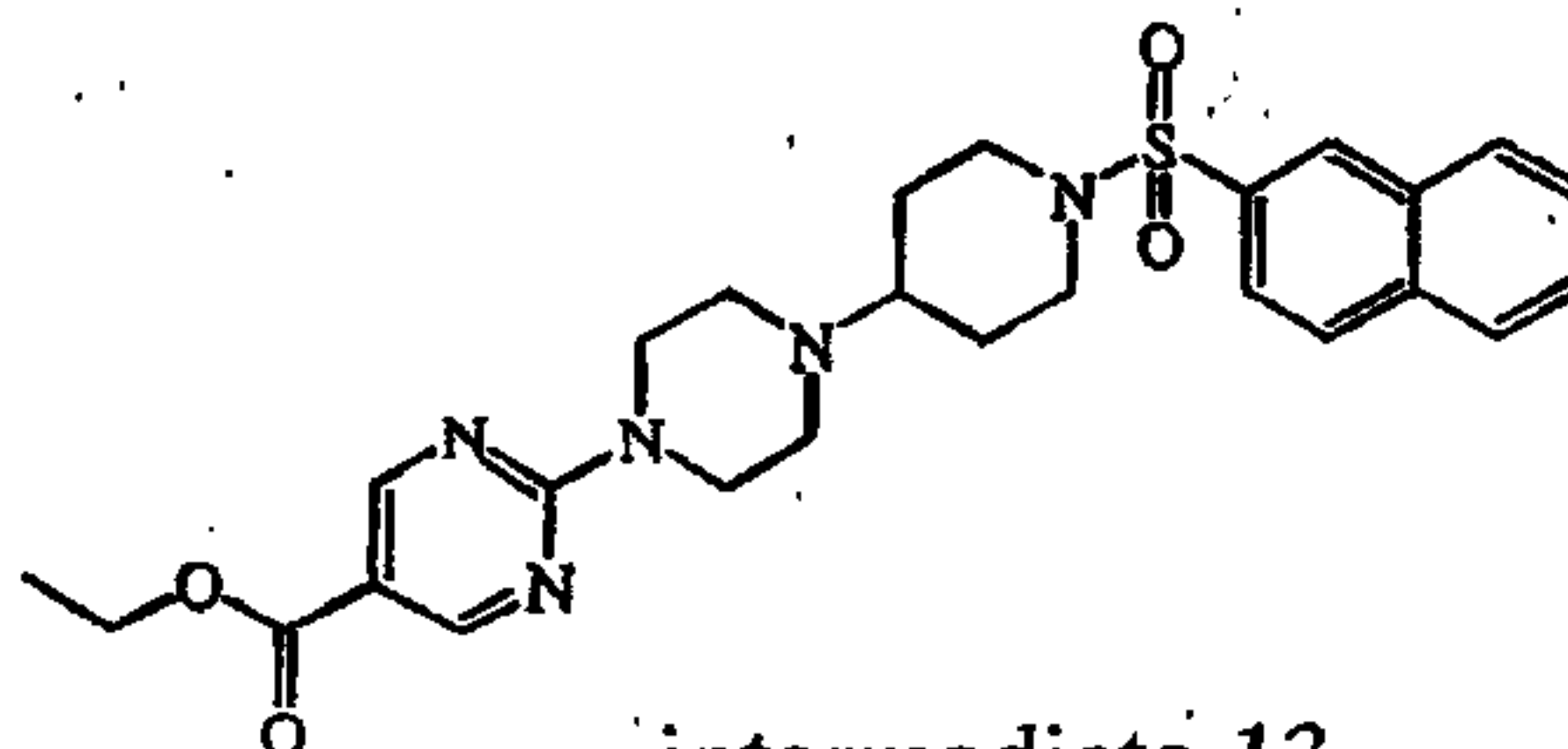
intermediate 13
