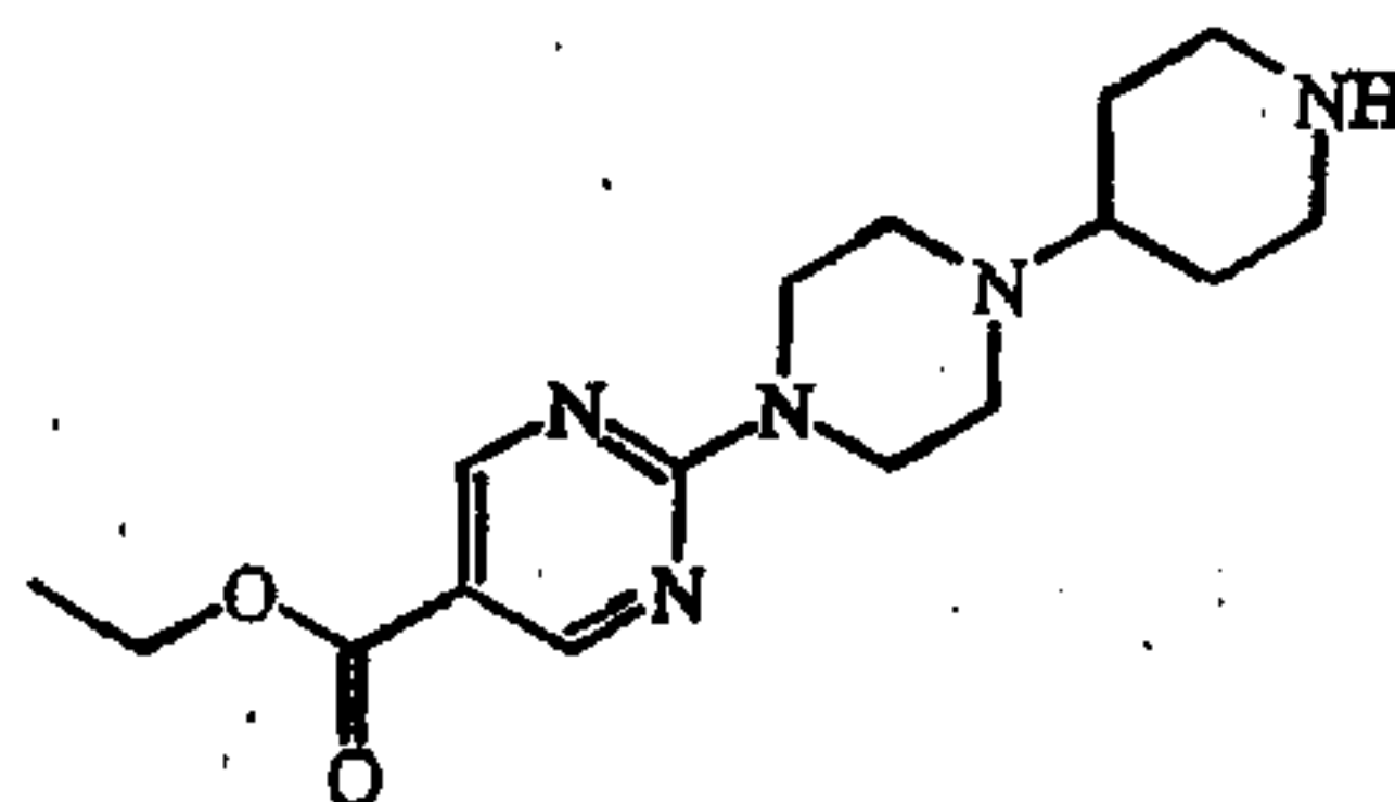
.HCl intermediate 12
