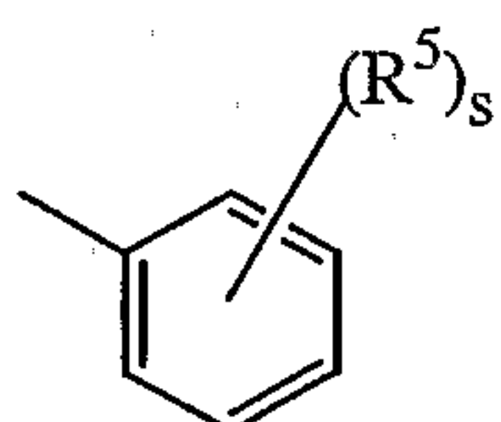
(a-1)
