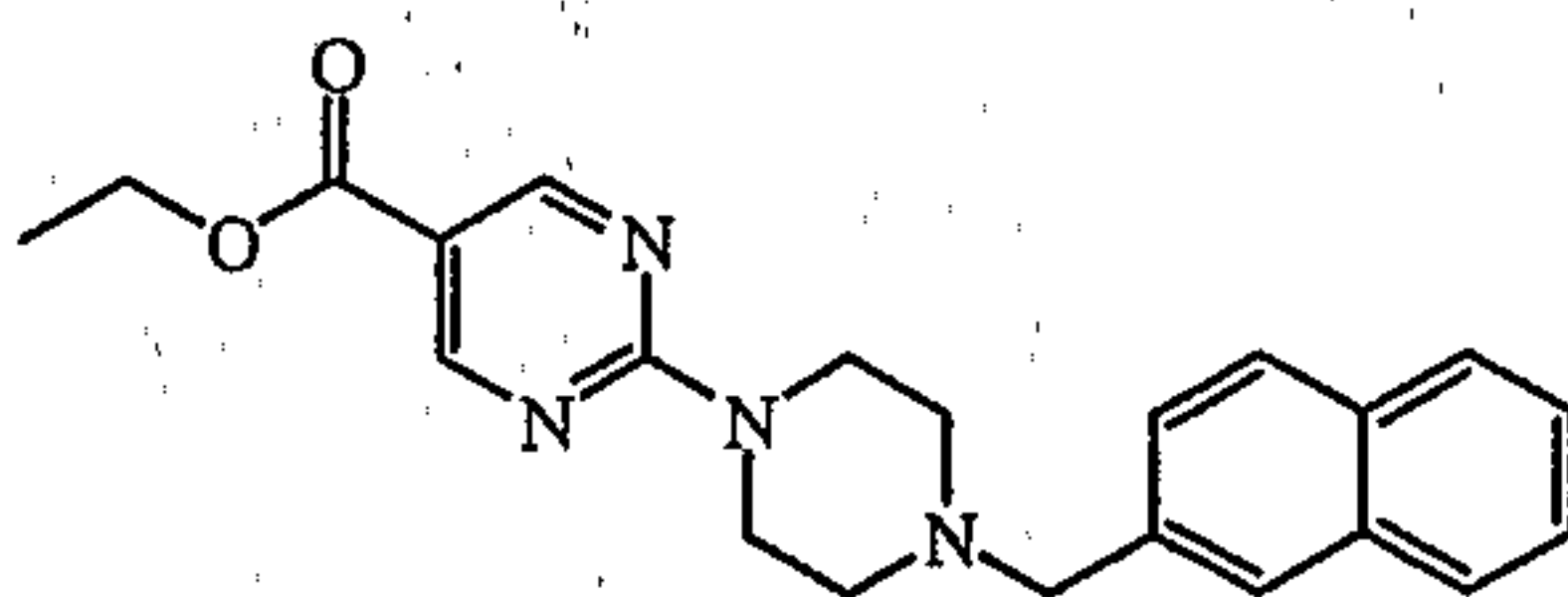
intermediate 28
