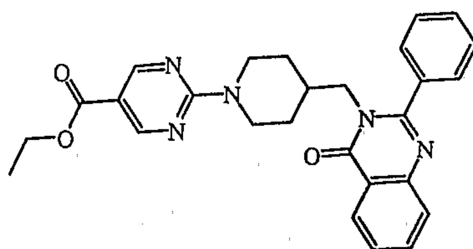
intermediate 21
