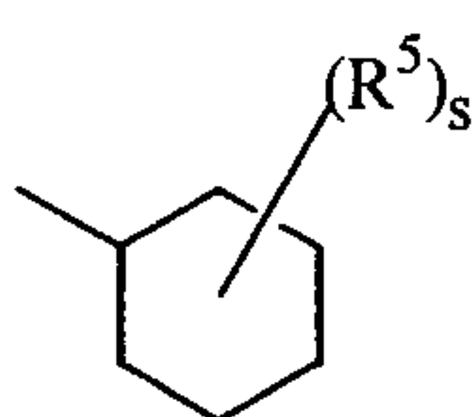
(a-2)
