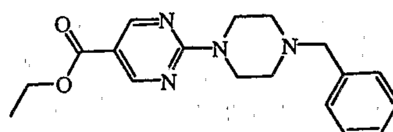
intermediate 9
