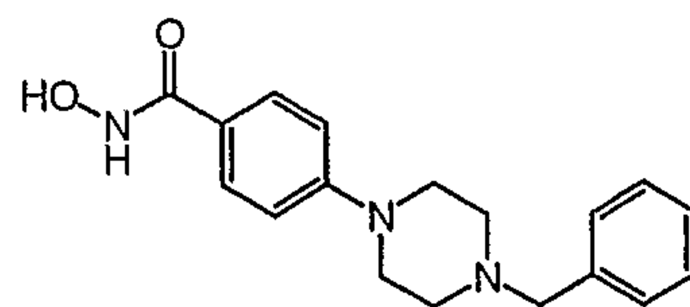
Compound 2
