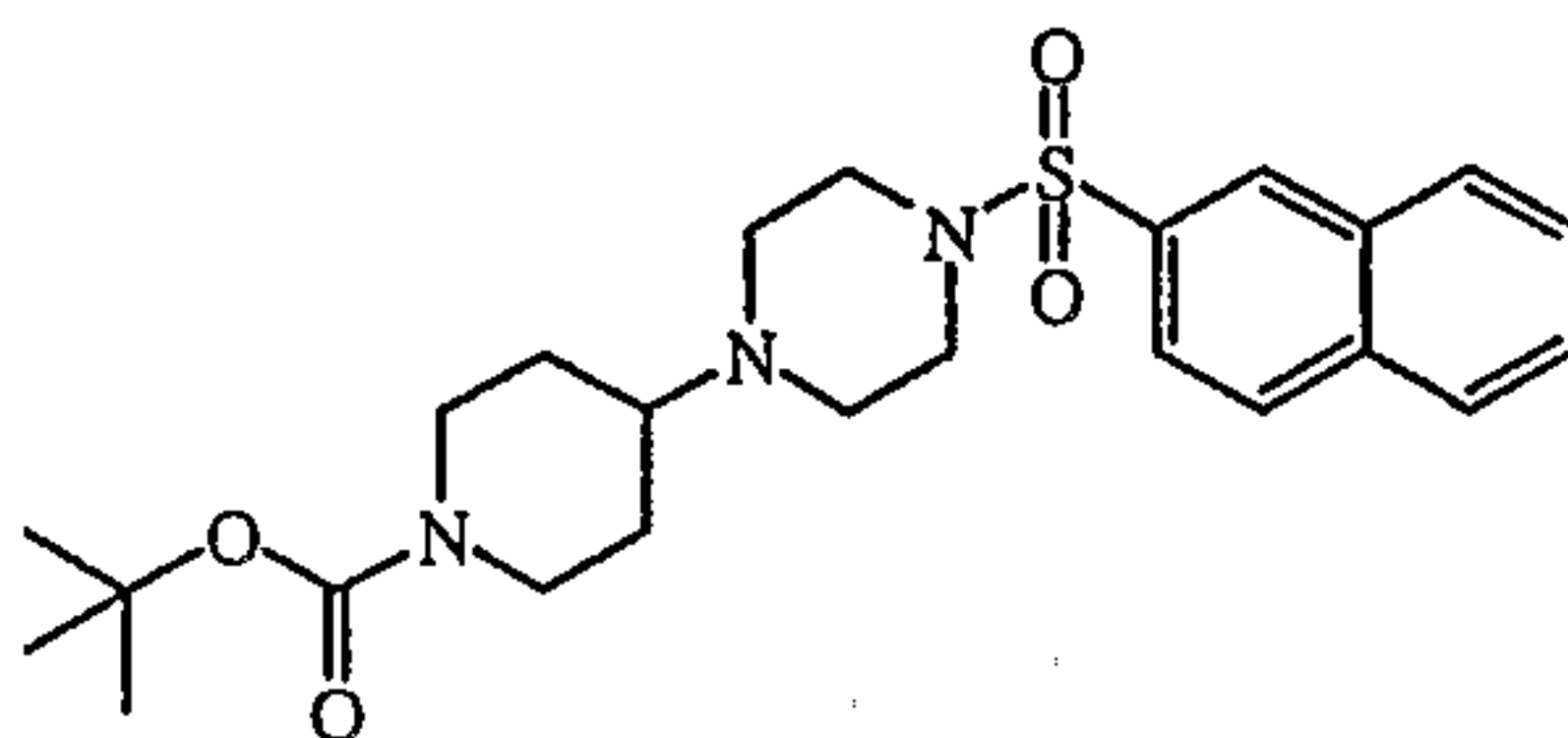
intermediate 14
