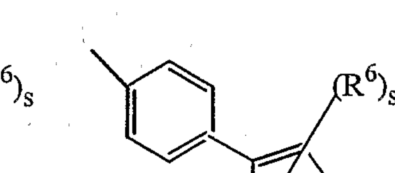
(a-19)
