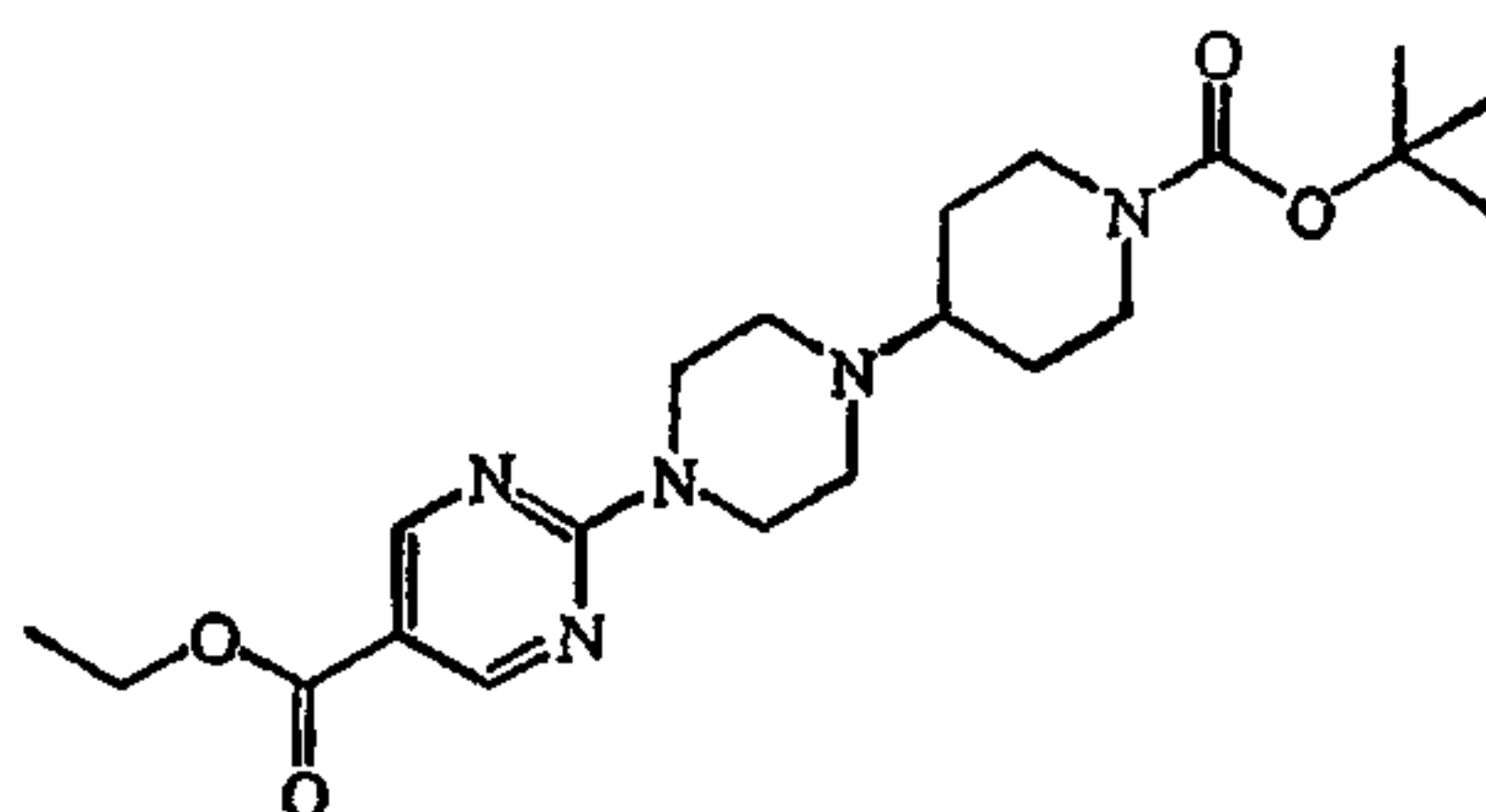
intermediate 11
