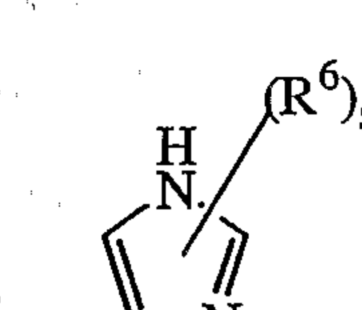
(a-14)
