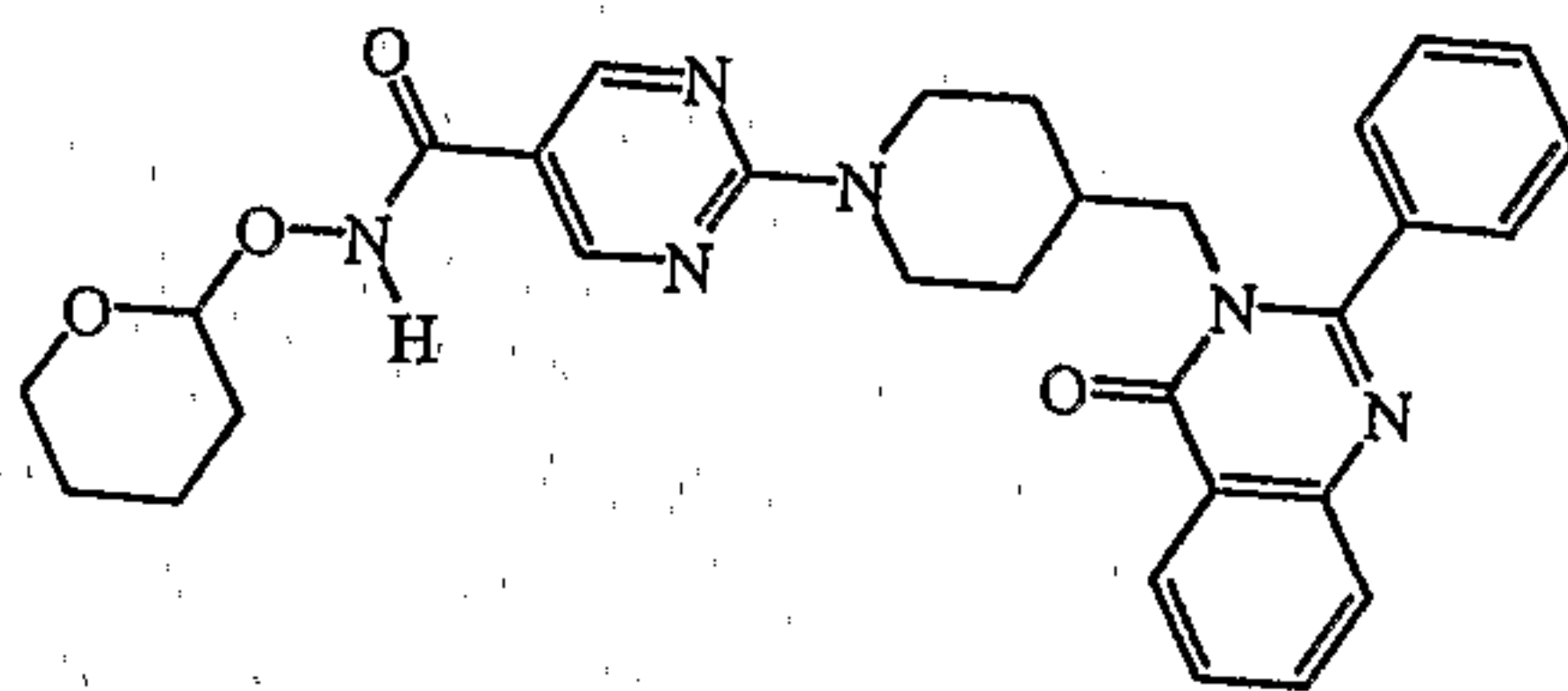
intermediate 23
