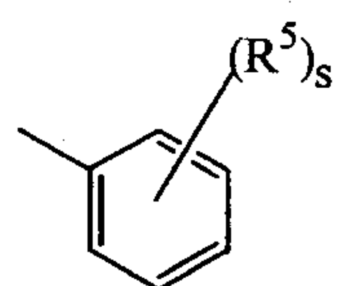
(a-1)
