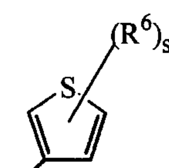
(a-10)
