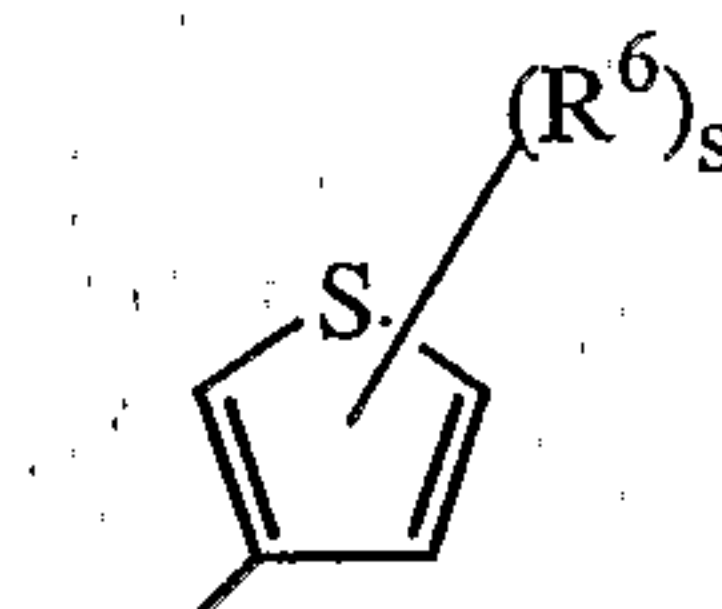
(a-10)
