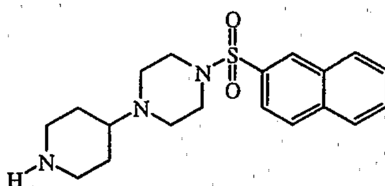
.HCl intermediate 15
