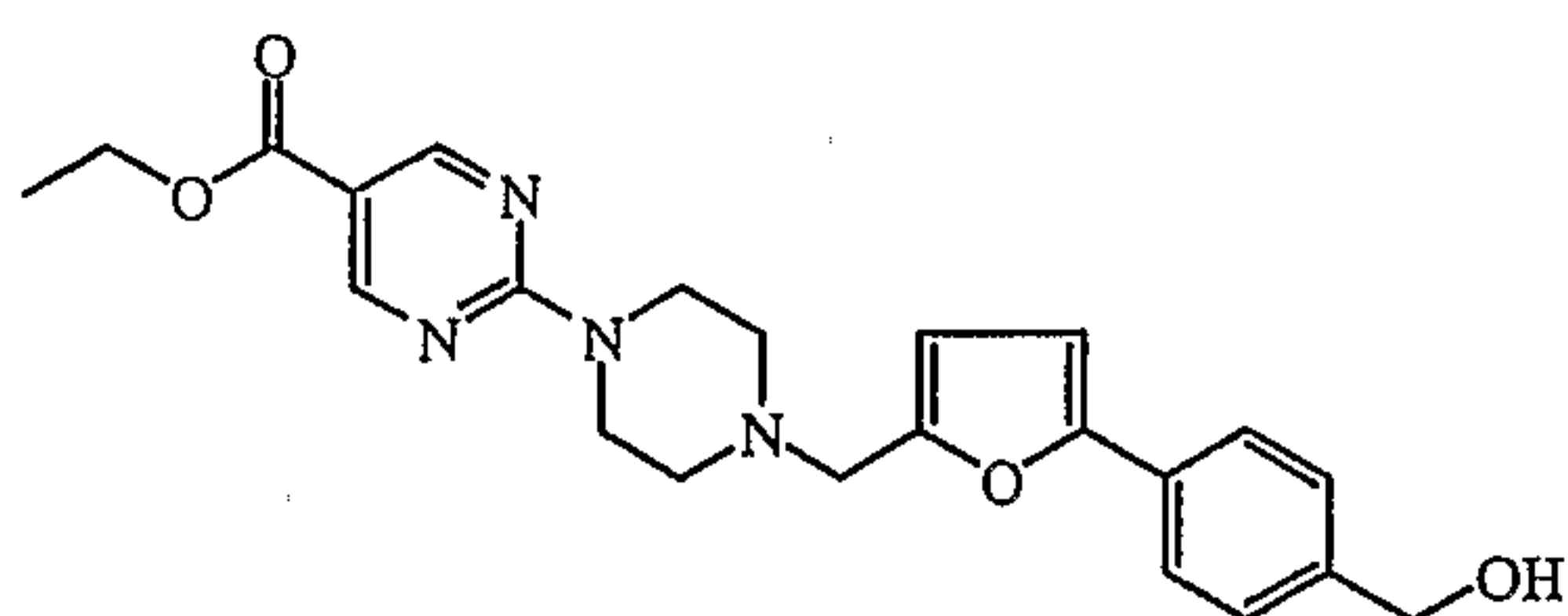
intermediate 27
