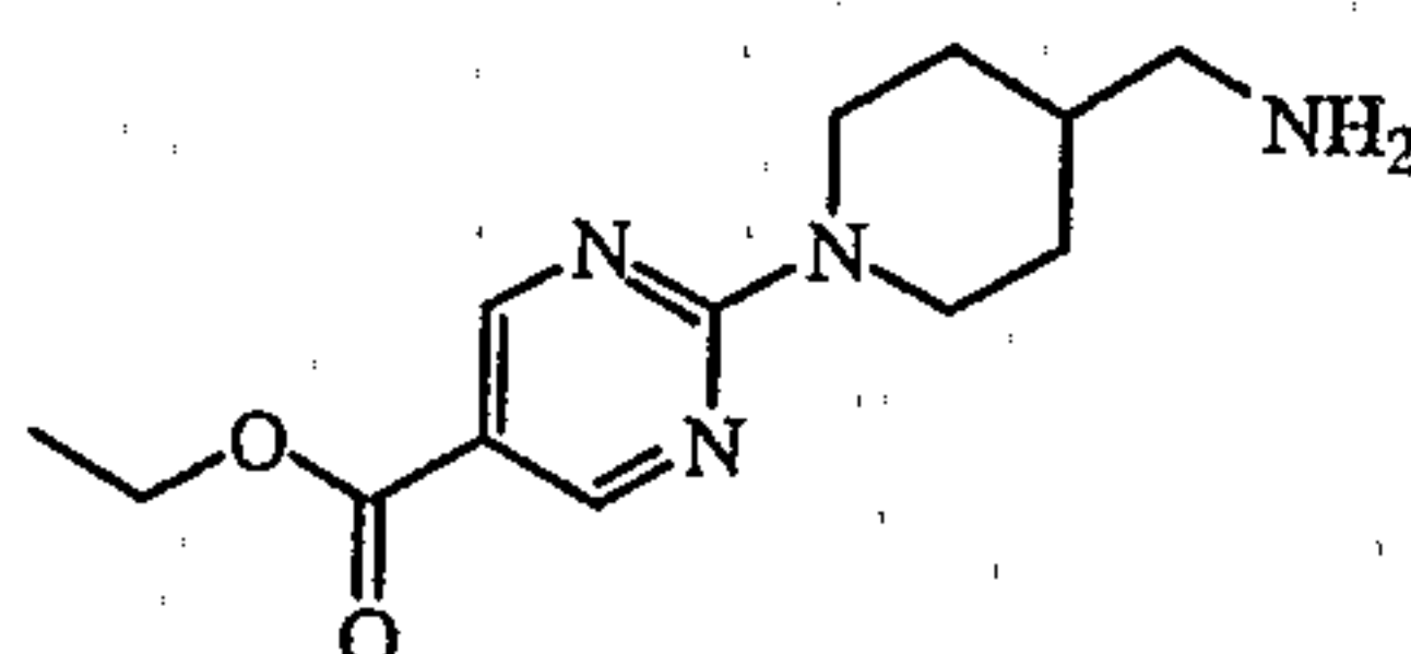
intermediate 17
