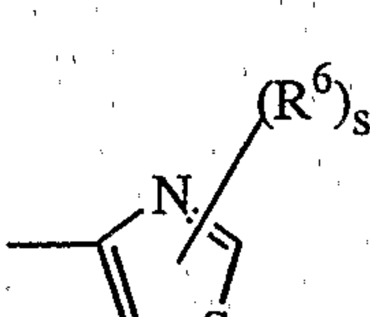
(a-15)
