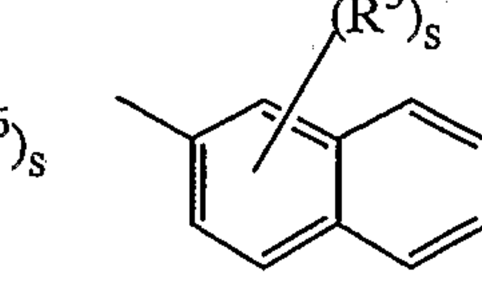
(a-20)
