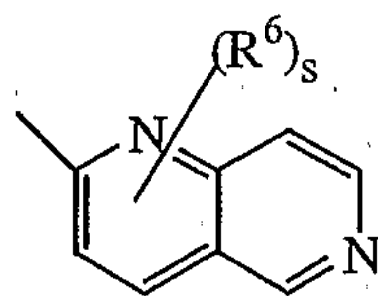
(a-25)
