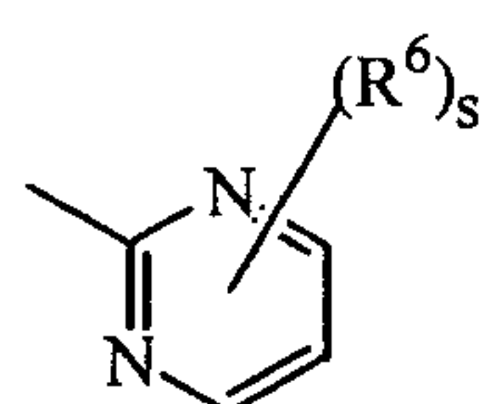
(a-5)
