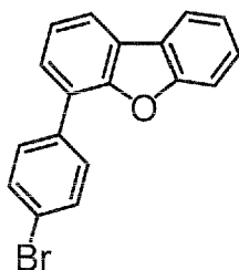
Intermediate 1-1
