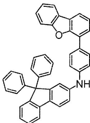
Intermediate 2-1
