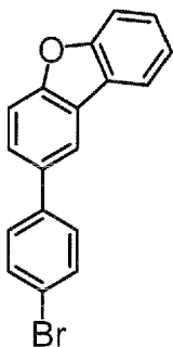
Intermediate 1-6
