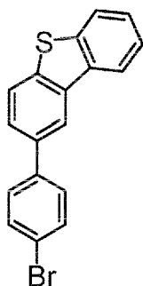
Intermediate 1-13
