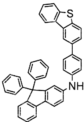
Intermediate 2-5
