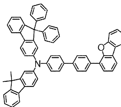
Comparative compound 2
