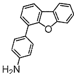
Intermediate 1-3
