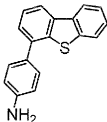
Intermediate 1-11
