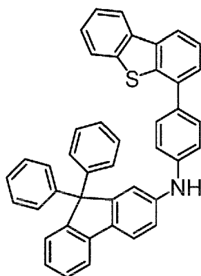
Intermediate 2-4
