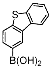
Intermediate 1-12
