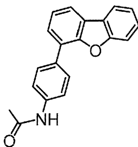
Intermediate 1-2
