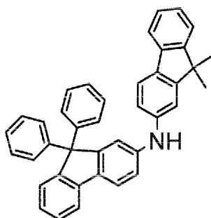
Intermediate 2-3
