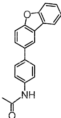
Intermediate 1-7
