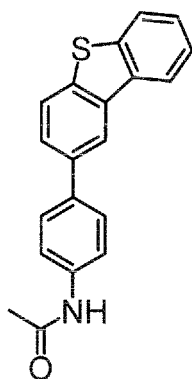
Intermediate 1-14
