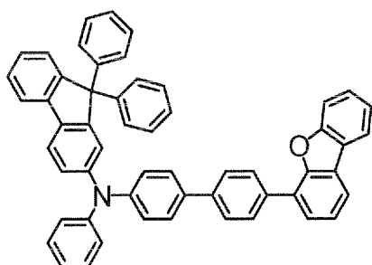
Comparative compound 1
