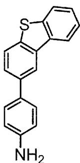
Intermediate 1-15
