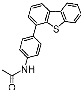
Intermediate 1-10
