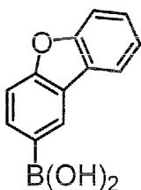
Intermediate 1-5
