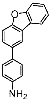
Intermediate 1-8
