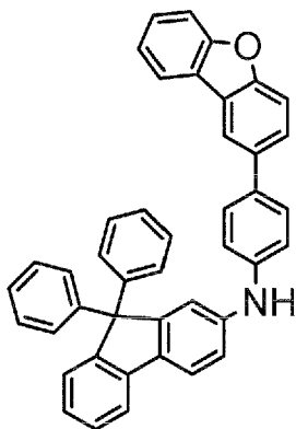
Intermediate 2-2
