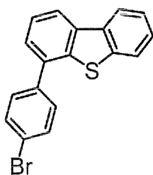
Intermediate 1-9
