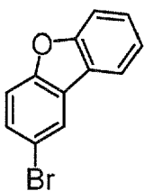
Intermediate 1-4
