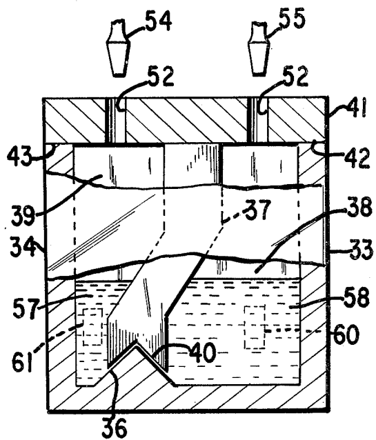
INTRODUCING LIQUID TO DISSOLVE REAGENTS
