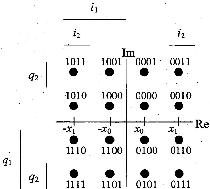
Mapping 1 (bit-mapping order: i_1q_1i_2q_2 )
