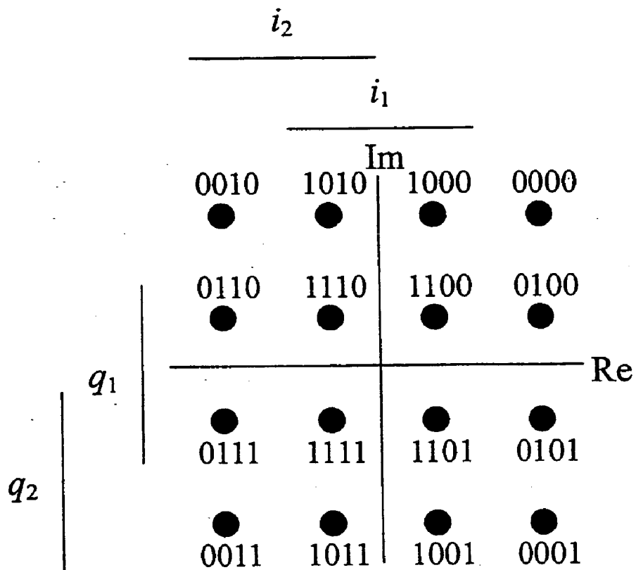
Mapping 2 (bit-mapping order: i_1q_1i_2q_2 )
