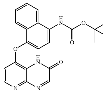
Tert-butyl 4-(2-oxo-1,2-dihydropyrido[2,3-b]pyrazin-8-yloxy)naphthalen-1-ylcarbamate
