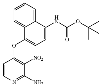
Tert-butyl 4-(2-amino-3-nitropyridin-4-yloxy)naphthalen-1-ylcarbamate
