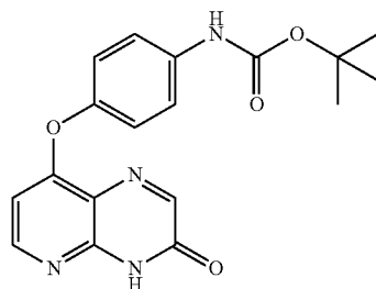
Tert-butyl 4-(3-oxo-3,4-dihydropyrido[2,3-b]pyrazin-8-yloxy)phenylcarbamate
