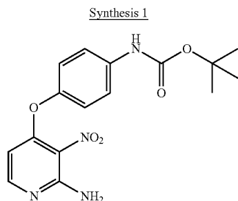
Tert-butyl 4-(2-amino-3-nitropyridin-4-yloxy)phenylcarbamate
