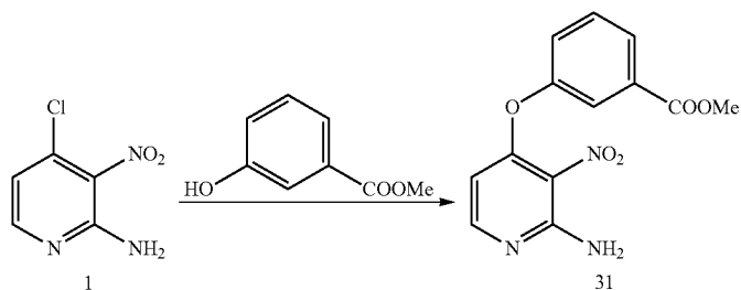
Scheme 10
