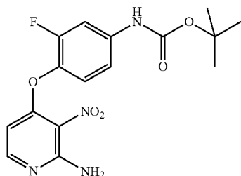
tert-butyl 4-(2-amino-3-nitropyridin-4-yloxy)-3-fluorophenylcarbamate
