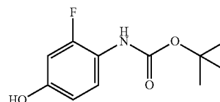
Tert-butyl 2-fluoro-4-hydroxyphenylcarbamate
