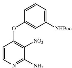
4-(3-N-(tert-Butoxycarbonyl)aminophenoxy)-3-nitro-2-amino-pyridine
