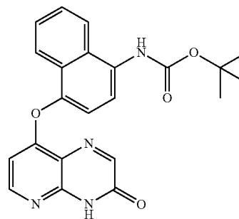
Tert-butyl 4-(2-oxo-1,2-dihydropyrido[2,3-b]pyrazin-8-yloxy)naphthalen-1-ylcarbamate
