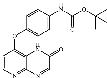
Tert-butyl 4-(2-oxo-1,2-dihydropyrido[2,3-b]pyrazin-8-yloxy)phenylcarbamate
