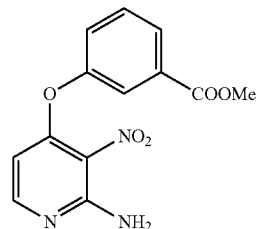
Methyl 3-(2-amino-3-nitropyridin-4-yloxy)benzoate
