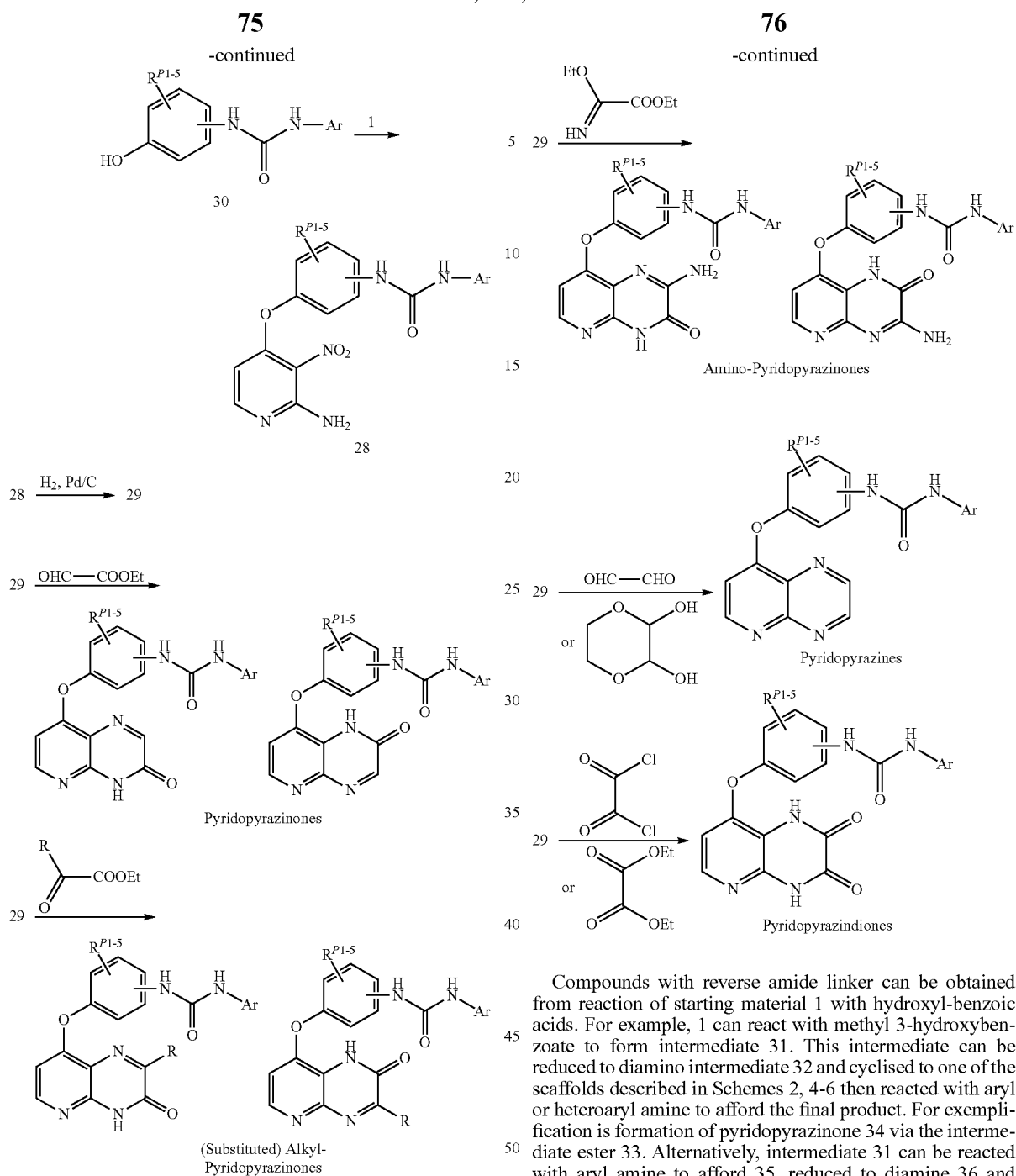
Scheme 10
