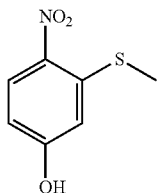
3-(methylthio)-4-nitrophenol
