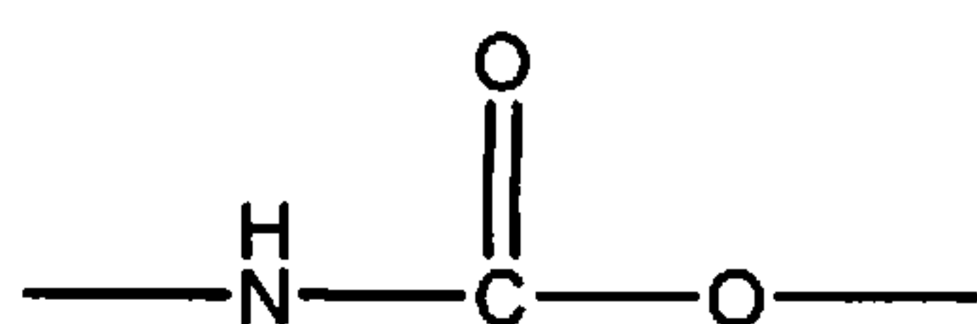
Carbamate.
