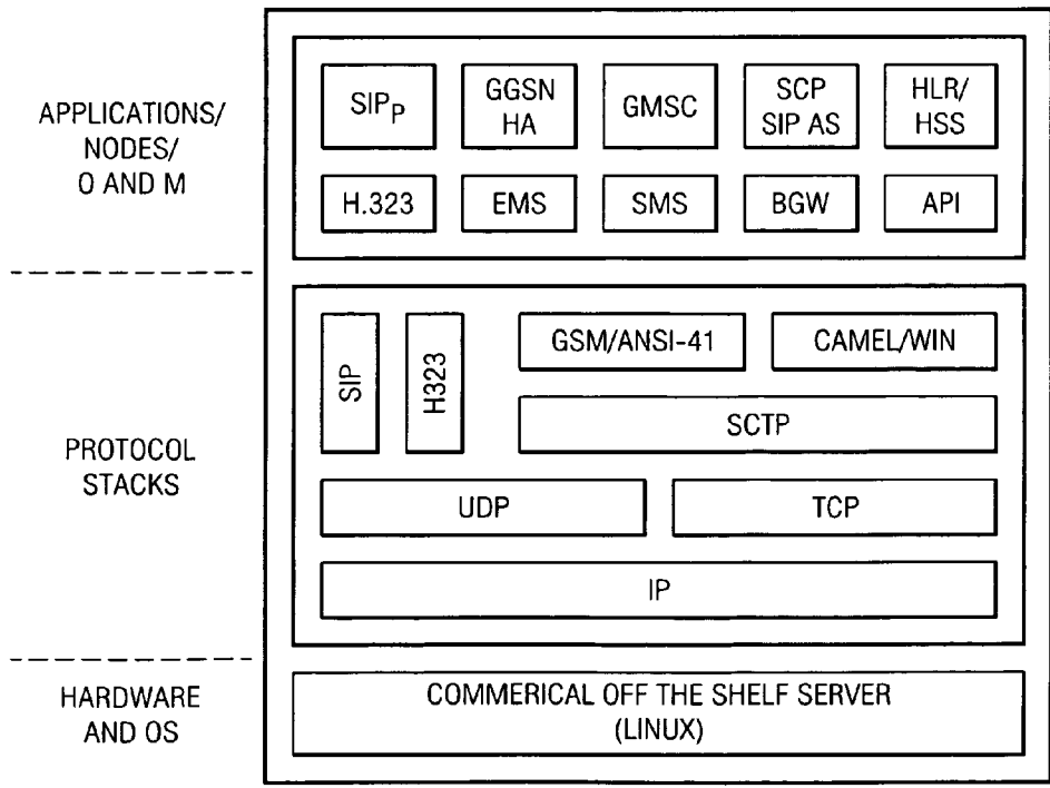
GATEWAY SERVER SYSTEM COMPONENTS
