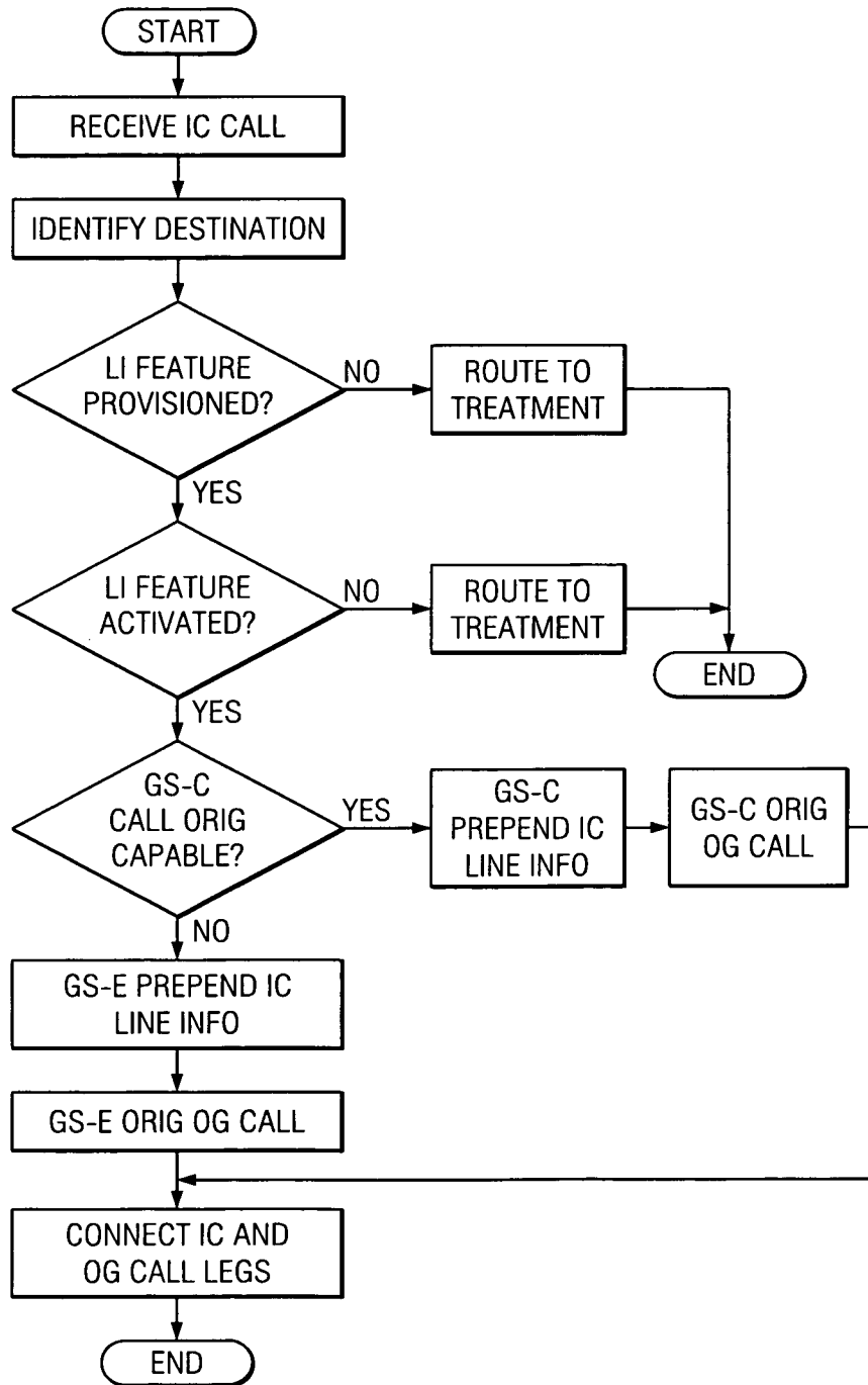
INCOMING CALL HANDLING FLOW CHART
