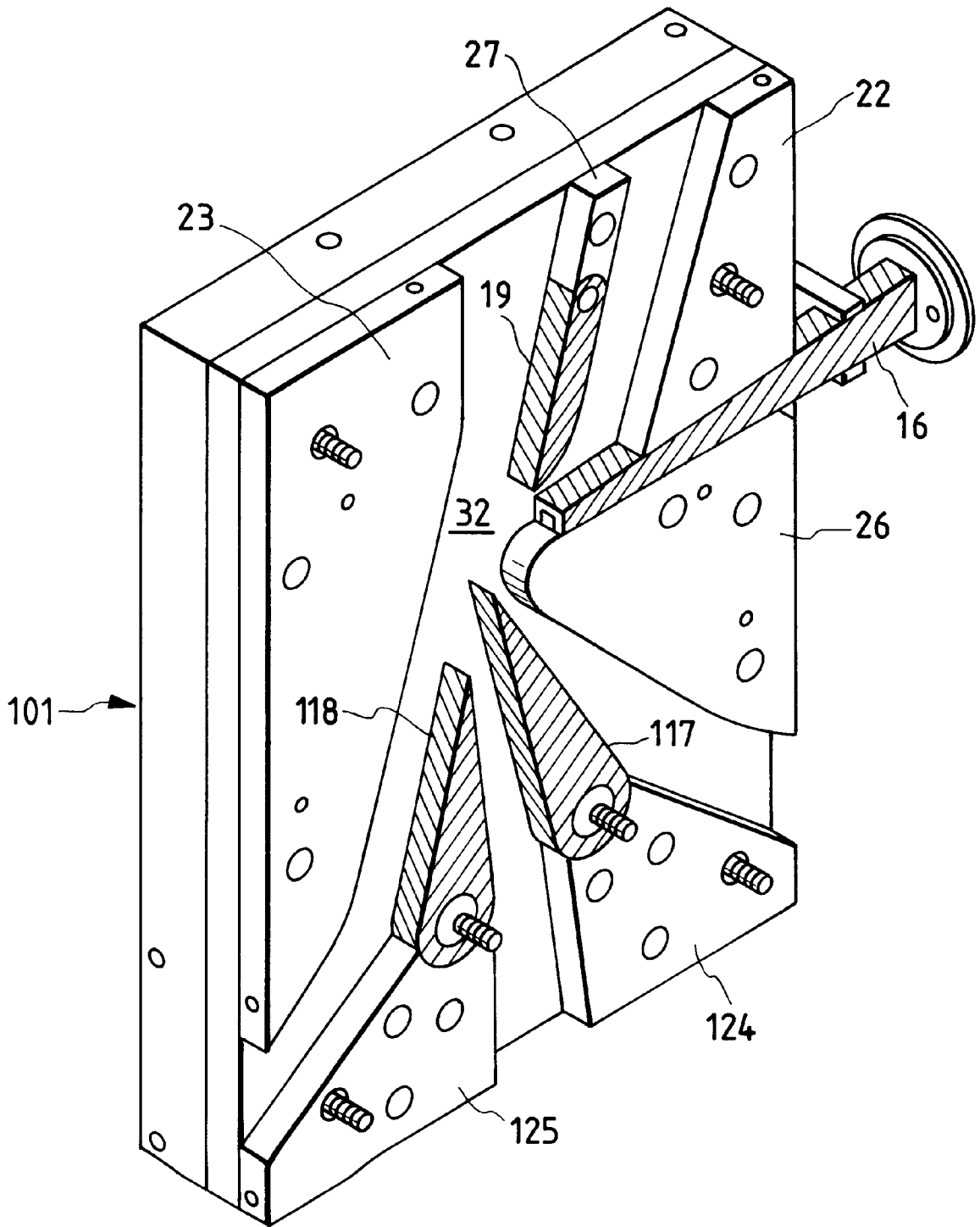
FIG. 16 PRIOR ART
