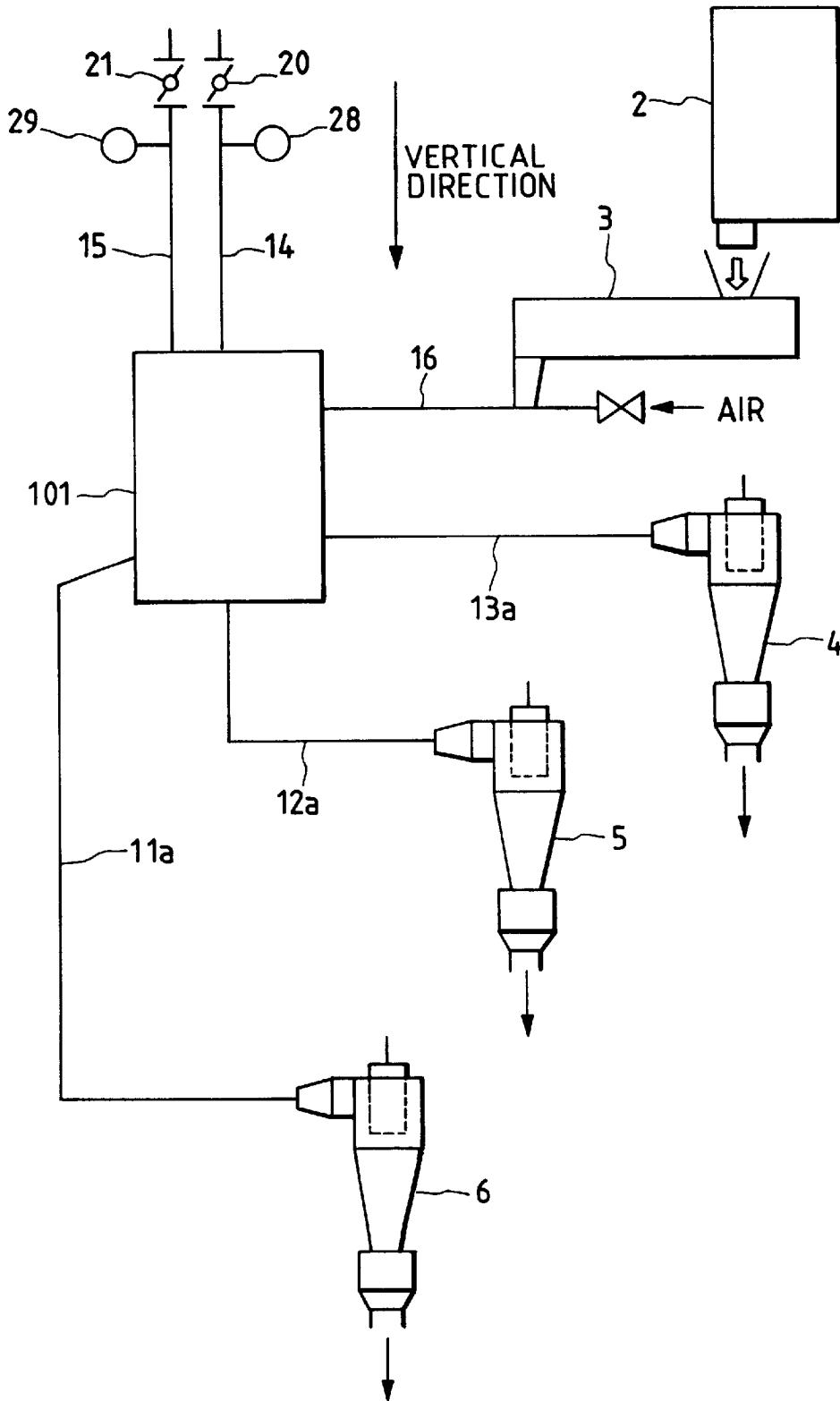
FIG. 18 PRIOR ART
