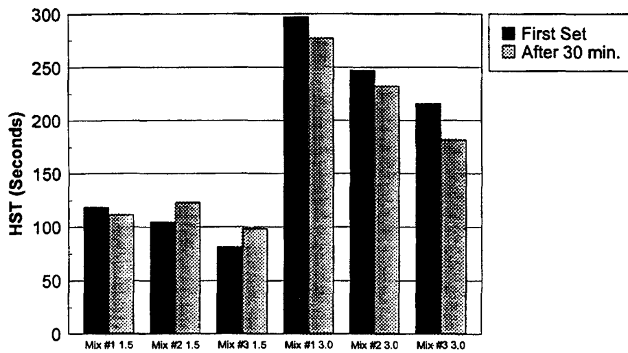
Figure 1: Results from Hercules Size Test (HST) performed on handsheets.
