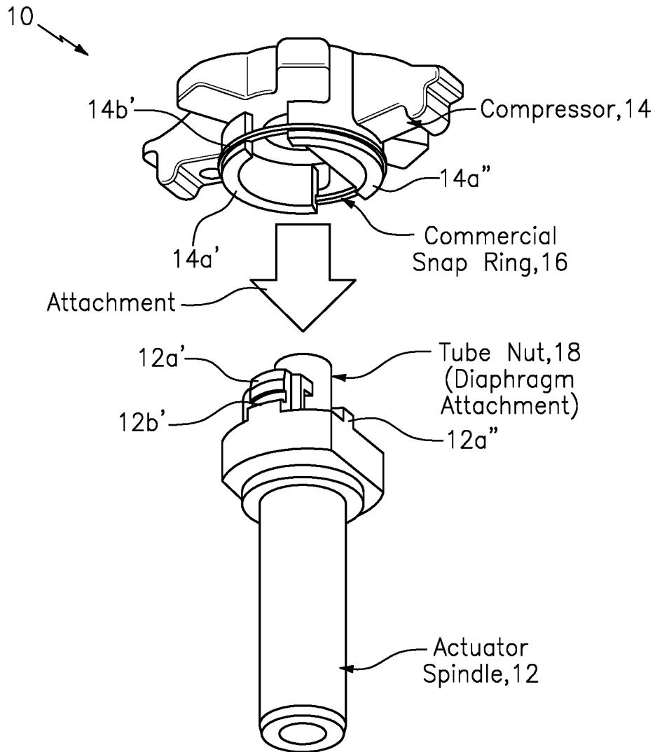
FIG. 4a: Attachment of Compressor to Actuator Spindle
