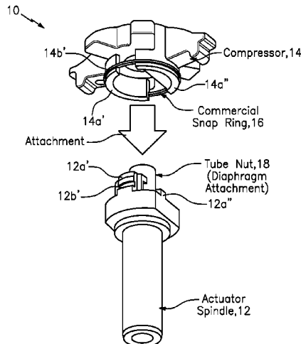
Attachment of Compressor to Actuator Spindle
