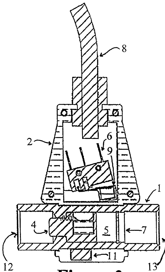
Figure 3 SECTION D-D
