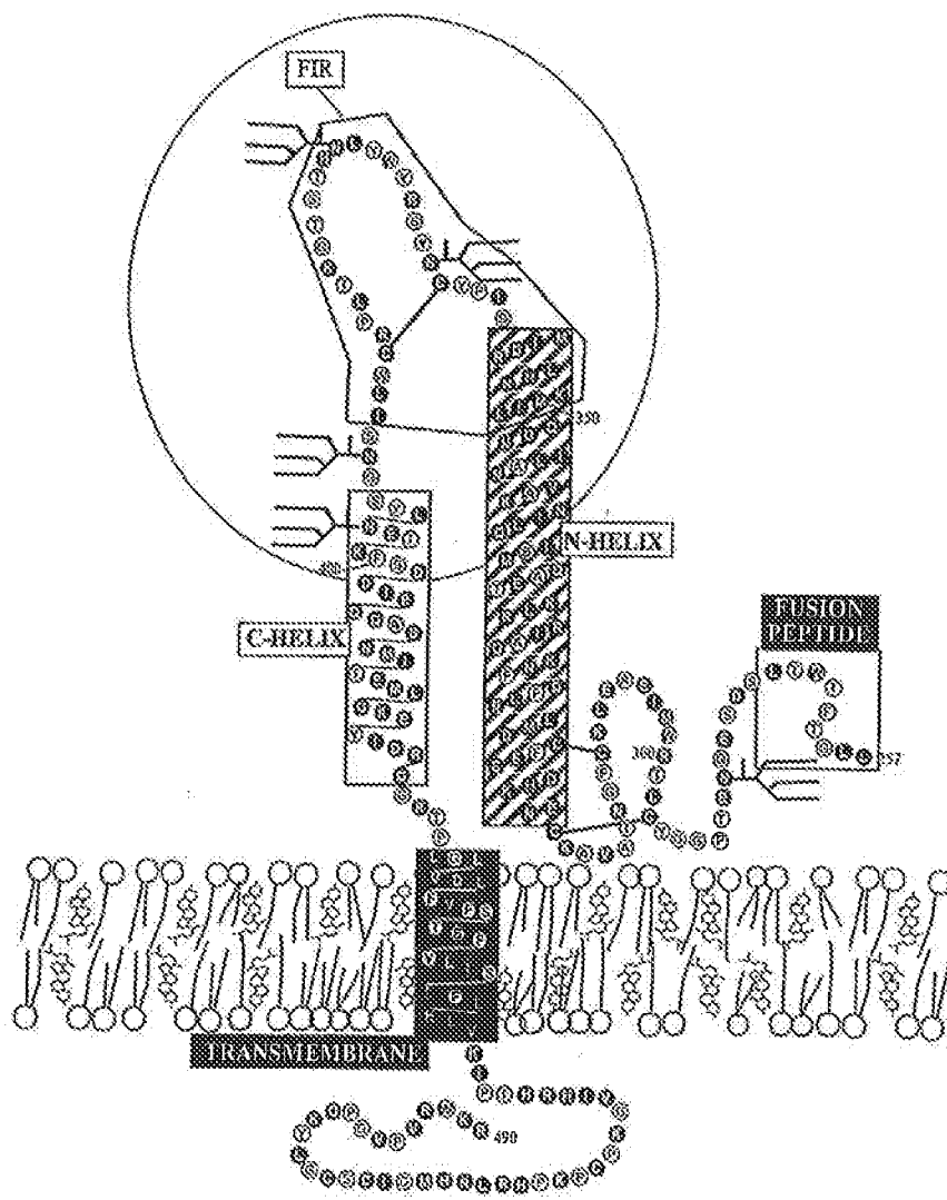
Lassa virus GP2 Figure 2
