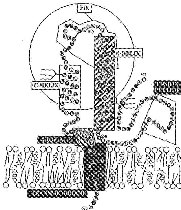
Ebola virus GP2 Figure 4
