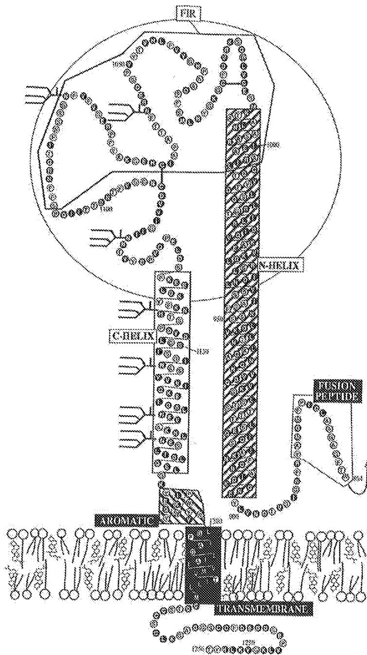
SARS CoV S Figure 3
