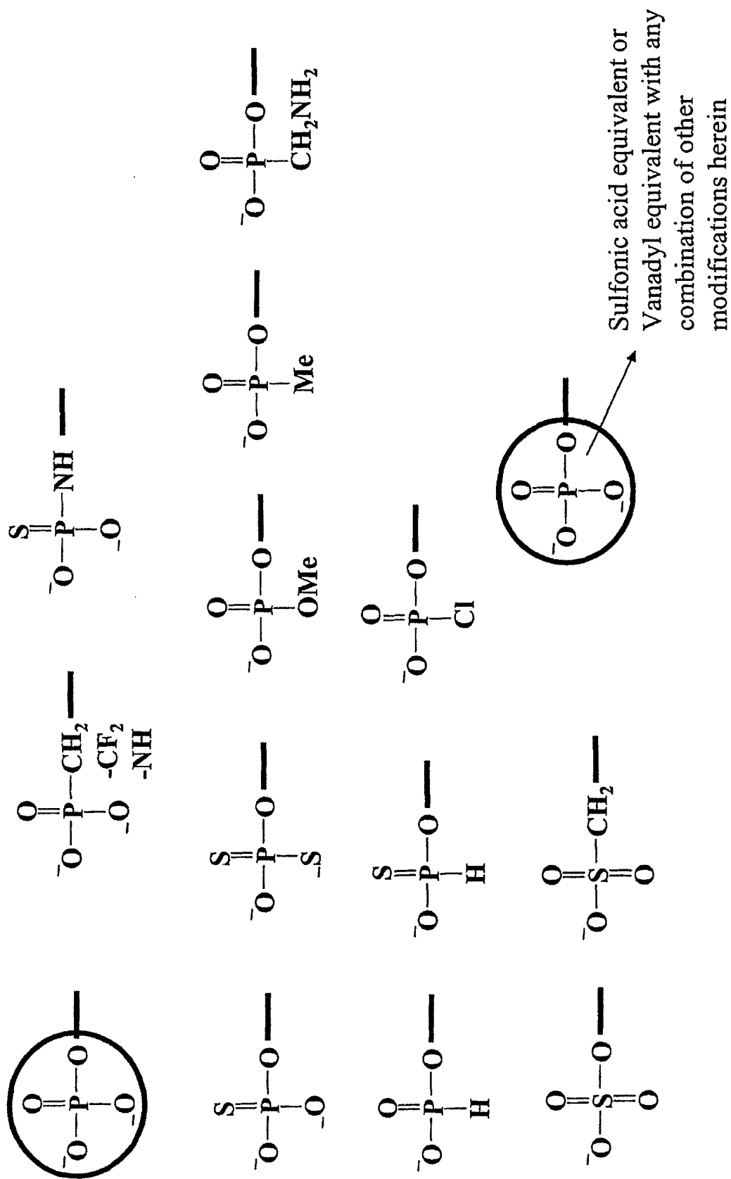
Figure 13: 5'-phosphate modifications
