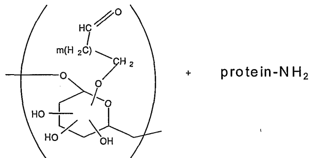
dextran aldehyde portion of polysaccharide above
