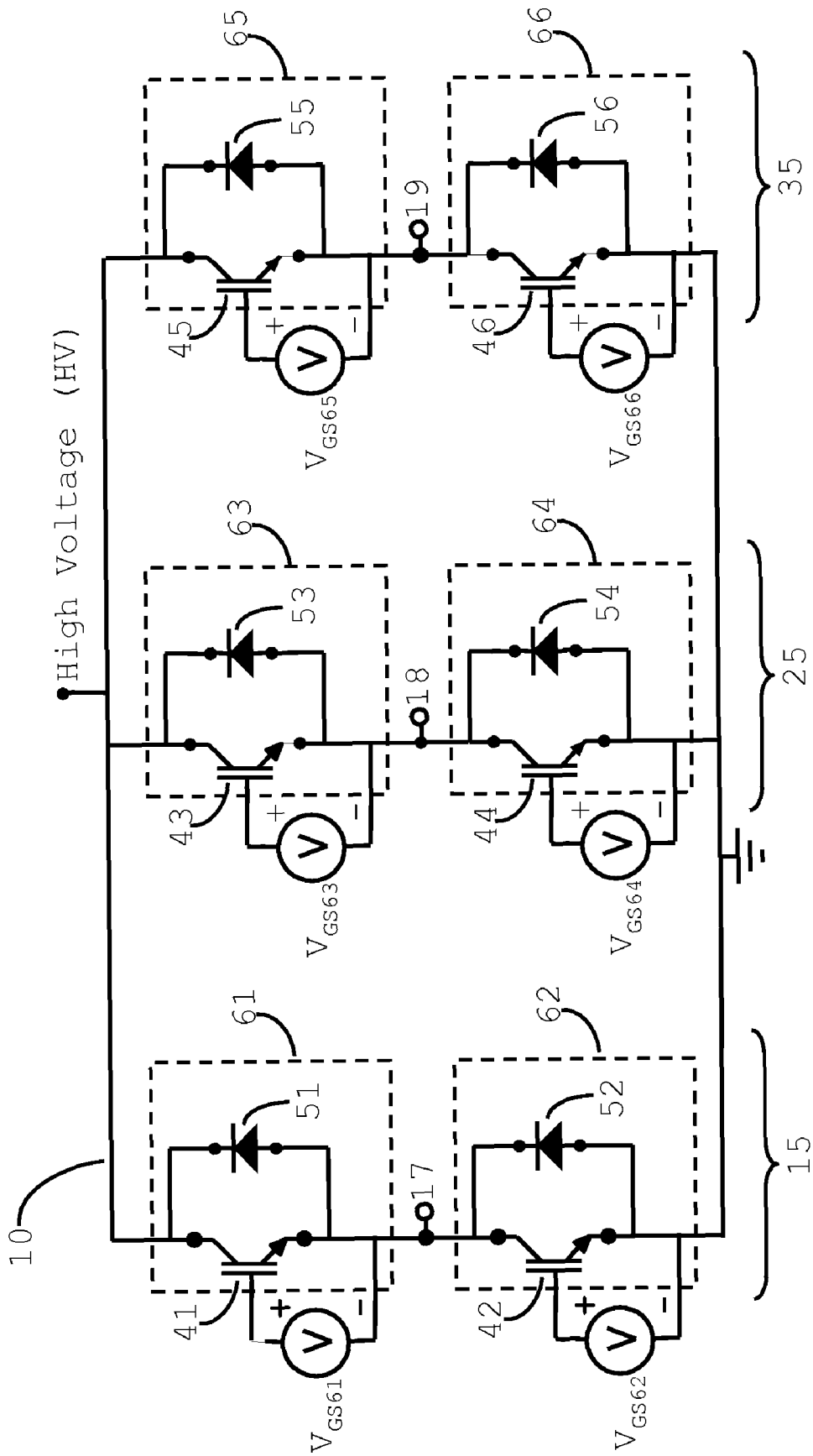
Figure 1 (prior art)
