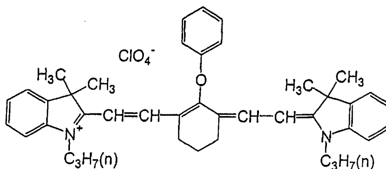
IR-768 perchlorate
