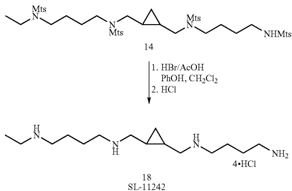
SL-11242 tetrahydrochloride 18
