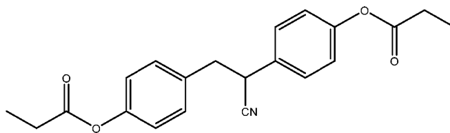
Compound 2
