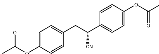
Compound 1
