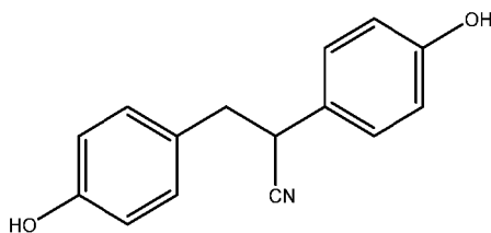
DPN (2,3-bis(4-hydroxyphenyl)propanenitrile)
