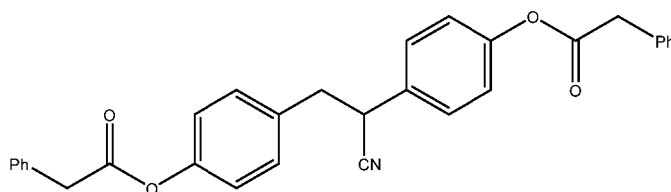
Compound 6
