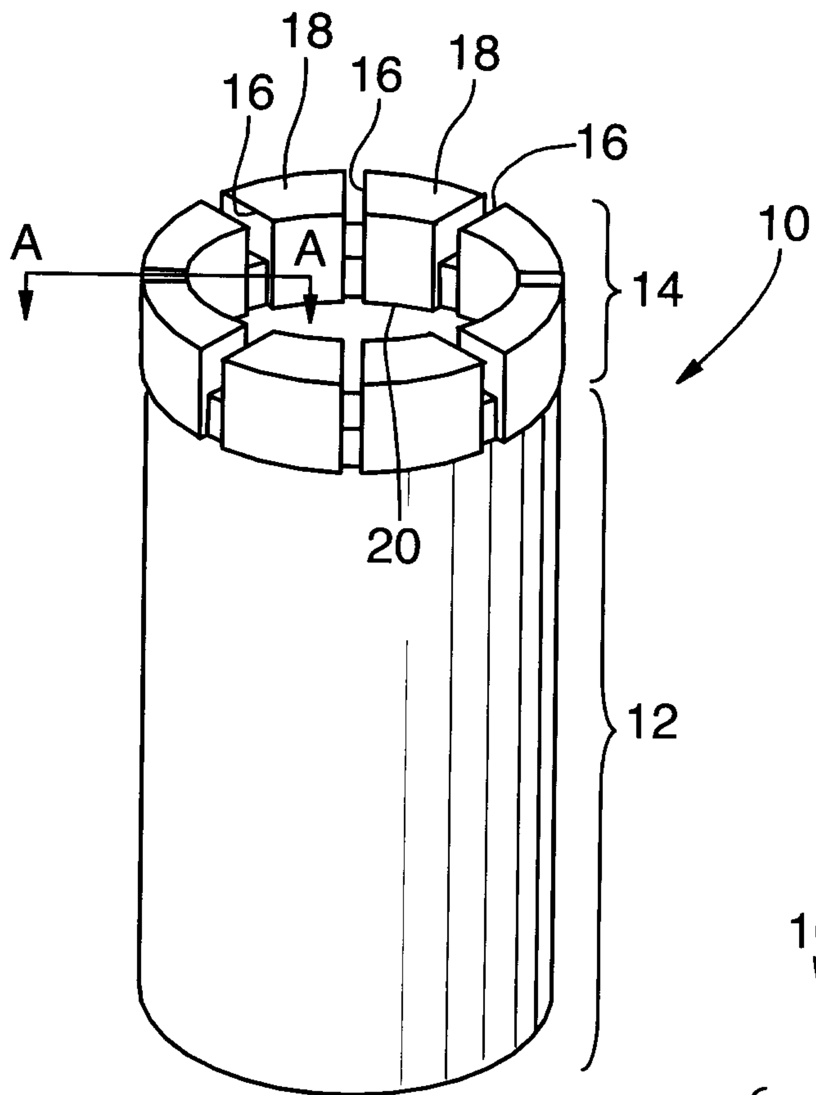
FIG. 1 (PRIOR ART)
