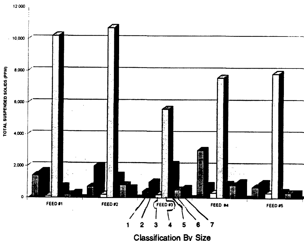
PARTICLE SIZE DISTRIBUTION OF SOME REPRESENTATIVE SPENT PARTS WASHER SOLVENT
