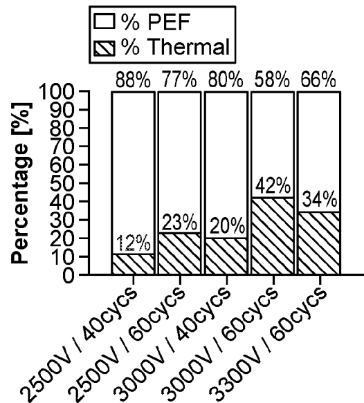
Lab 95 - Summary Volume Analysis xxxxV / 400kHz / xx cyces / 100pkts 500-1000µs cyc delay / 3s pkt delay
