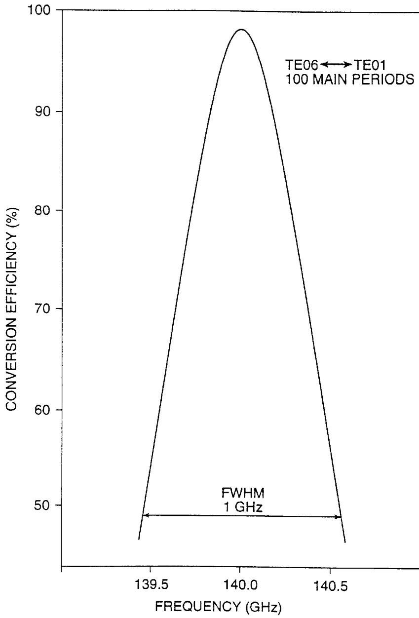
FIG. 24 PRIOR ART
