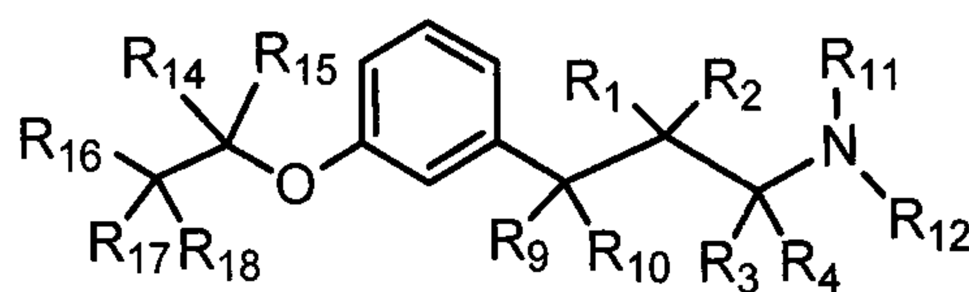
Formula (IIa)
