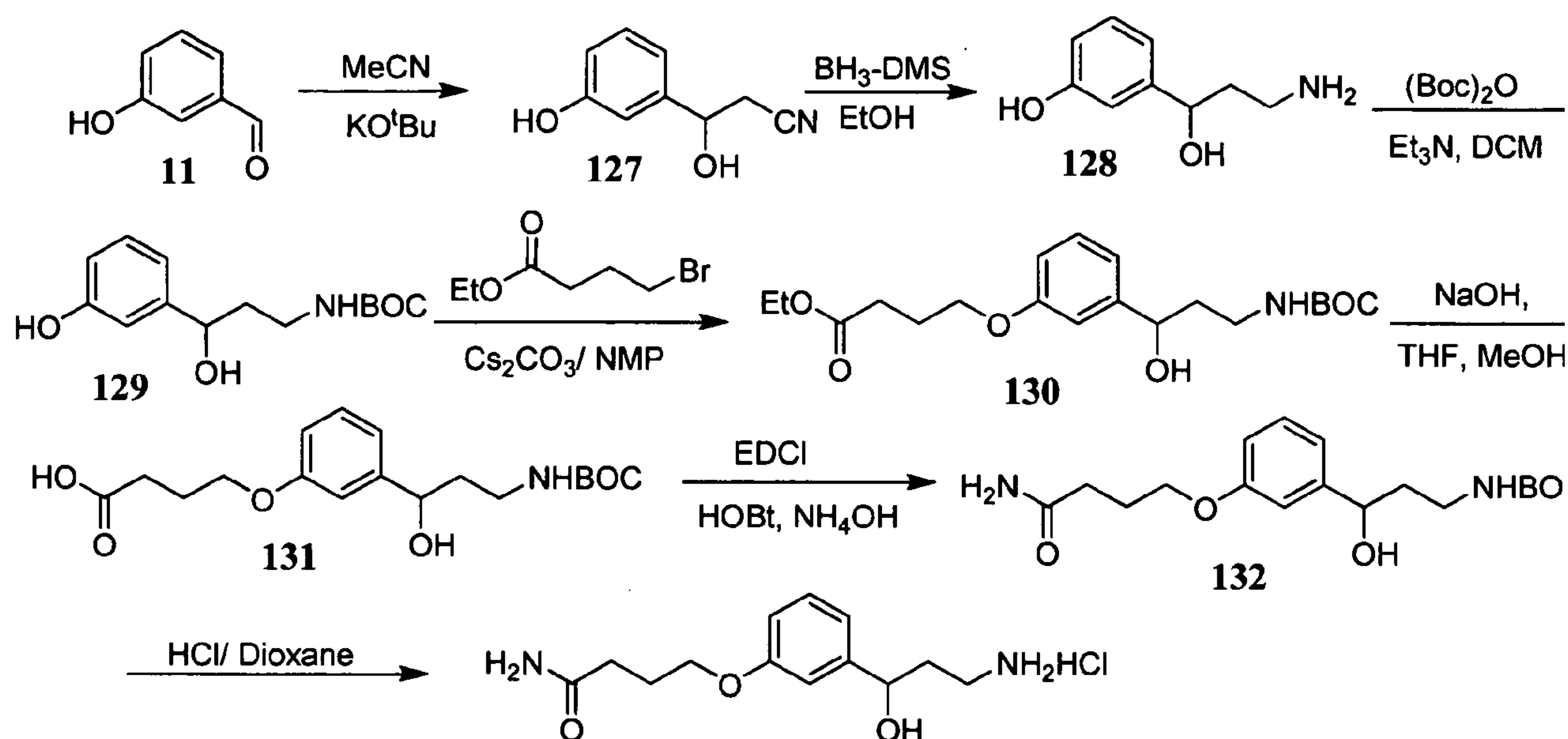
SCHEME 42
