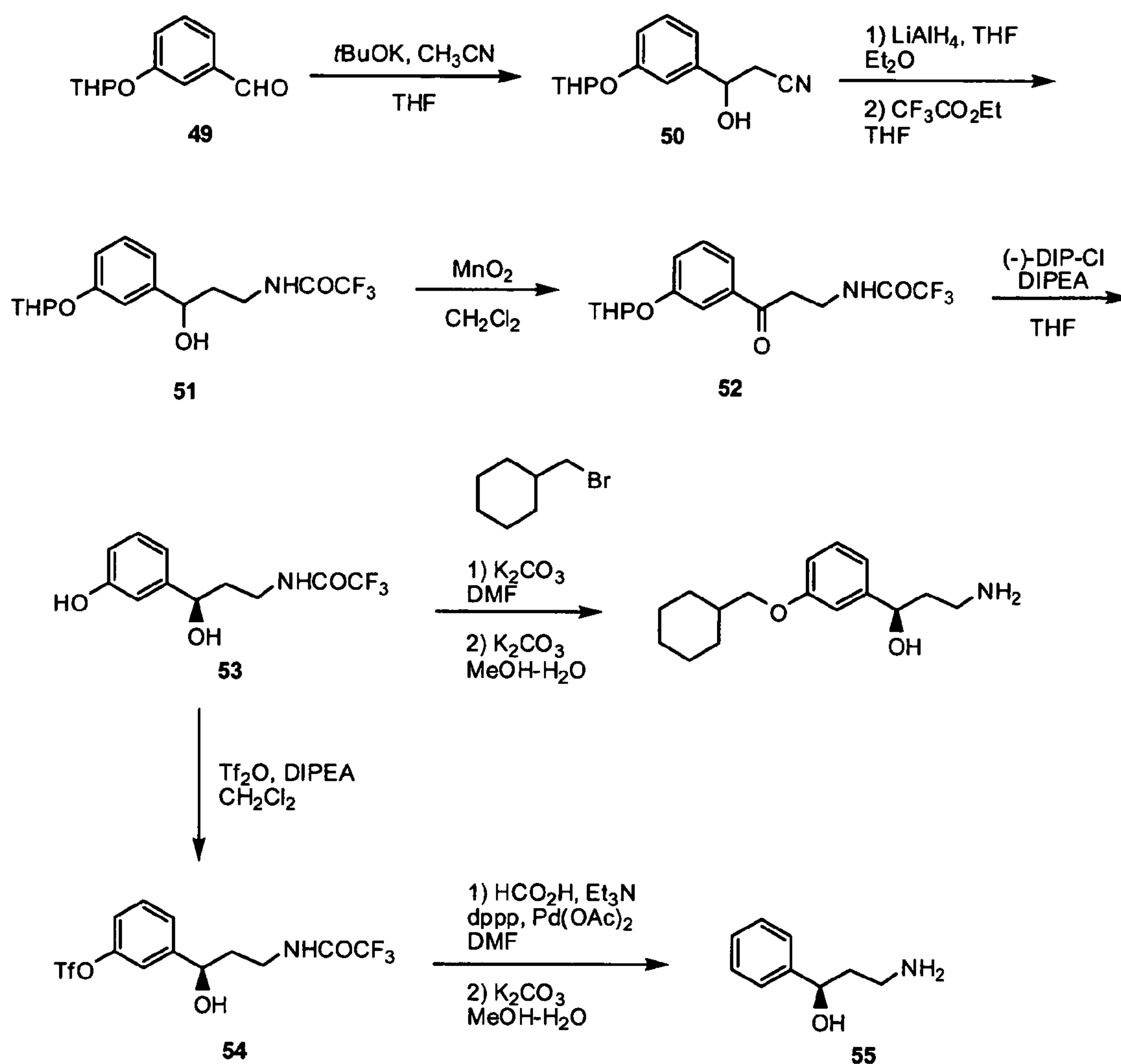
SCHEME 15
