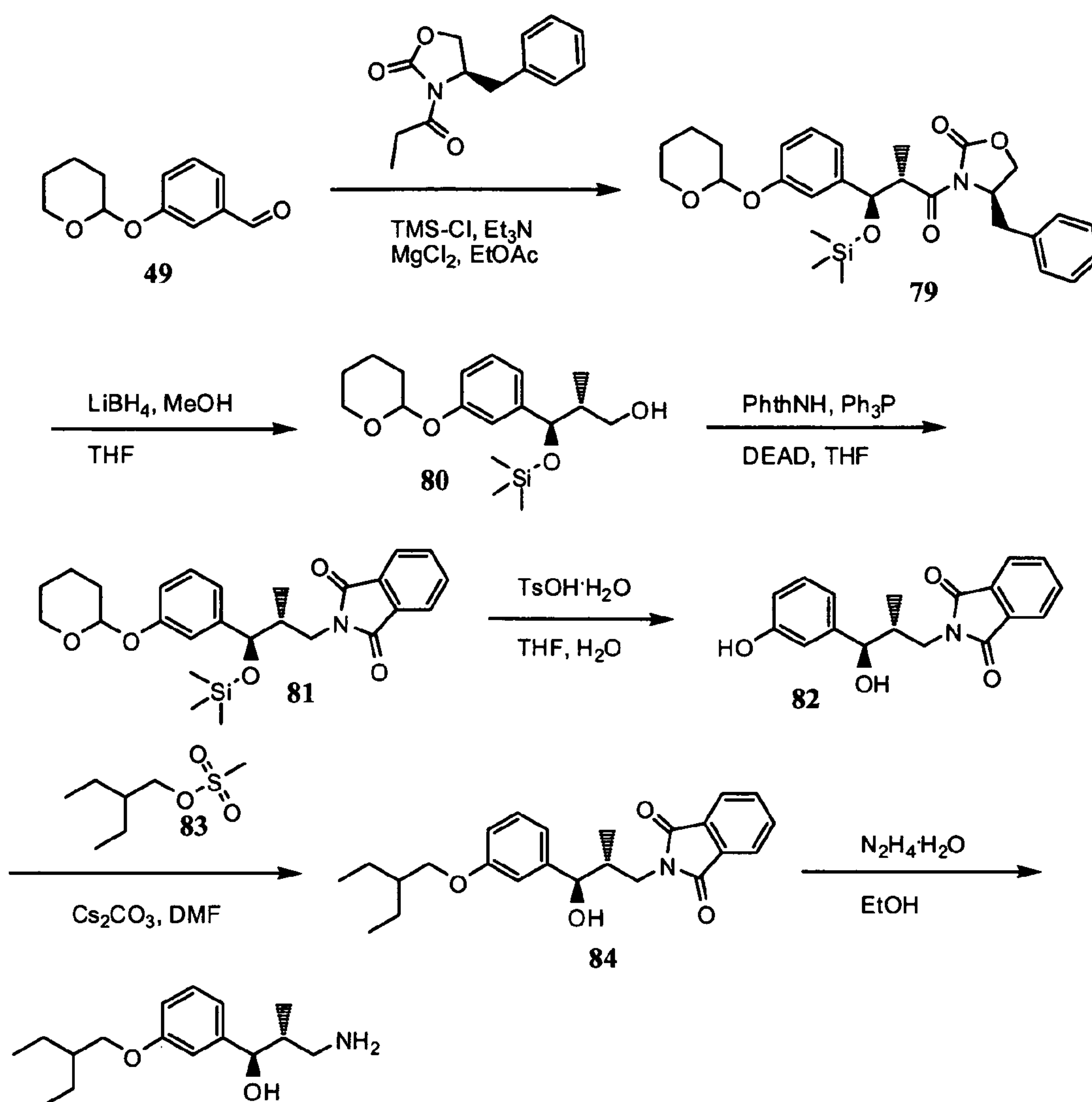
SCHEME 23
