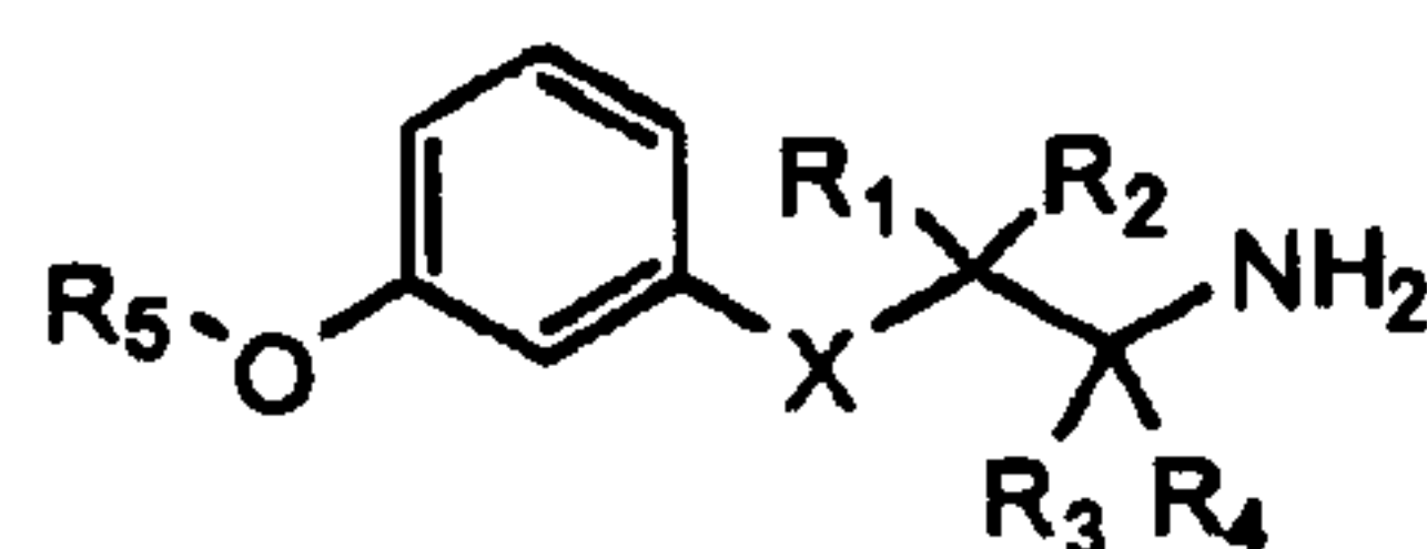
Formula (I)
