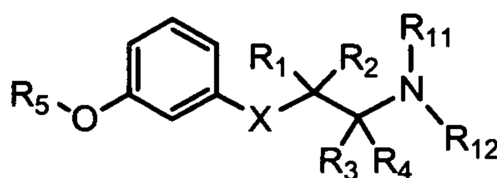
Formula (I)
