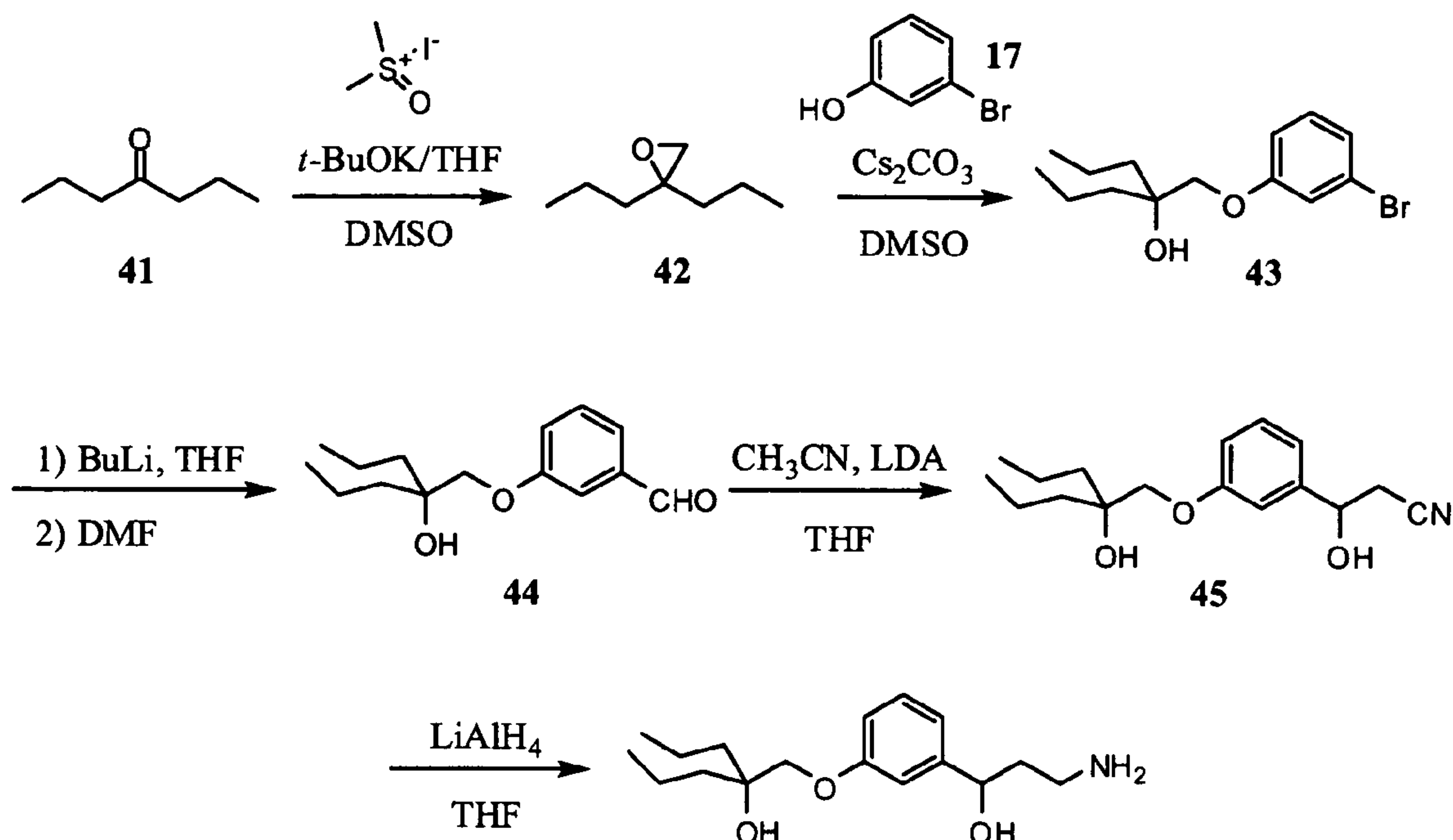
SCHEME 12
