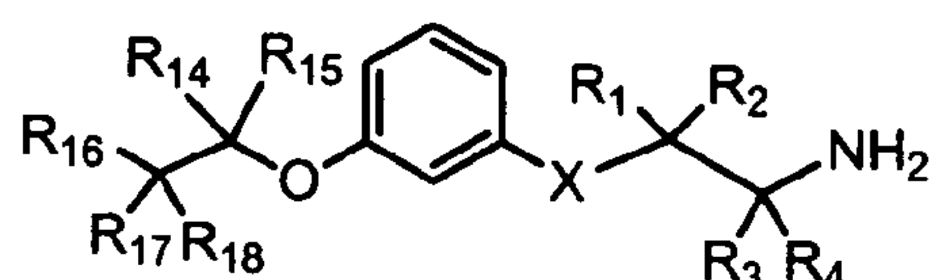
Formula (II)
