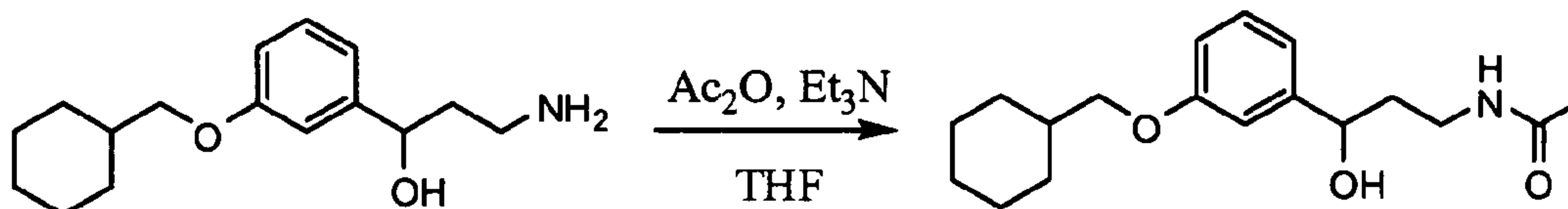
SCHEME 11
