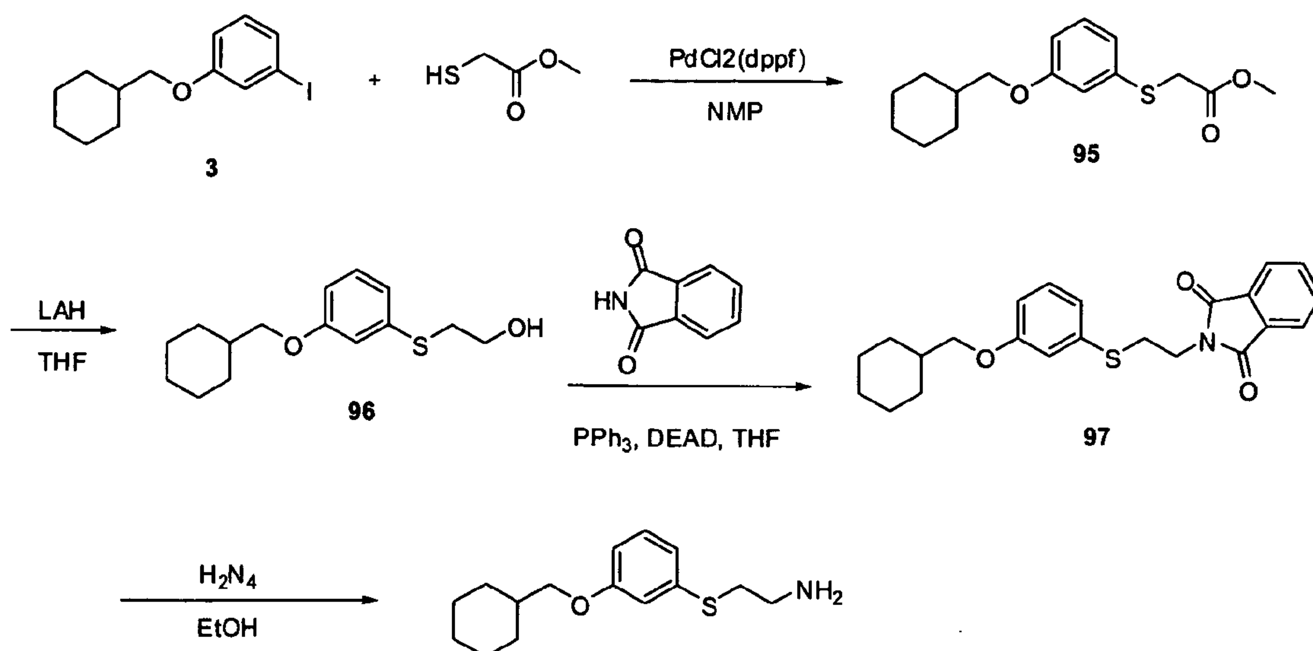
SCHEME 31
