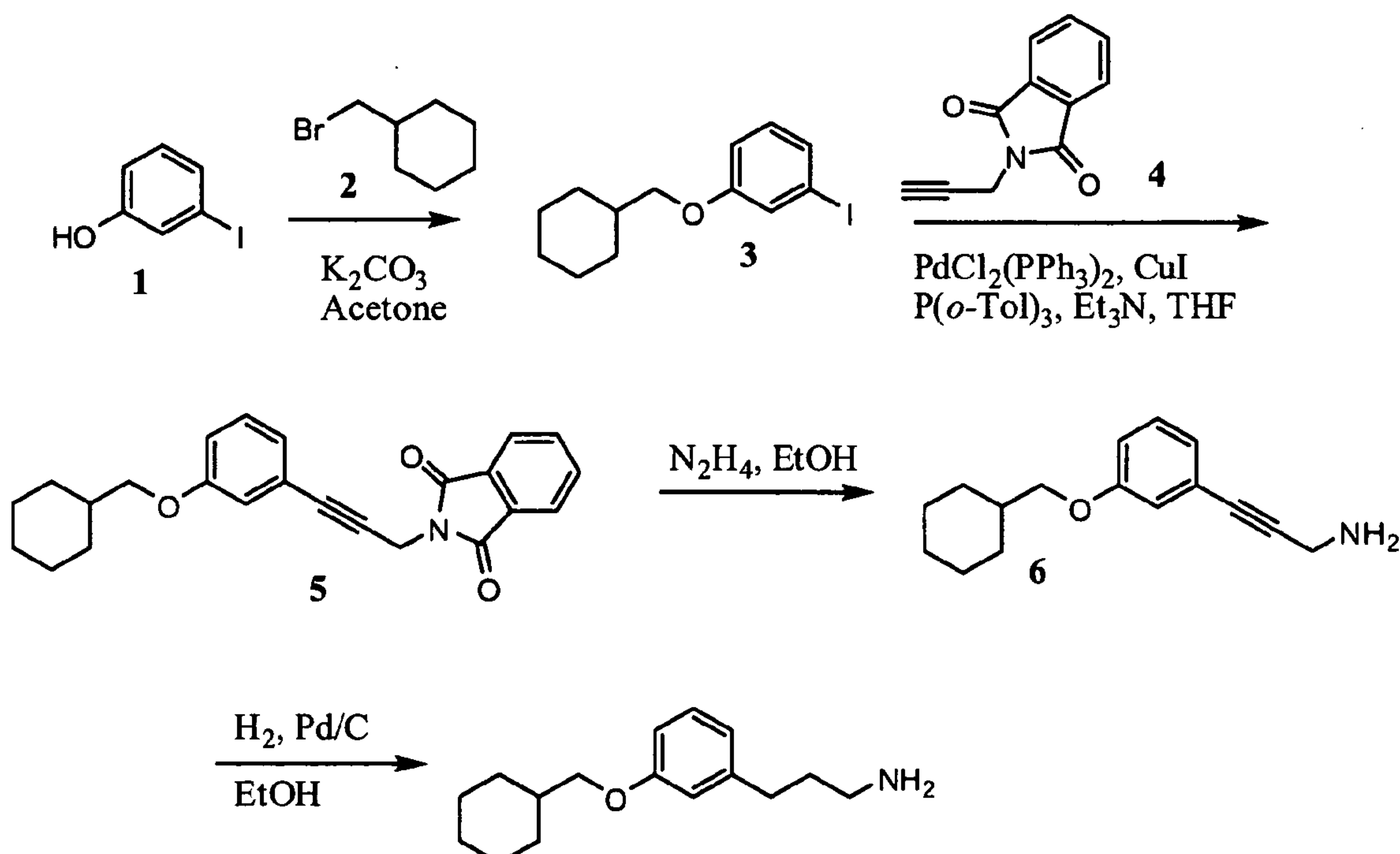
SCHEME 1
