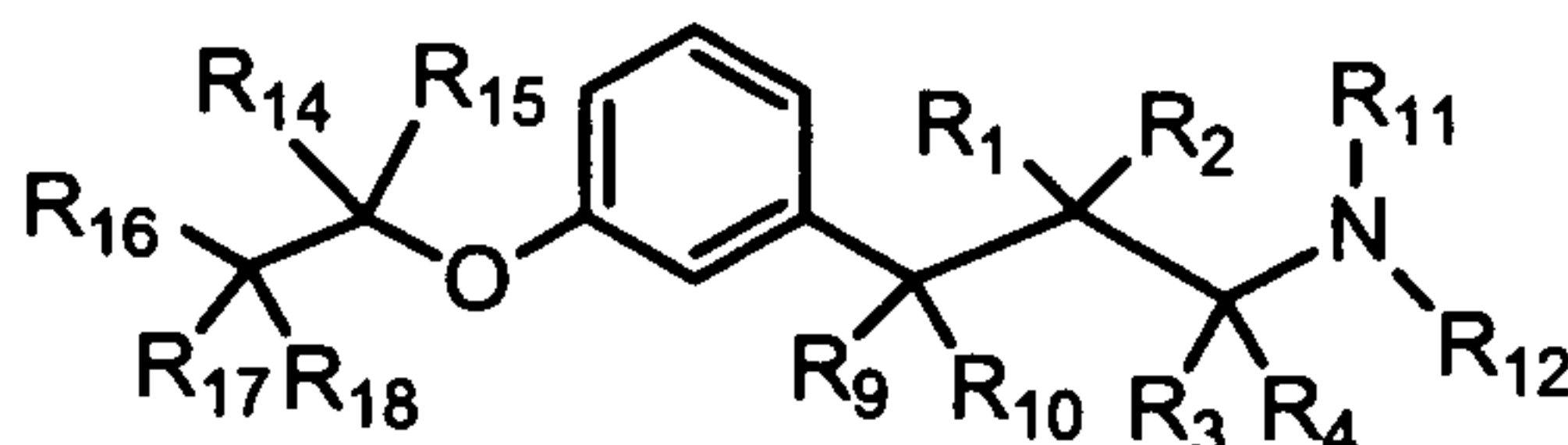
Formula (IIa)
