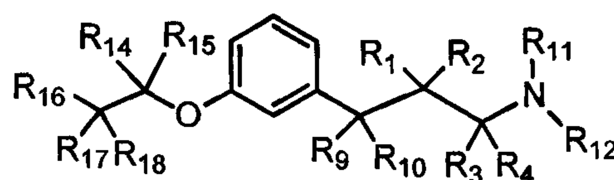
Formula (IIa)
