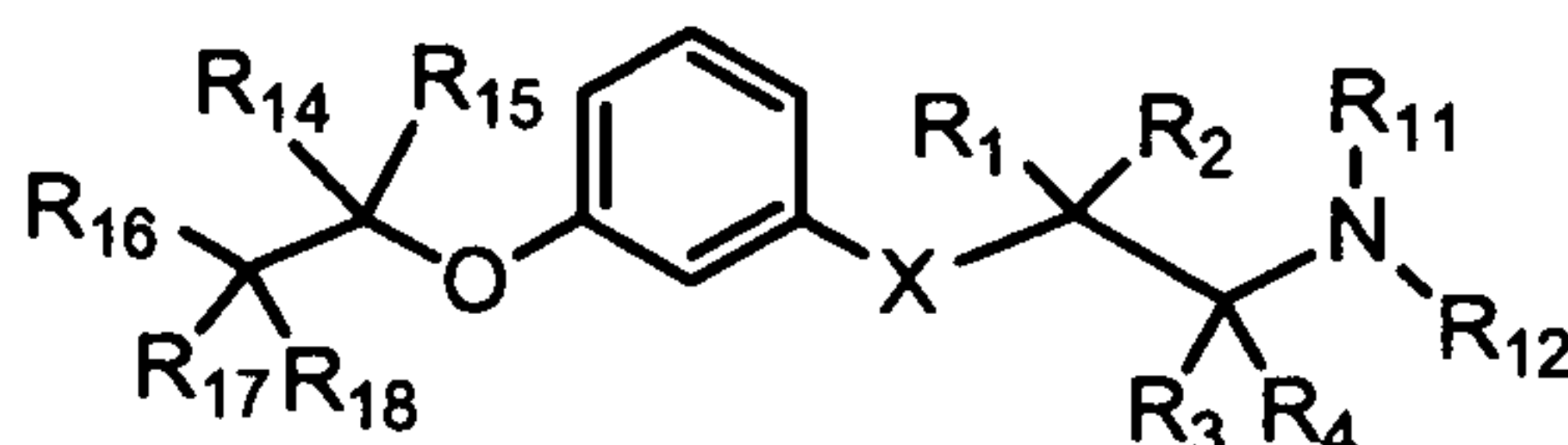
Formula (II)
