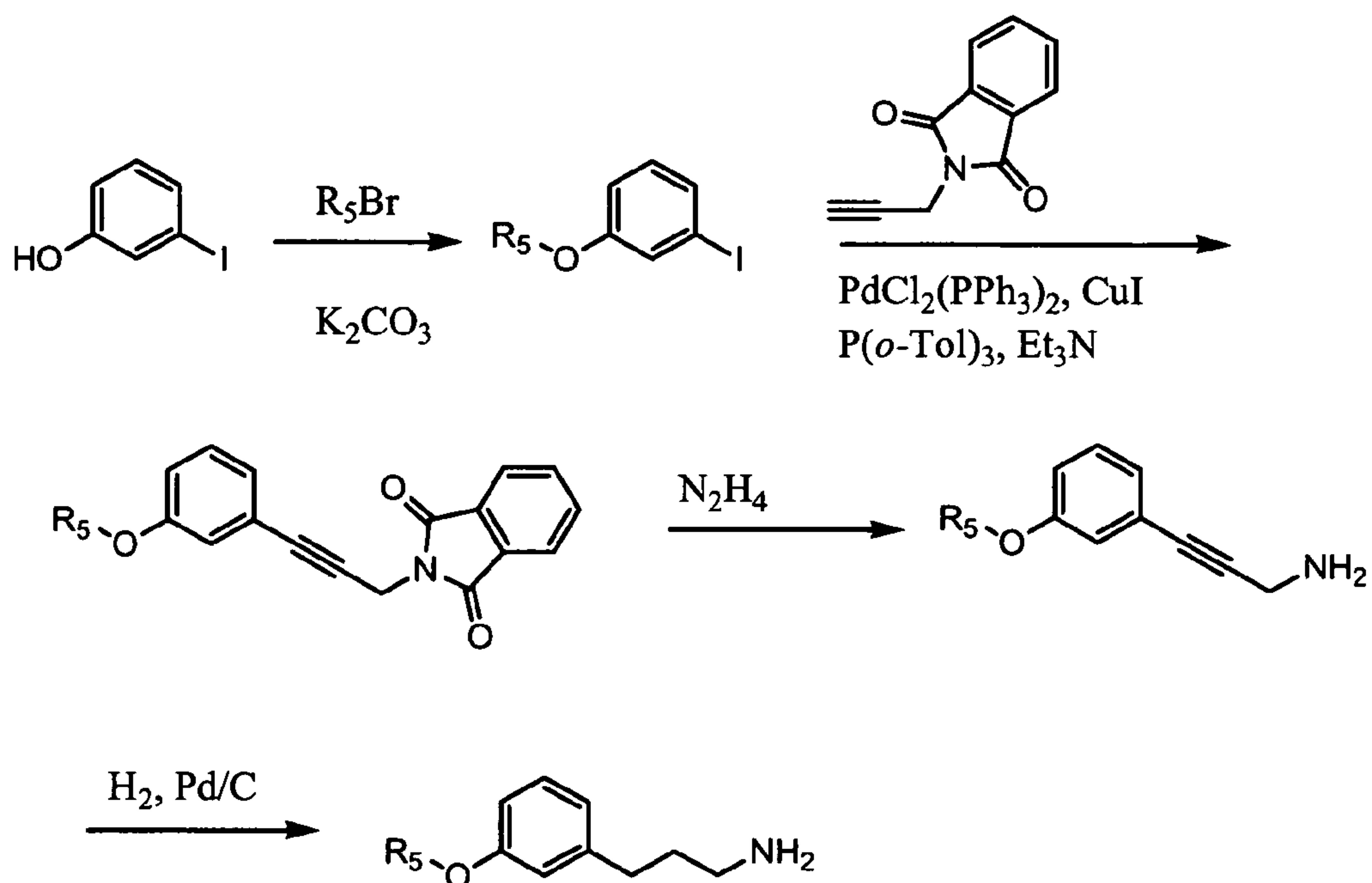
SCHEME I
