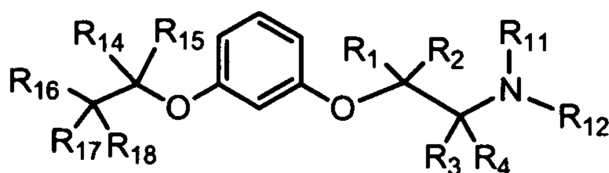
Formula (IIb)
