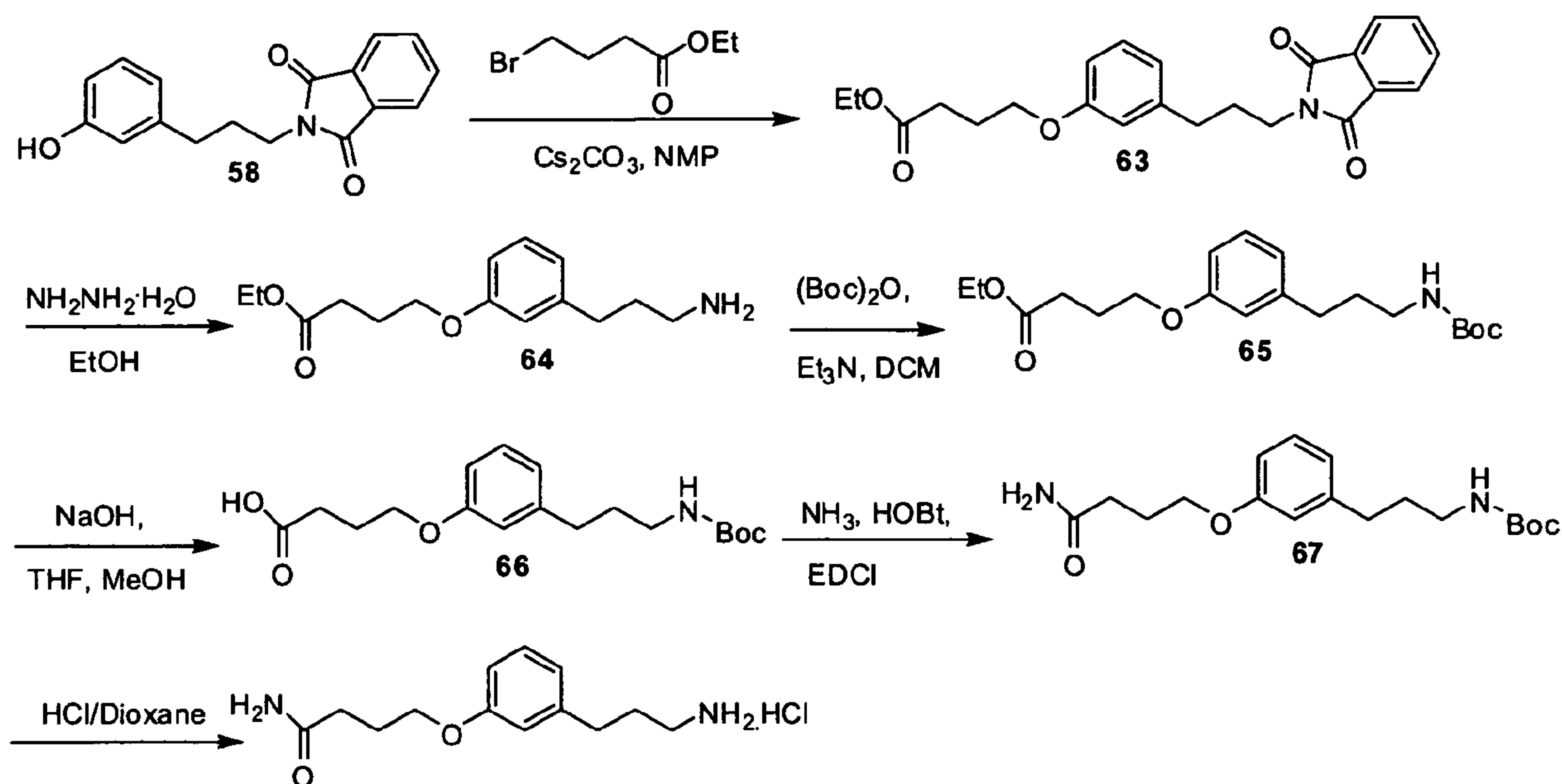
SCHEME 19
