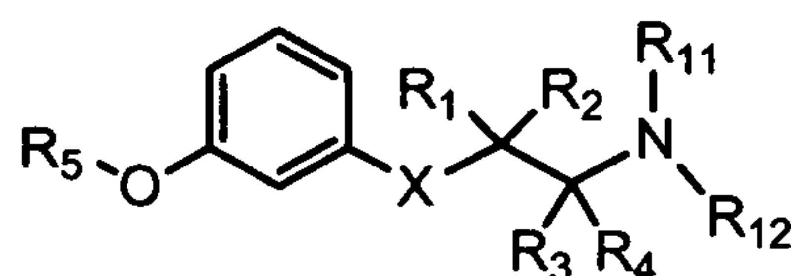
Formula (I)
