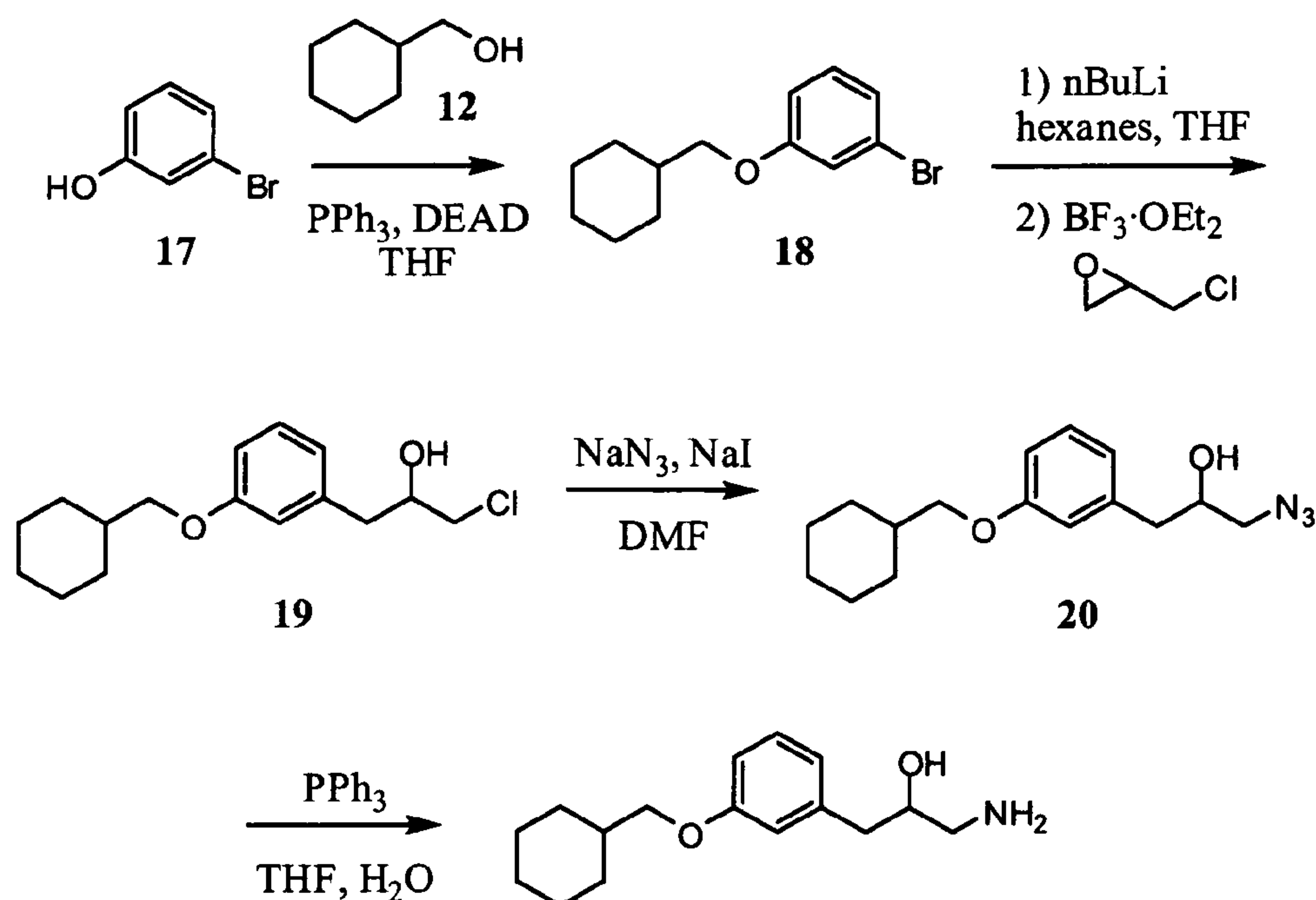
SCHEME 5
