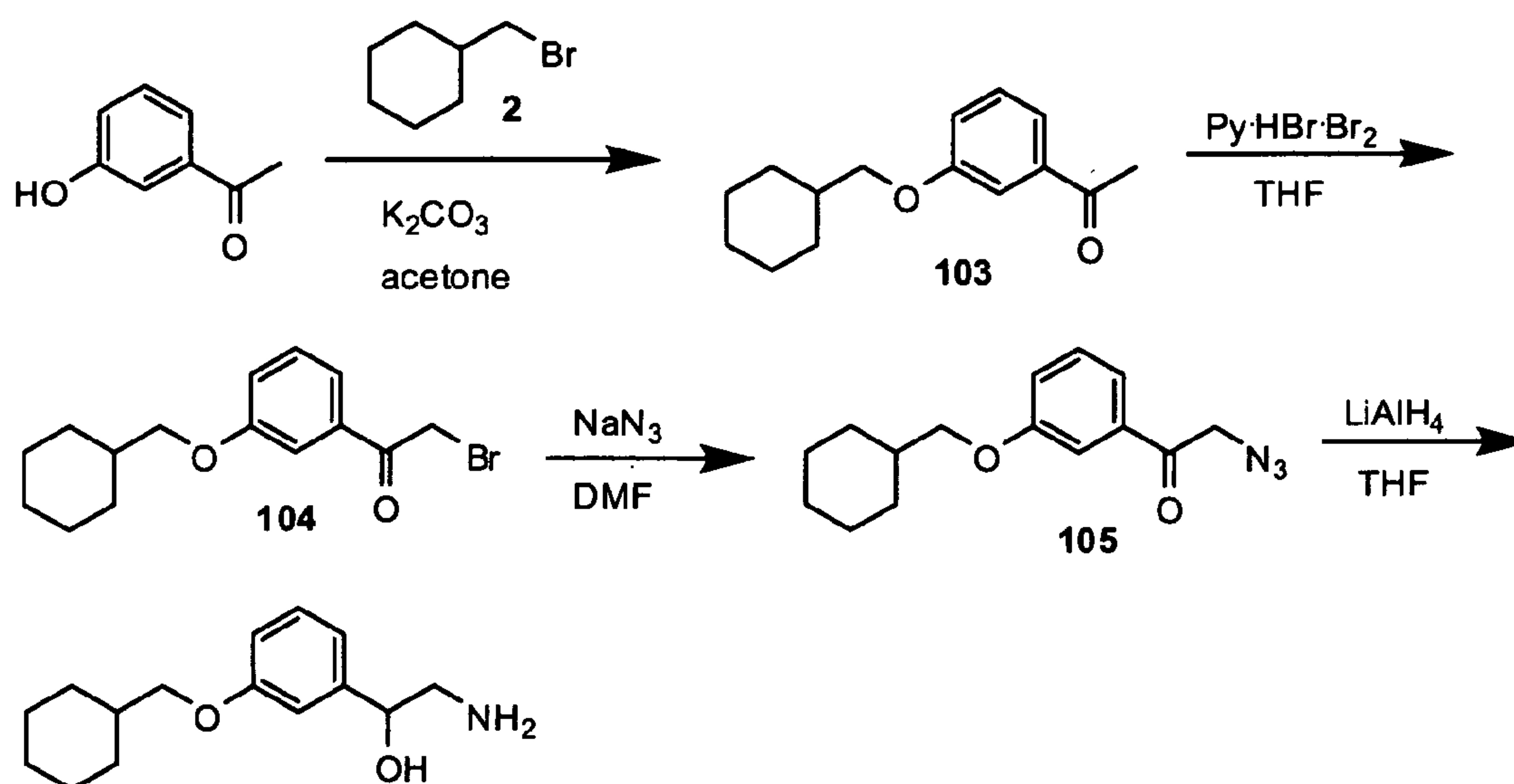
SCHEME 35
