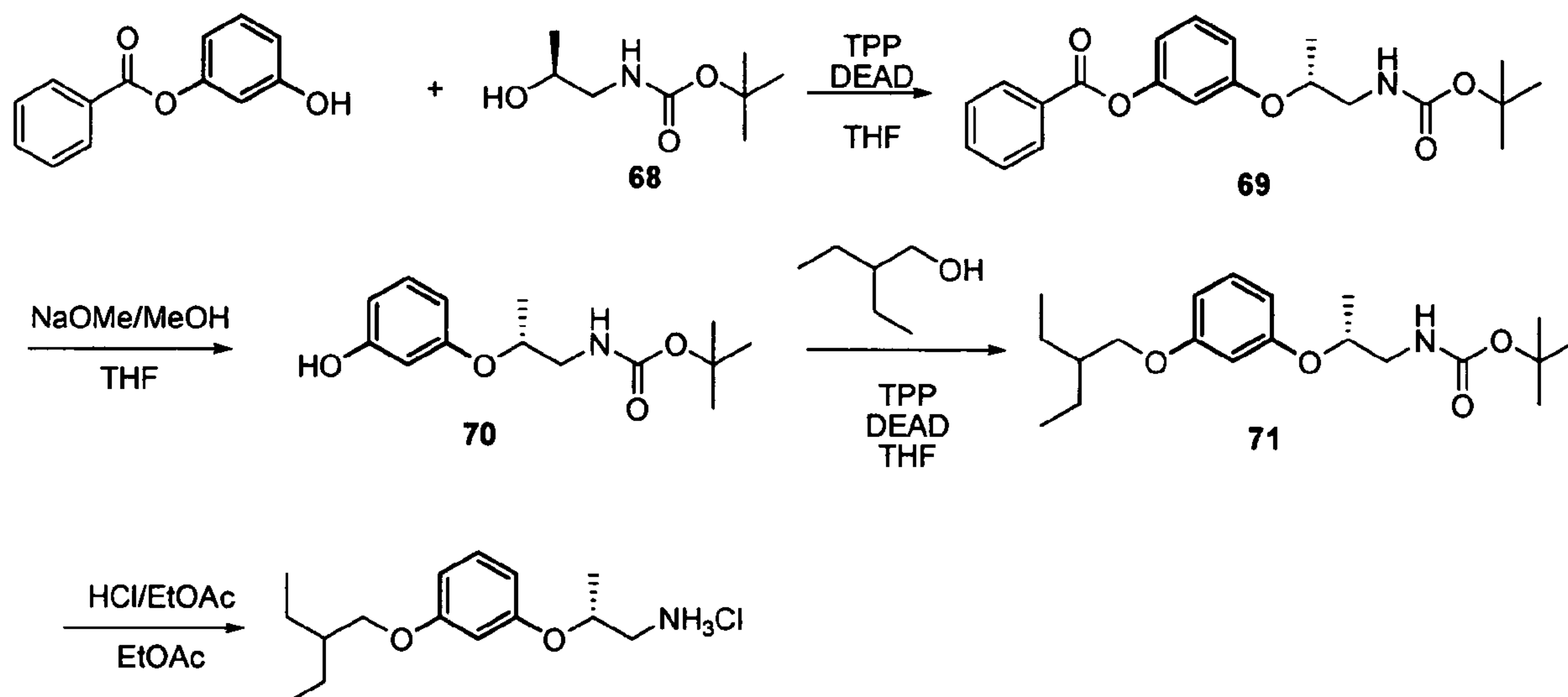
SCHEME 20
