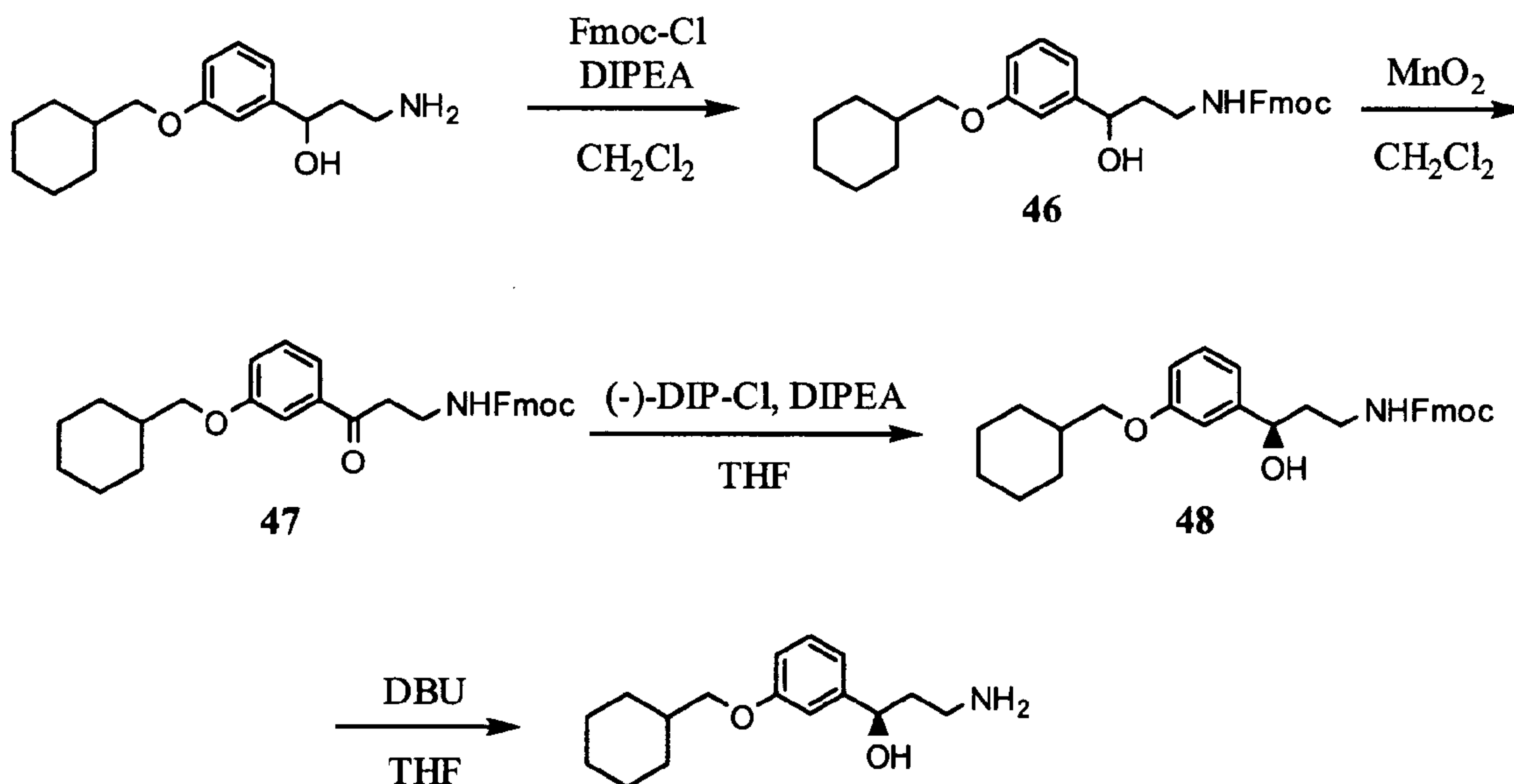
SCHEME 14
