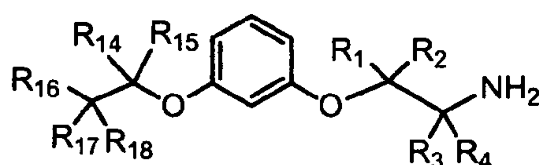
Formula (IIb)
