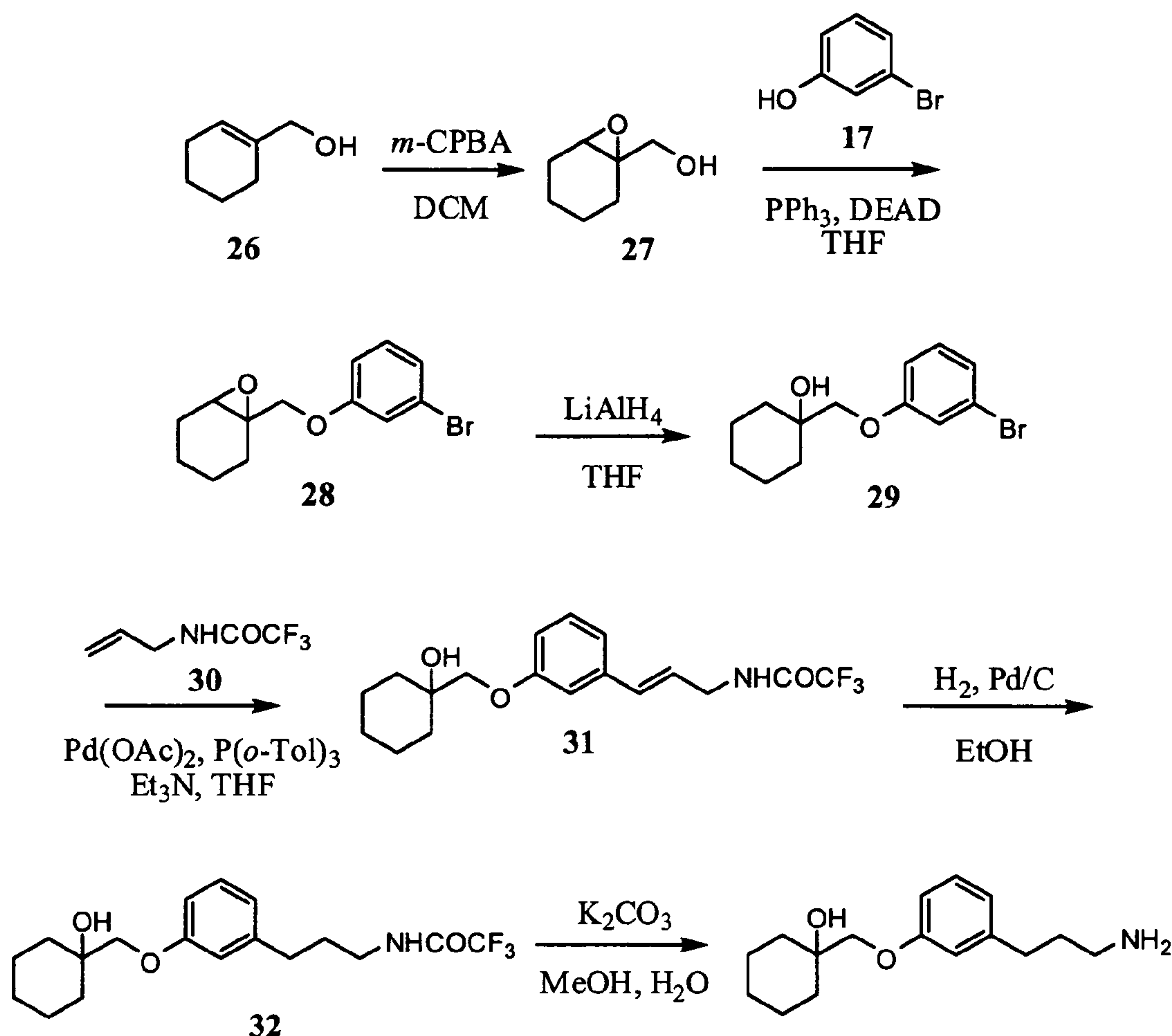
SCHEME 7
