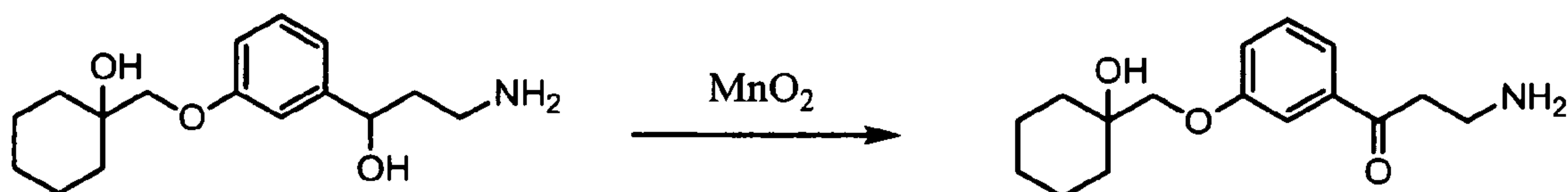
SCHEME 13
