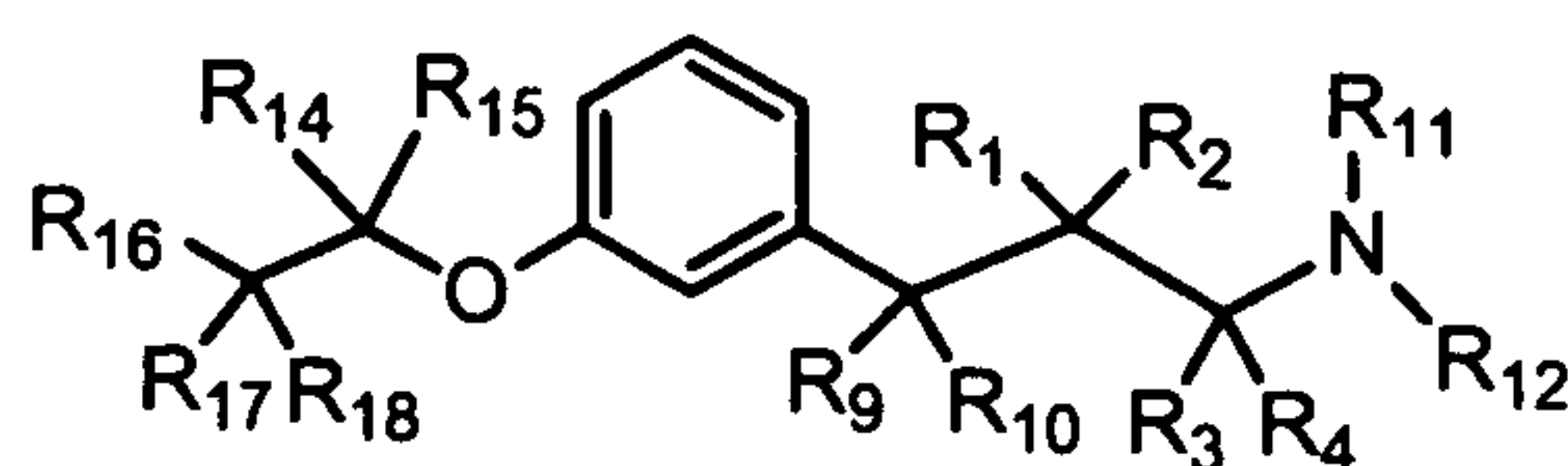
Formula (IIa)
