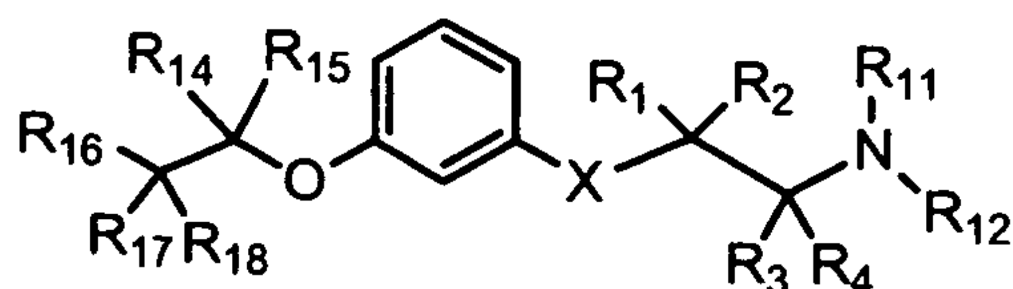
Formula (II)
