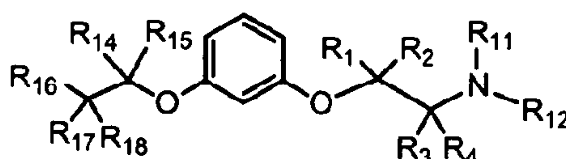
Formula (IIb)
