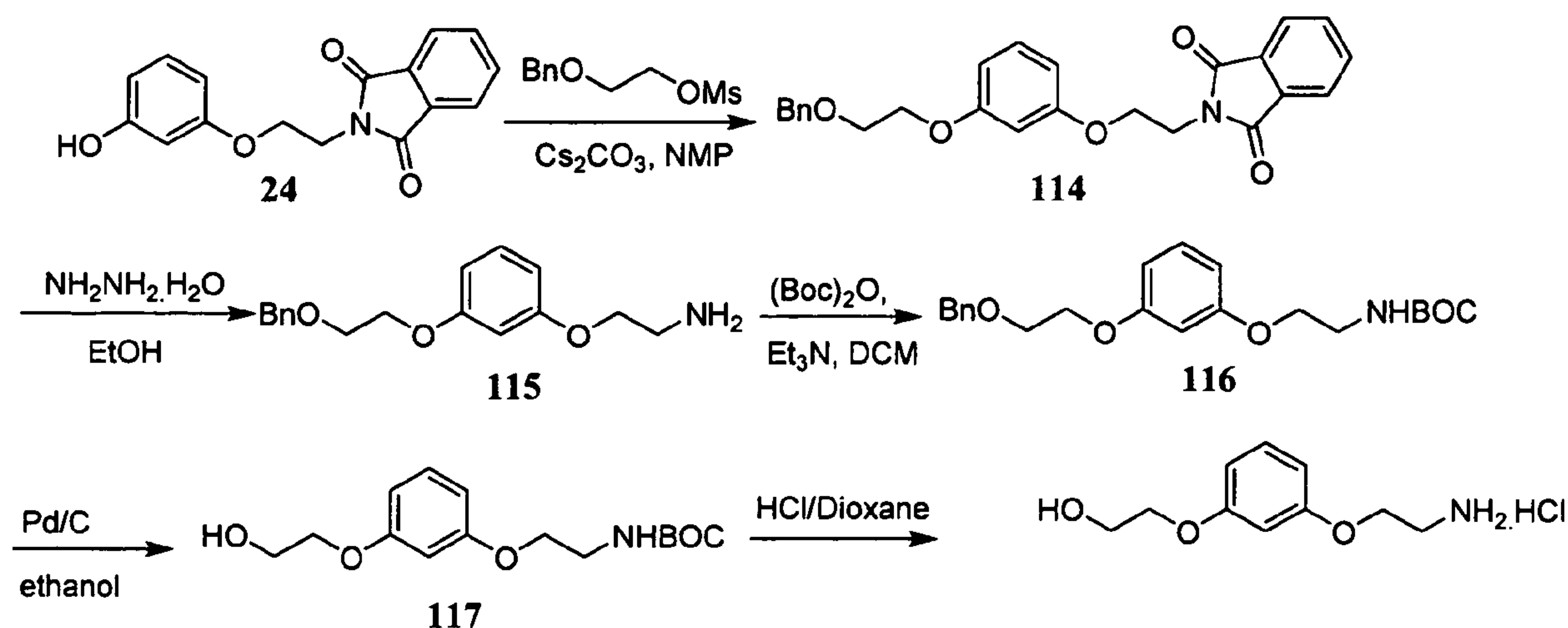
SCHEME 39
