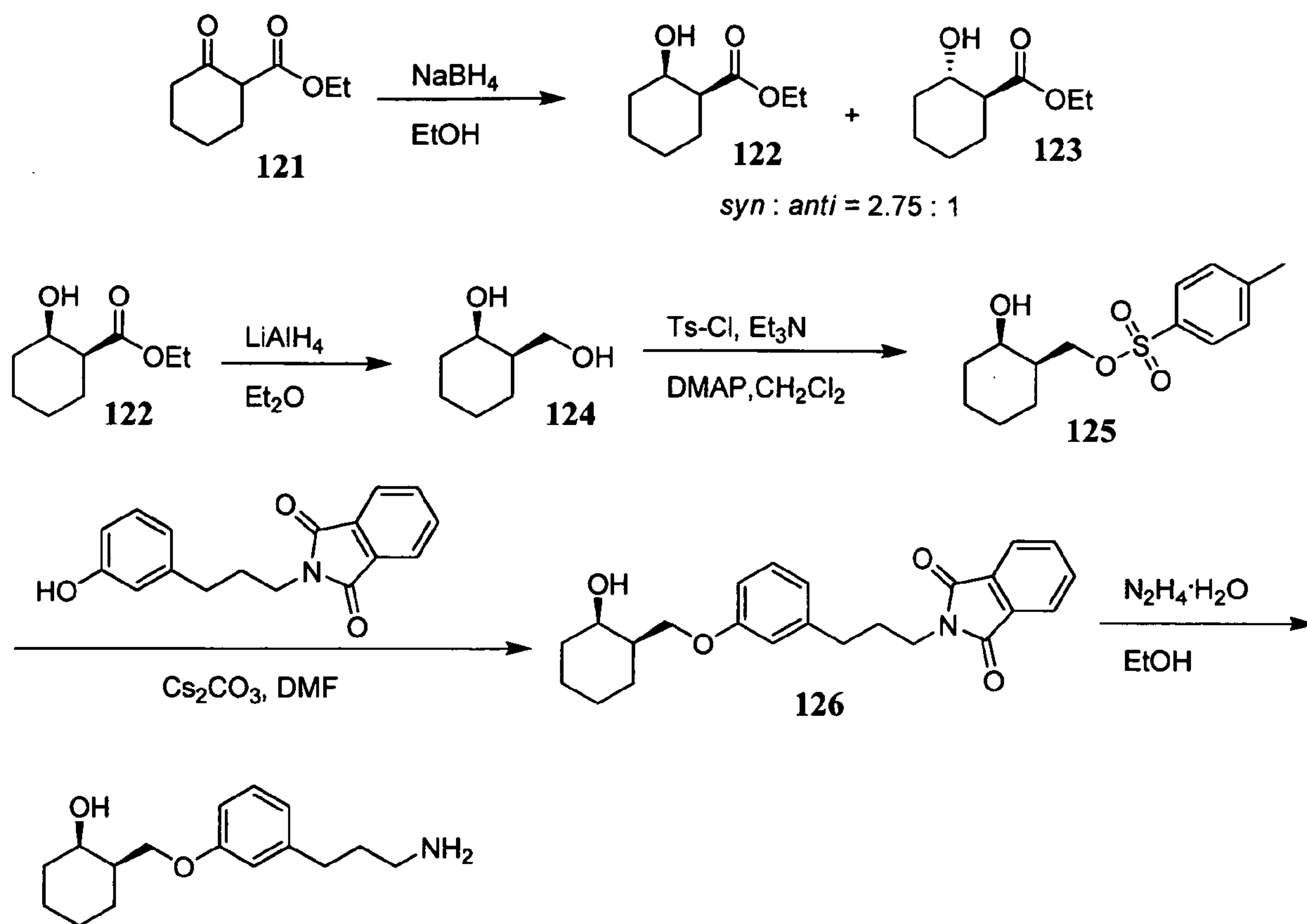
SCHEME 41
