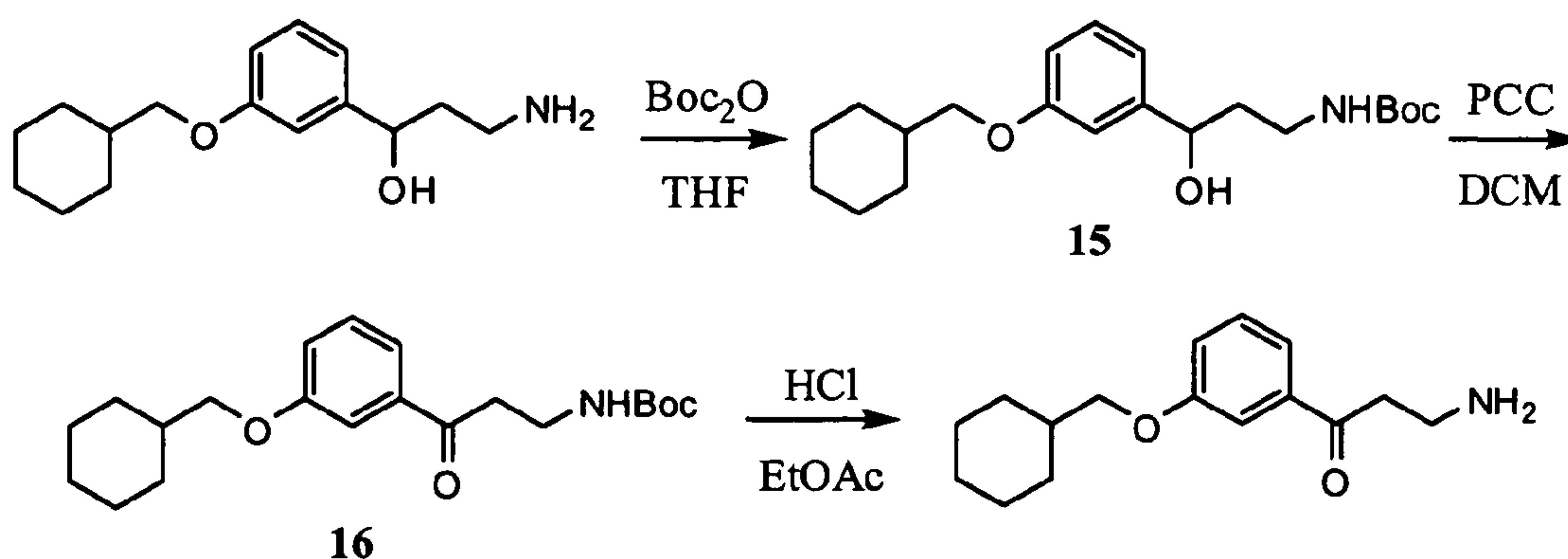
SCHEME 4
