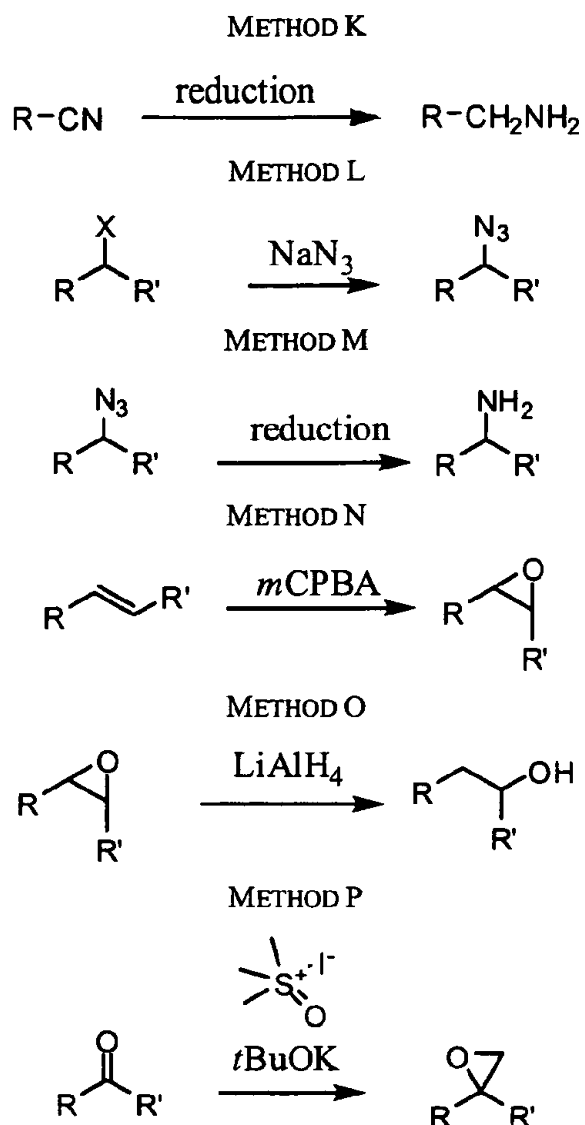
SCHEME I
