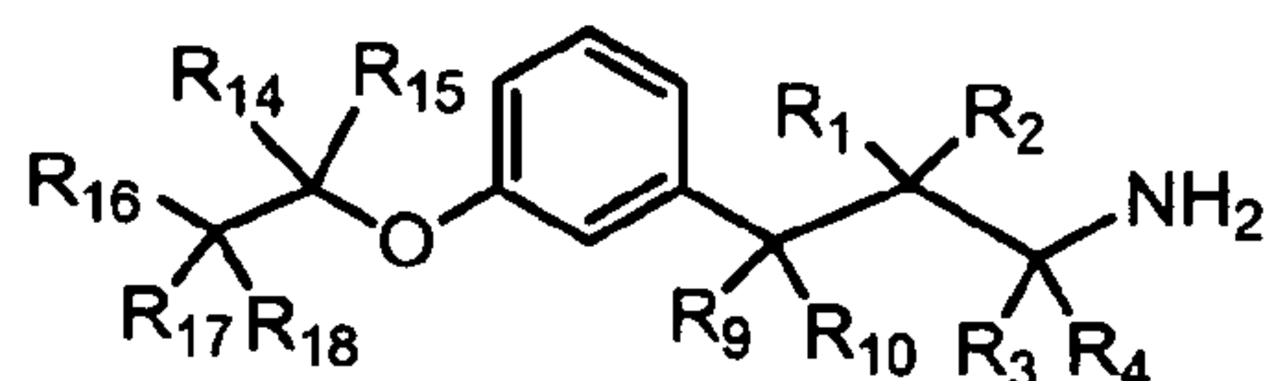
Formula (IIa)
