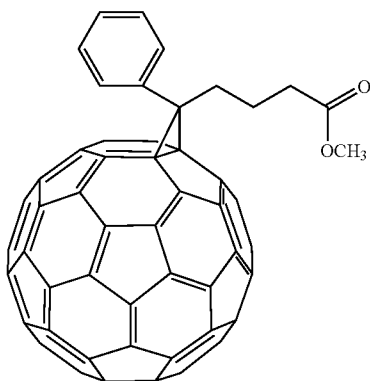
PCBM
