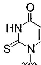
2-thio-U
