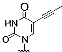
5-propynyl-U
