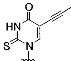
2-thio-5-propynyl-U
