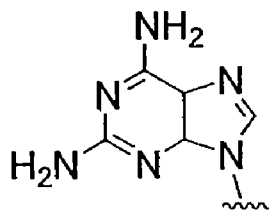
N9-(2,6,-diaminopurine)
