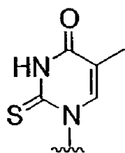
2-thio-T
