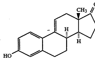
\Delta^9(11) -Dehydro-8-isoestrone(VI)
