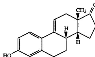
Δ9(11)-Dehydro-8-isoestrone (VI)
