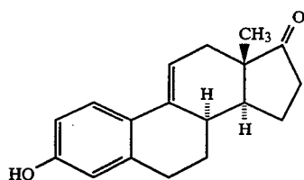
Δ9(11)-Dehydro-8-isoestrone(VI)
