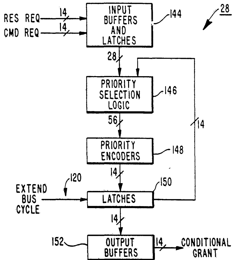
ARBITER BLOCK DIAGRAM
