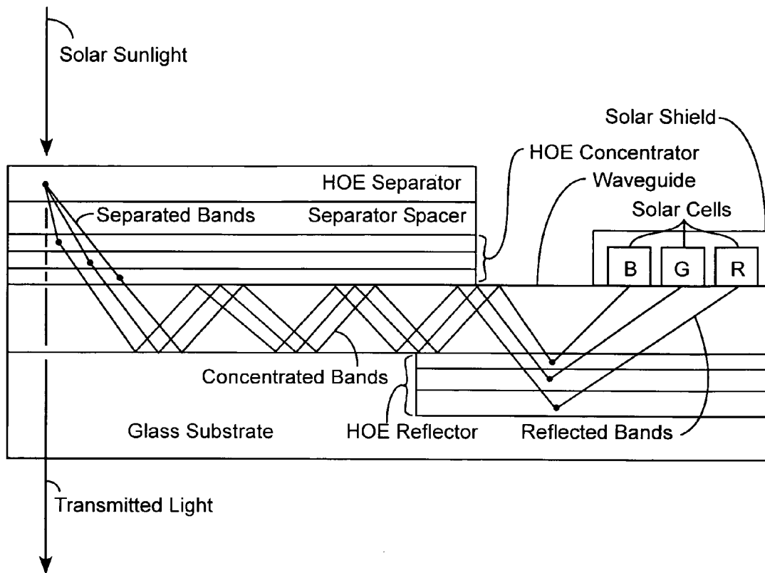
MULTIPLE HOE WAVEGUIDE SERIAL SOLAR CONCENTRATOR
