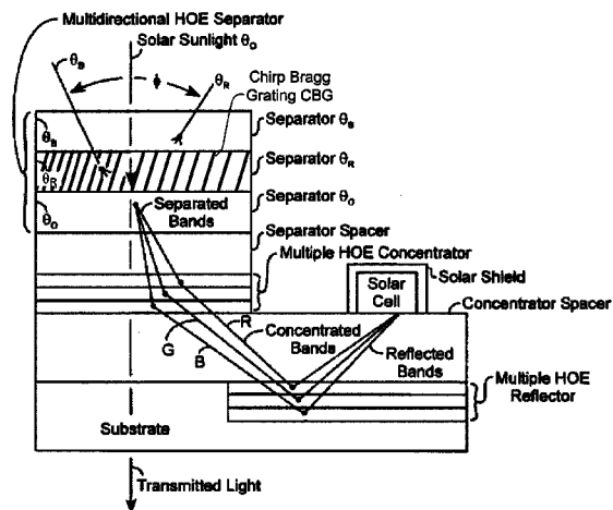
MULTIDIRECTIONAL MULTIPLE HOE SOLAR CONCENTRATOR
