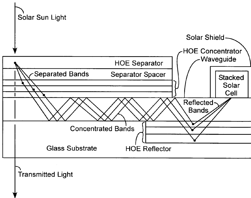
MULTIPLE HOE WAVEGUIDE STACKED SOLAR CONCENTRATOR
