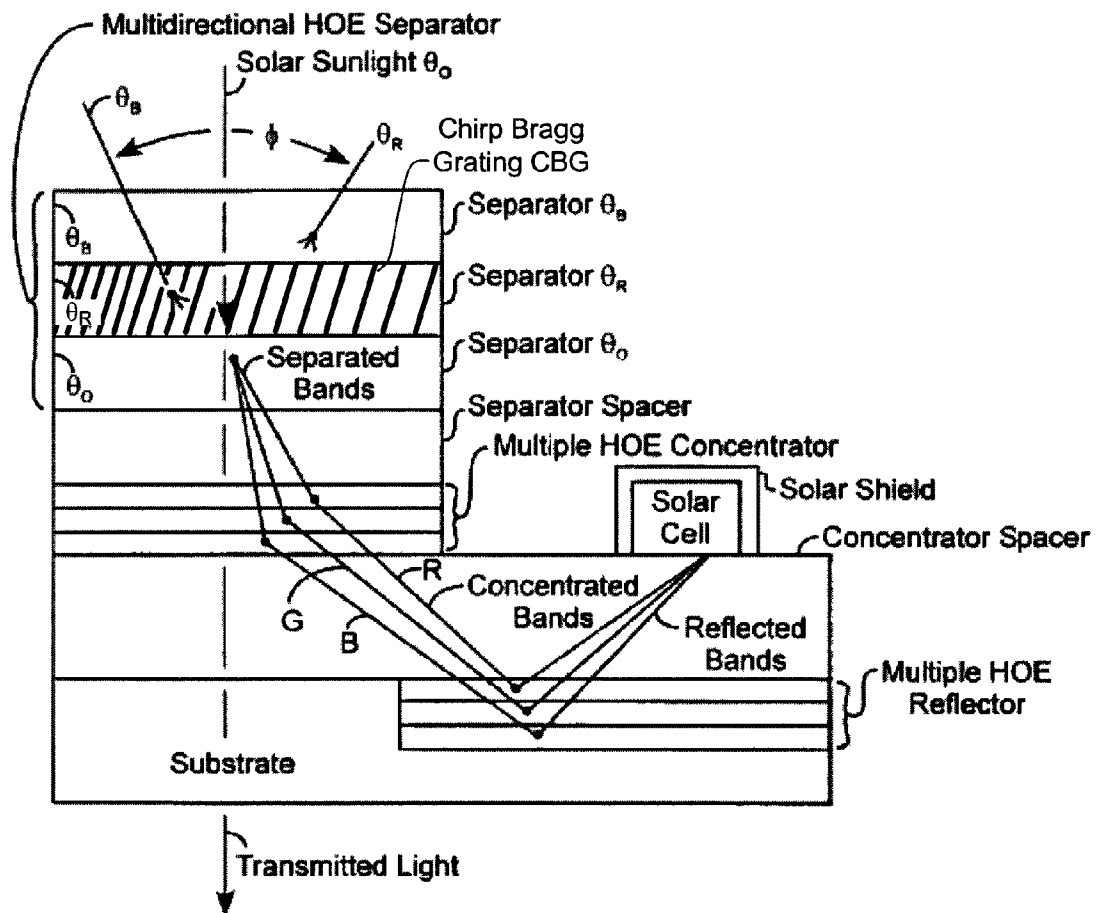
MULTIDIRECTIONAL MULTIPLE HOE SOLAR CONCENTRATOR
