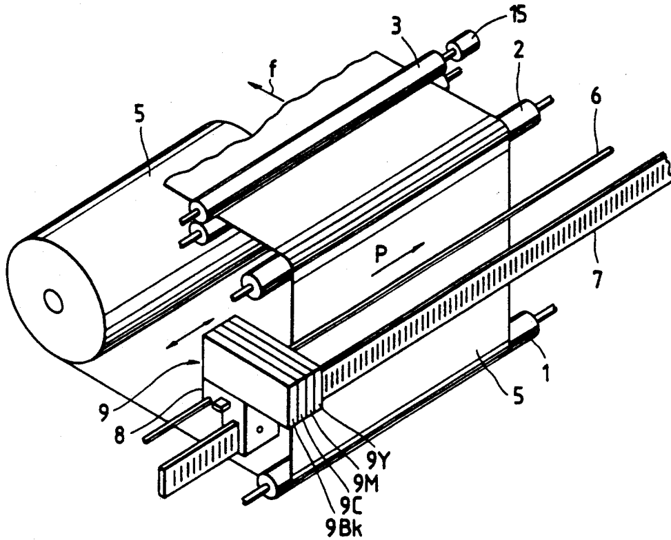
FIG. 1 PRIOR ART
