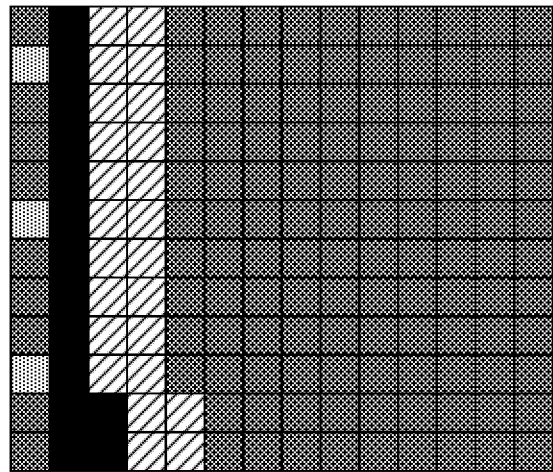
DMRS HARQ ACK (puncture the data) HARQ ACK (rate matching is performed on the data) CSI uplink data
