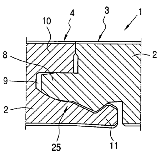
FIG. 4 PRIOR ART
