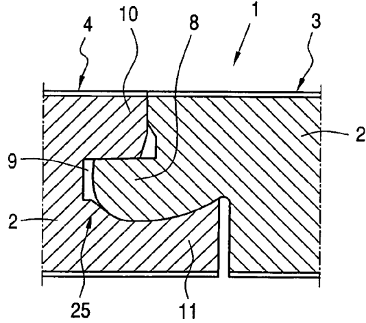
FIG. 5 PRIOR ART
