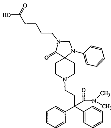
Compound AP, 5-[8-(3-Dimethylcarbamoyl-3,3-diphenyl-propyl)- 4-oxo-1-phenyl-1,3,8-triaza-spiro[4.5]dec-3-yl]-pentanoic acid;
