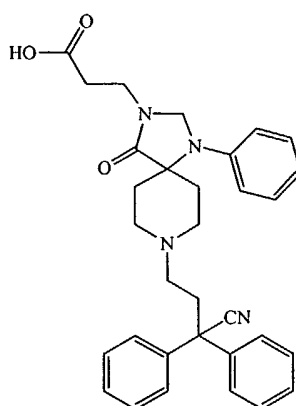
Compound AV, 3-[8-(3-Cyano-3,3-diphenyl-propyl)-4-oxo-1-phenyl-1,3,8-triaza-spiro[4.5]dec-3-yl]-propionic acid;
