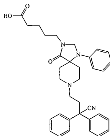
Compound AU, 5-[8-(3-Cyano-3,3-diphenyl-propyl)-4-oxo-1-phenyl-1,3,8-triaza-spiro[4.5]dec-3-yl]-pentanoic acid;
