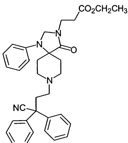
Compound G 3-[8-(3-cyano-3,3-diphenyl-propyl)-4-oxo-1-phenyl-1,3,8-triaza-spiro[4.5]dec-3-yl]-propionic acid ethyl ester;
