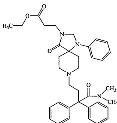
Compound AR, 3-[8-(3-Dimethylcarbamoyl-3,3-diphenyl-propyl)- 4-oxo-1-phenyl-1,3,8-triaza-spiro[4.5]dec-3-yl]-propionic acid ethyl ester;
