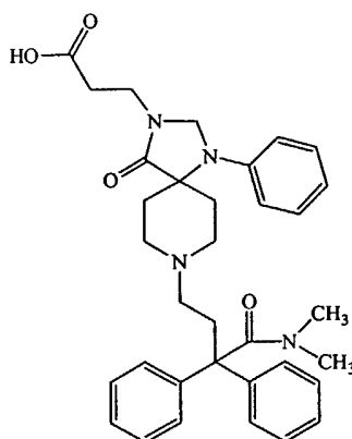
Compound AT, 3-[8-(3-Dimethylcarbamoyl-3,3-diphenyl-propyl)- 4-oxo-1-phenyl-1,3,8-triaza-spiro[4.5]dec-3-yl]-propionic acid; and pharmaceutically acceptable salts thereof.
