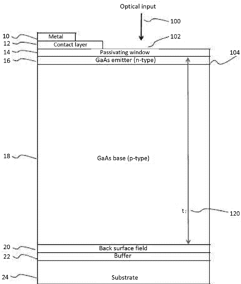
Figure 1 Prior Art
