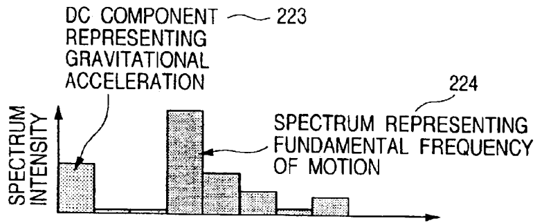
FIG. 5(b) TYPICAL RESULT OF HAVING OBSERVED WAVEFORM PARTITIONED BY WINDOW FUNCTION AND SUBJECTED TO SPECTRUM ANALYSIS
