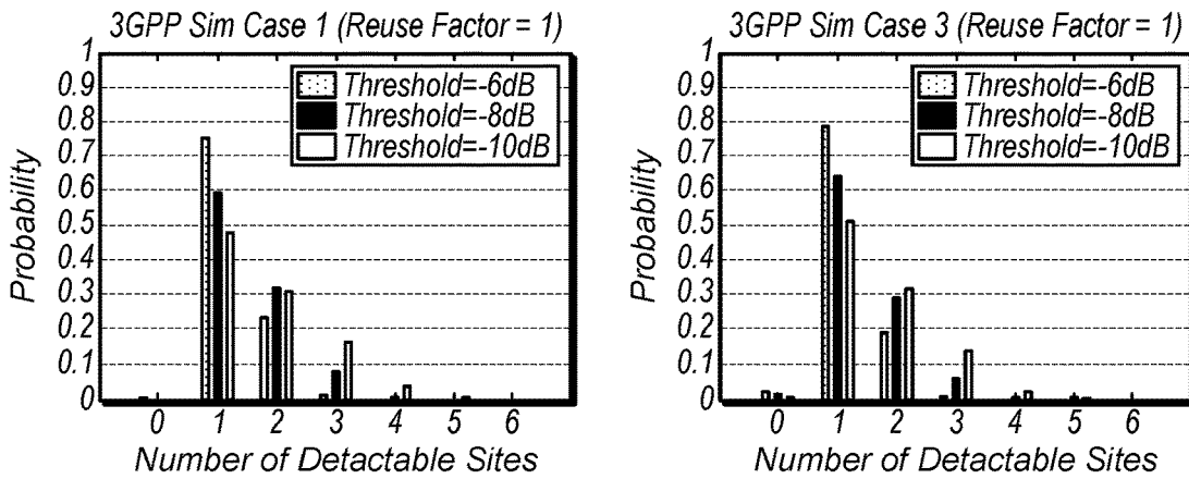
Distributions of Number of Detectable Sites (Reuse Factor = 1) FIG. 4
