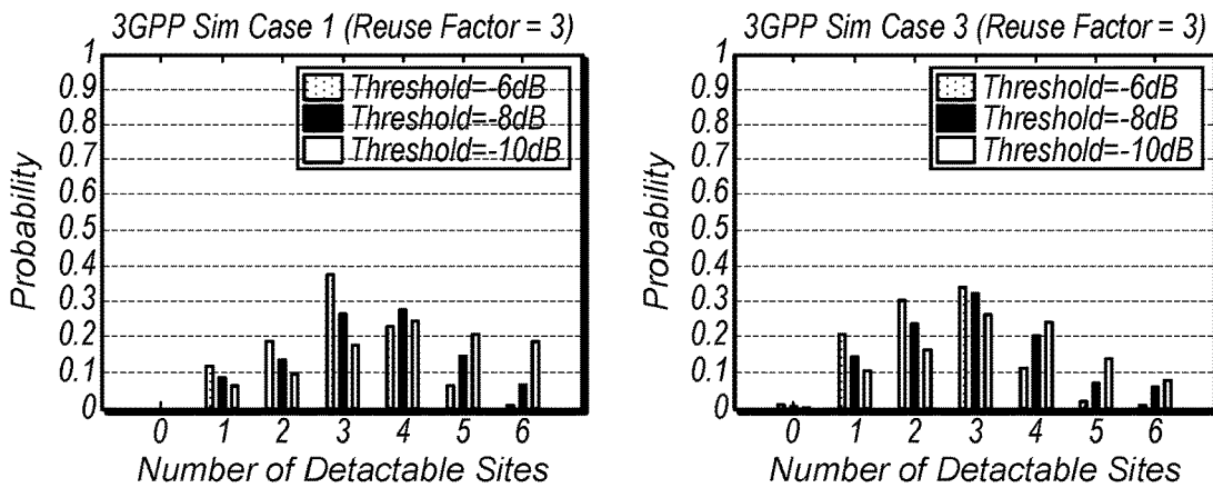
Distributions of Number of Detectable Sites (Reuse Factor = 3) FIG. 5
