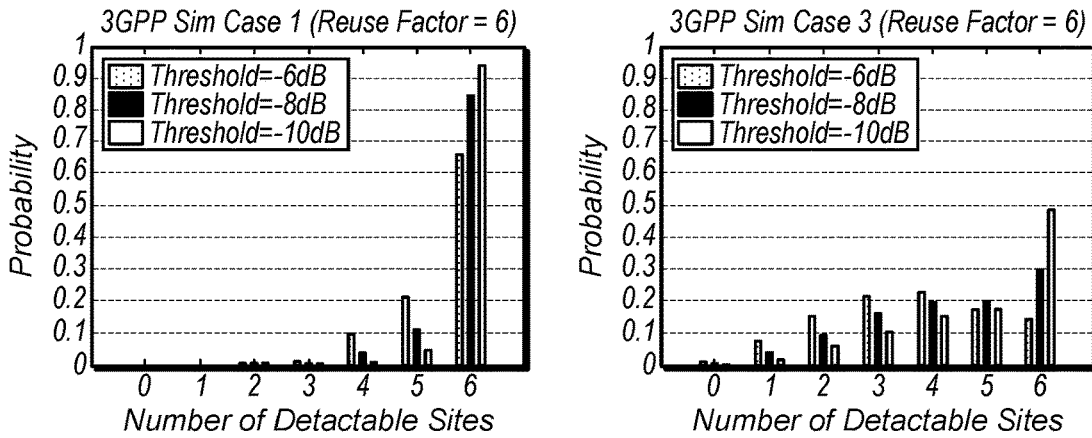
Distributions of Number of Detectable Sites (Reuse Factor = 6) FIG. 6
