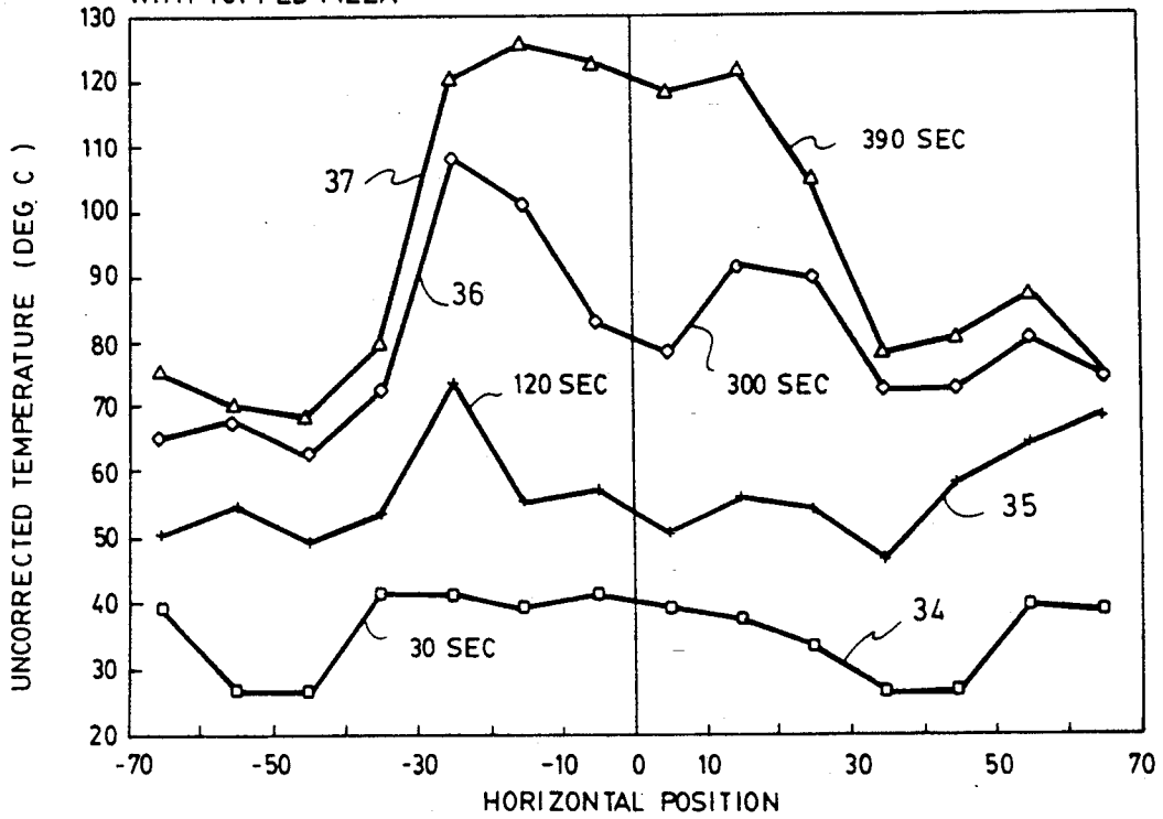
TEMP. PROFILE OF SCORED PIZZA SUSCEPTOR WITH TOPPED PIZZA
