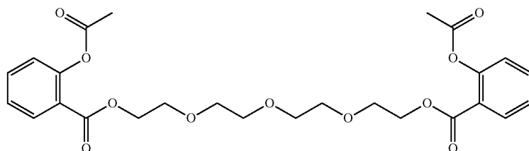
Tetraethylene glycol(aspirin) 2
