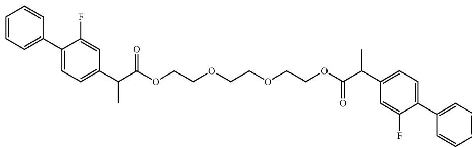
Tetraethylene glycol(flurbiprofen) 2
