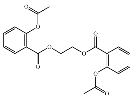
Ethylene glycol(aspirin) 2
