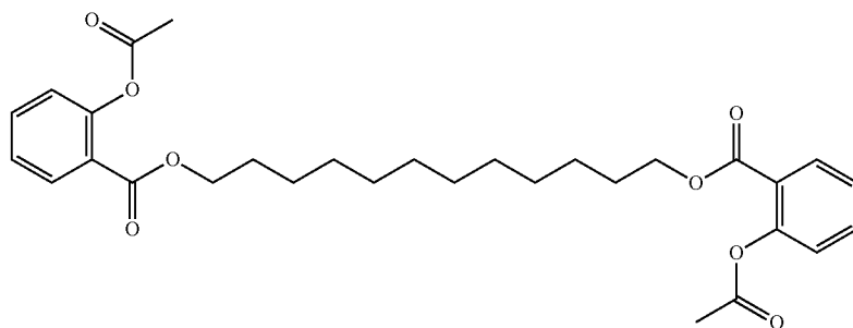
1,12-Dodecanediol(aspirin) 2
