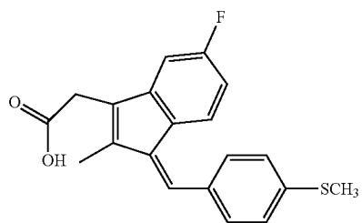
Sulindac sulfide
