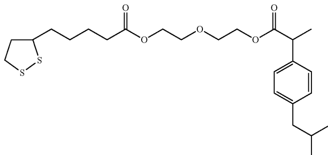
(\alpha -Lipoic acid)-diethylene glycol(ibuprofen)
