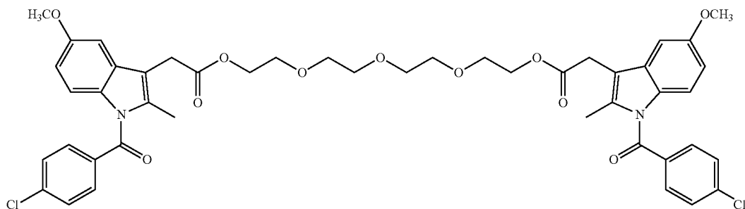
Tetraethylene glycol(indomethacin) 2
