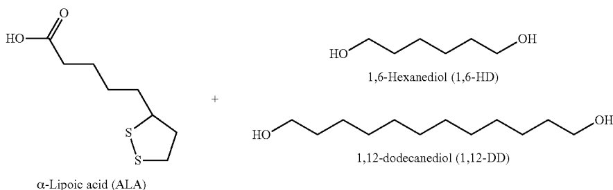
\alpha -Lipoic acid (ALA)
