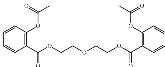
Diethylene glycol(aspirin) 2
