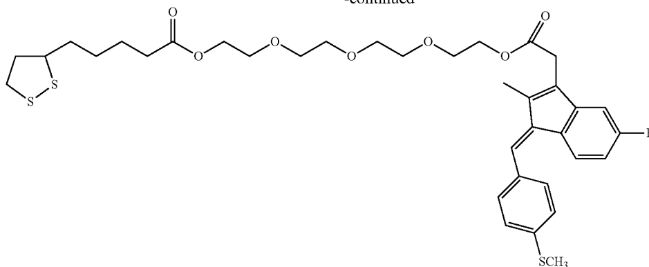
(α-Lipoic acid)-tetraethylene glycol(sulindac sulfide)
