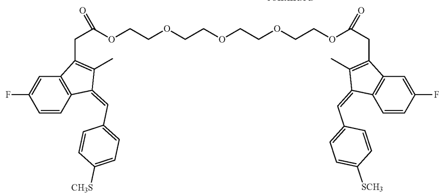
Tetraethylene glycol(sulindac sulfide) 2
