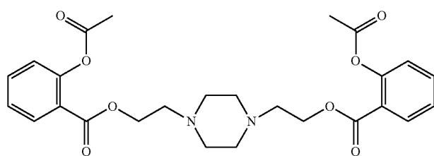
[1,4]Bis(2-hydroxyethyl)-piperazine](Aspirin) 2
