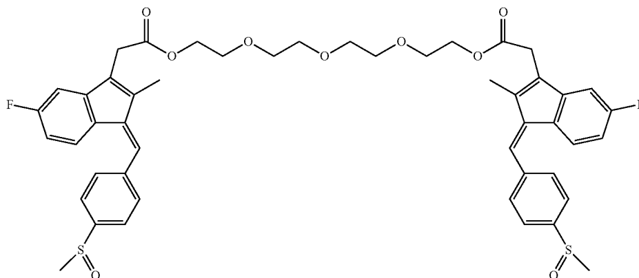
Tetraethylene glycol(sulindac) 2
