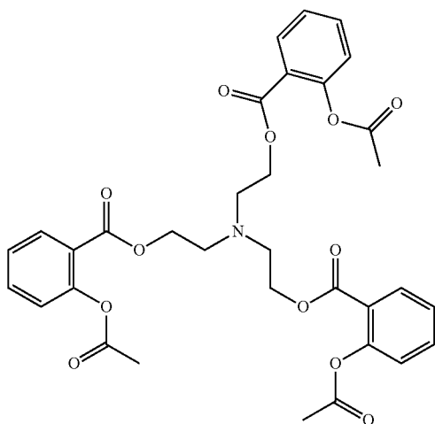
Triethanolamine (Aspirin) 2
