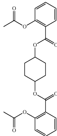
1,4-Cyclohexanediol (Aspirin) 2
