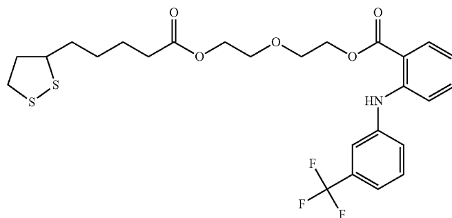
( \alpha -Lipoic acid)-diethylene glycol(flufenamic acid)
