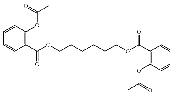
1,6-Hexanediol(aspirin) 2
