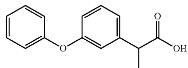
Fenoprofen
