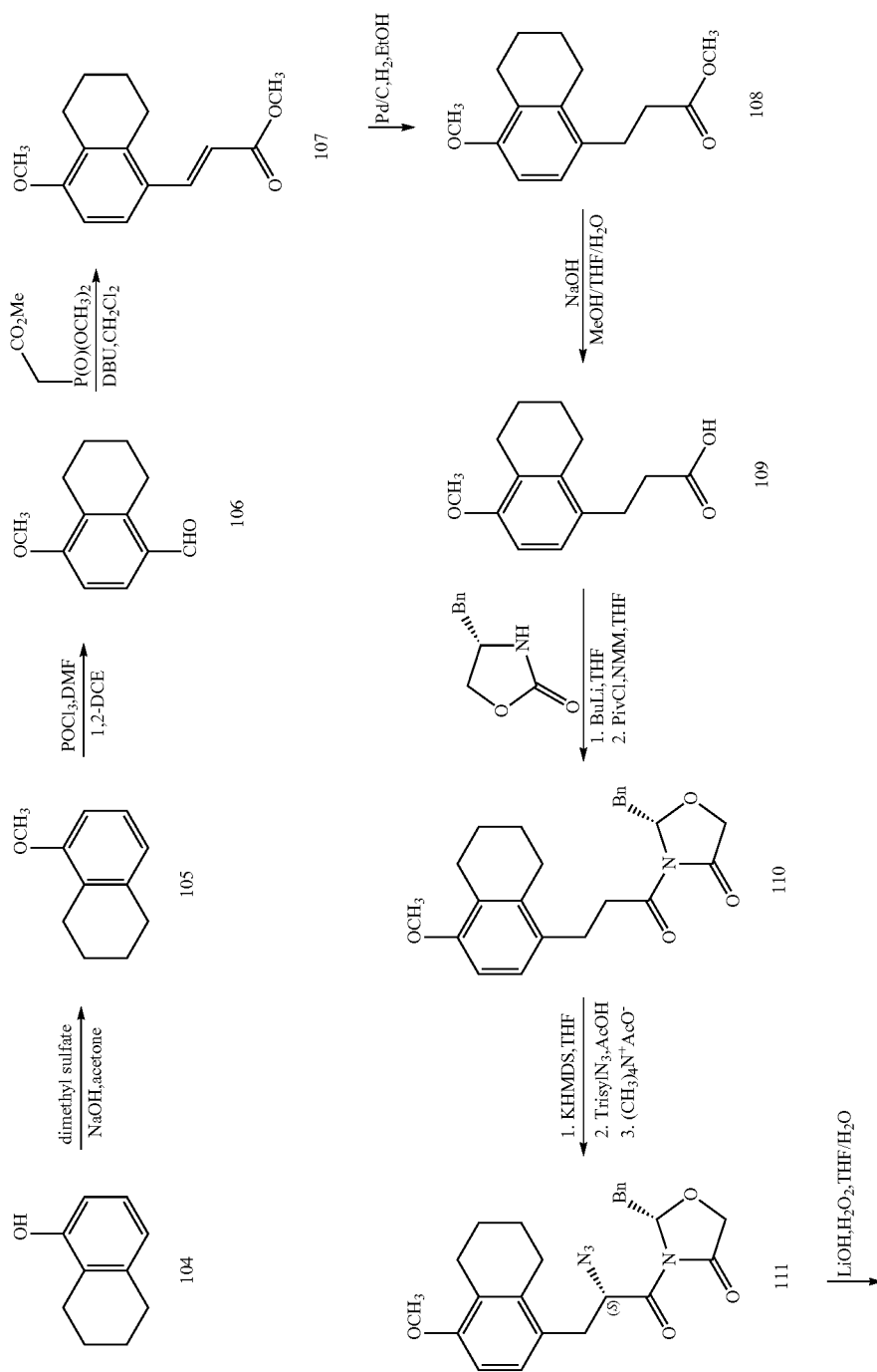
Scheme 17
