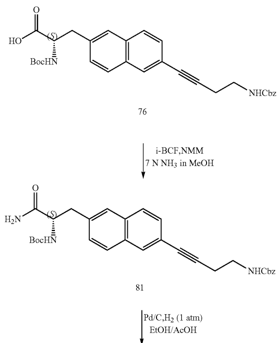
Scheme 12
