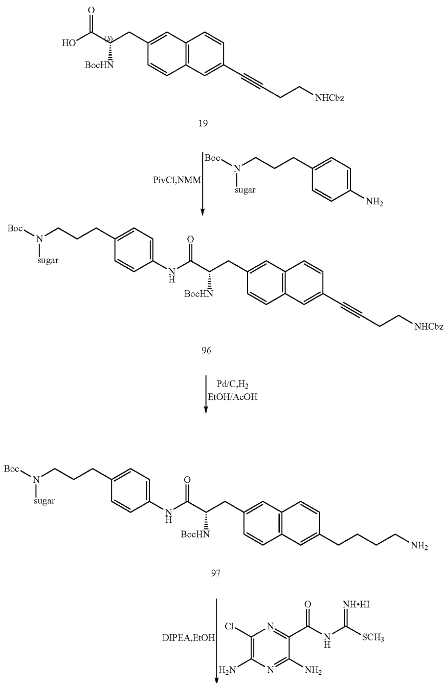
Scheme 15
