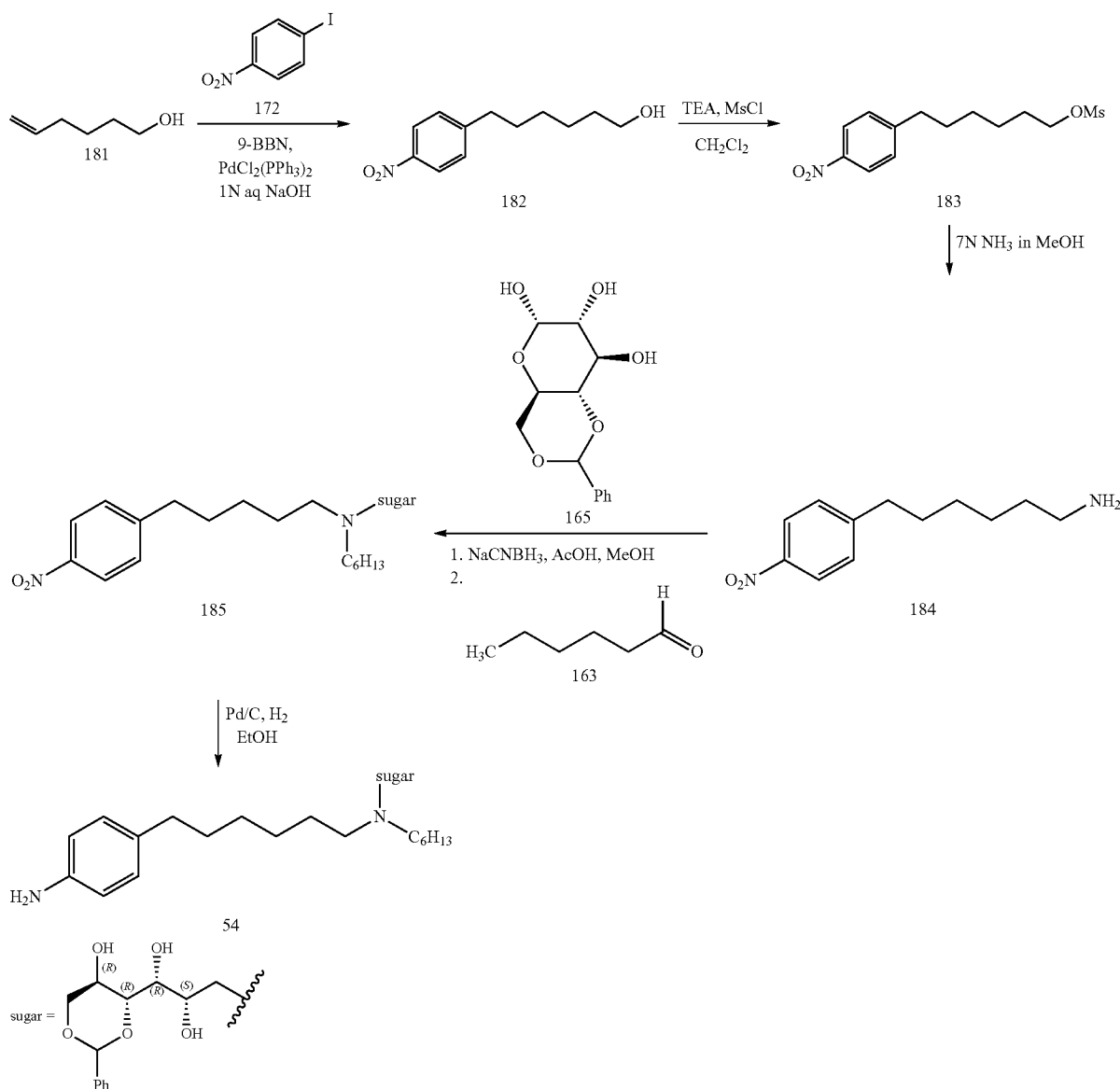
Scheme 34
