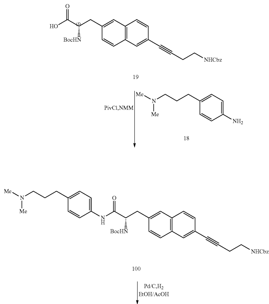
Scheme 16
