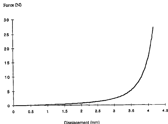
Compression of 5 mm disk (5 mm diameter) at 2 mm/min
