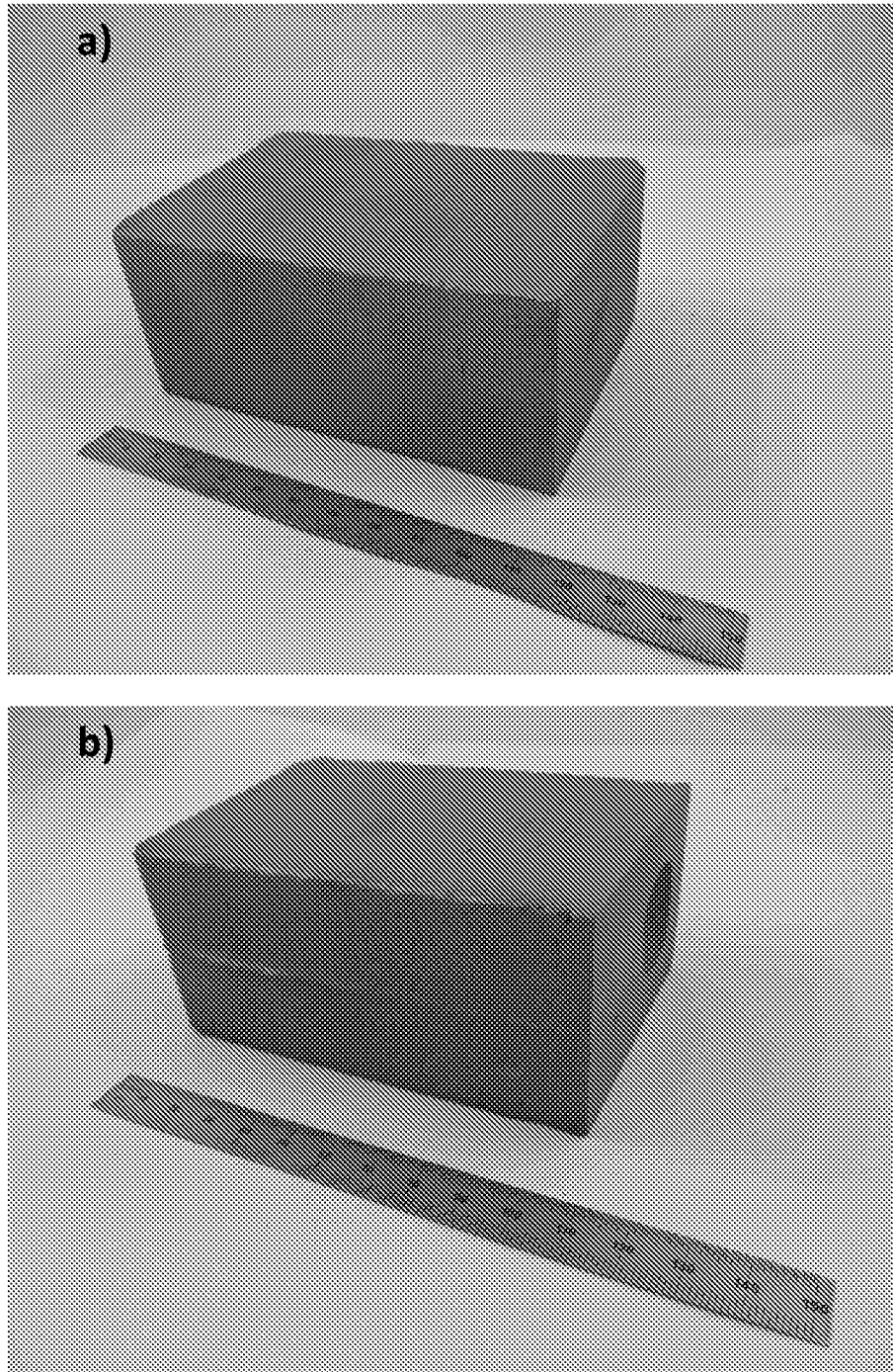
FIG. 5 Images of laboratory cast 50 mm slabs from; a) Alloy 6 and b) Alloy 9.
