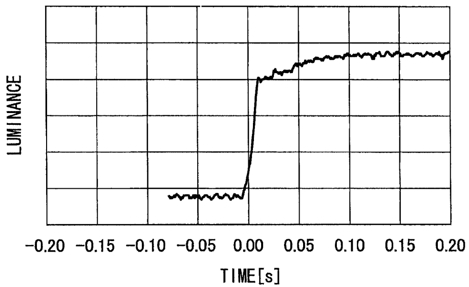
RESPONSE WAVEFORM 0→64
