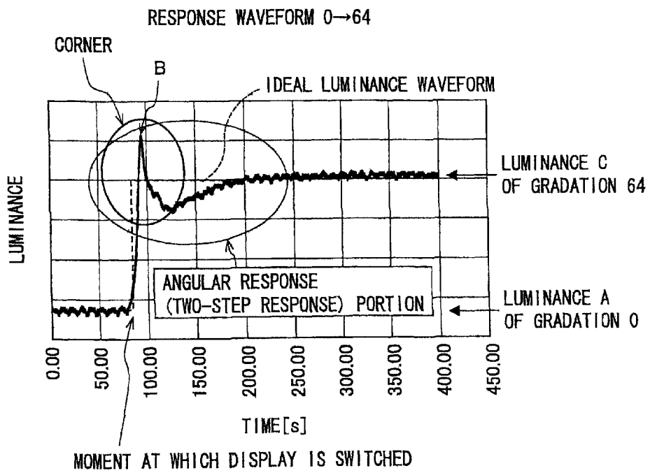
FIG. 12 Conventional Art
