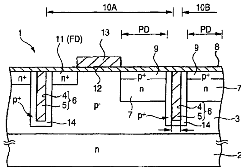
FIG. 24 (PRIOR ART)
