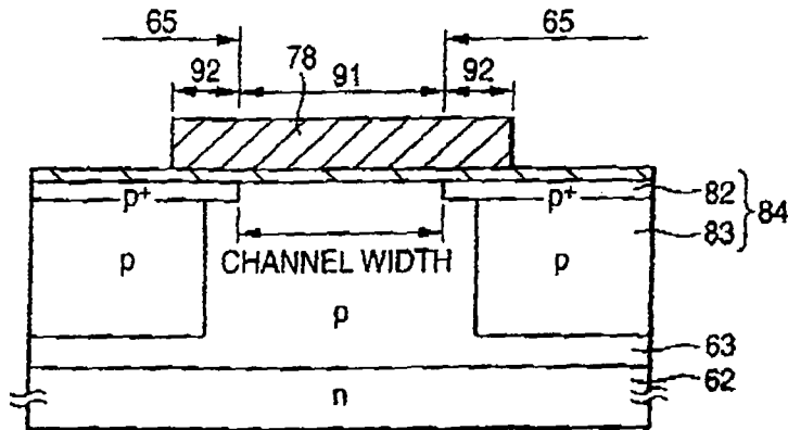
FIG. 2C C-C CROSS SECTION
