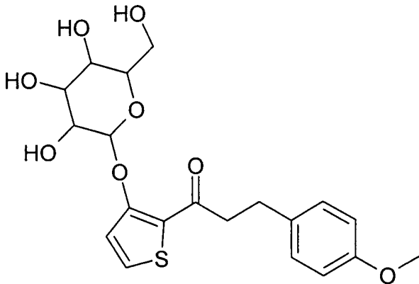
3-(4-Methoxy-phenyl)-1-[3-(3,4,5-trihydroxy-6-hydroxymethyl-tetrahydro-pyran-2-yloxy)-thiophen-2-yl]-propan-1-on
