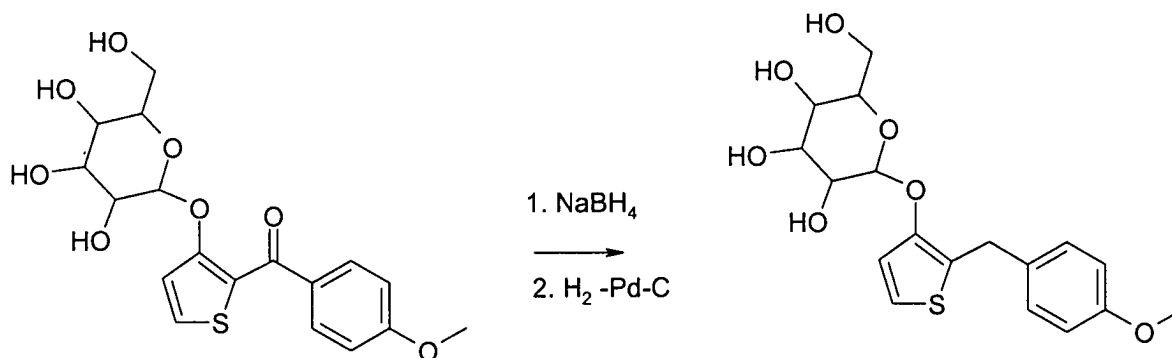
d) 2-Hydroxymethyl-6-[2-(4-methoxy-benzyl)-thiophen-3-yloxy]-tetrahydro-pyran-3,4,5-triol
