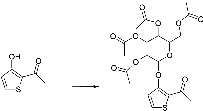
a) Essigsäure-4,5-diacetoxy-6-acetoxymethyl-2-(2-acetyl-thiophen-3-yloxy)-tetrahydro-pyran-3-yl-ester
