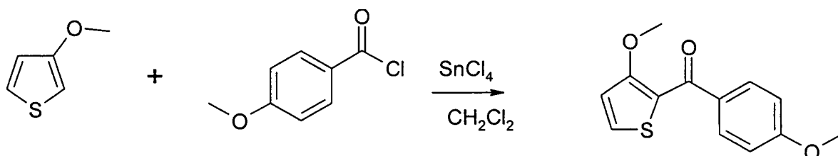
a) (4-Methoxy-phenyl)-(3-methoxy-thiophen-2-yl)-methanon
