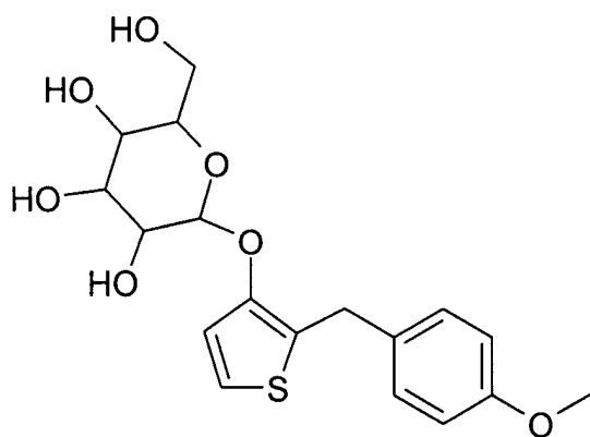
2-Hydroxymethyl-6-[2-(4-methoxy-benzyl)-thiophen-3-yloxy]-tetrahydro-pyran-3,4,5-triol
