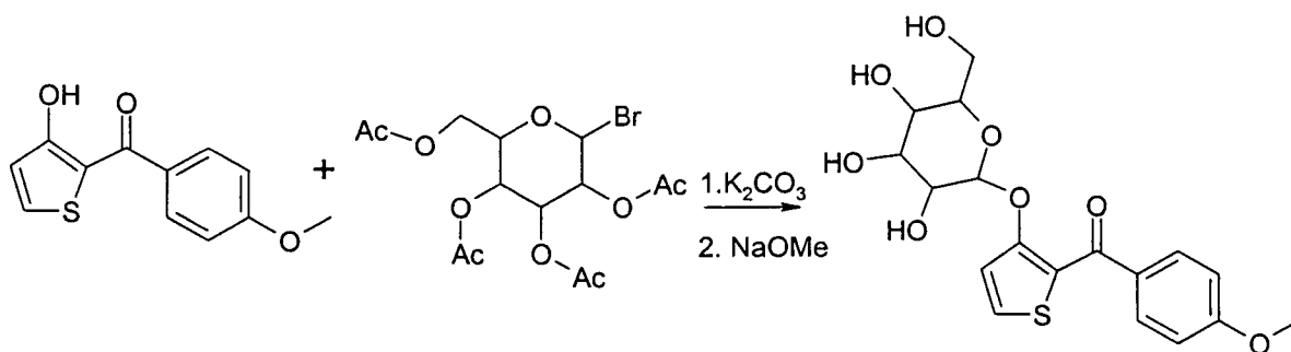
c) (4-Methoxy-phenyl)-[3-(3,4,5-trihydroxy-6-hydroxymethyl-tetrahydro-pyran-2-yloxy)-thiophen-2-yl]-methanon = Beispiel 8
