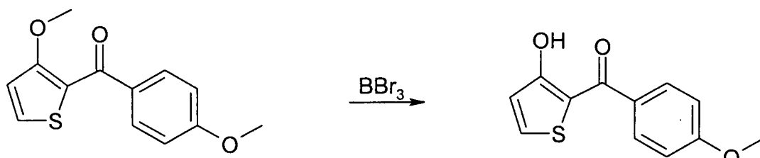
b) (3-Hydroxy-thiophen-2-yl)-(4-methoxy-phenyl)-methanon
