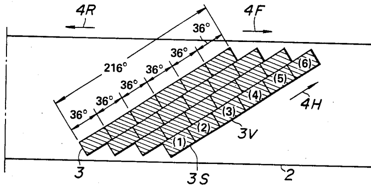
FIG. 3 (PRIOR ART)
