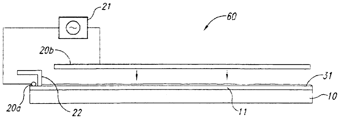
Fig. 1 (Prior Art)
