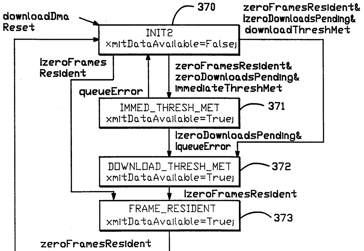
Data Available Control State Diagram
