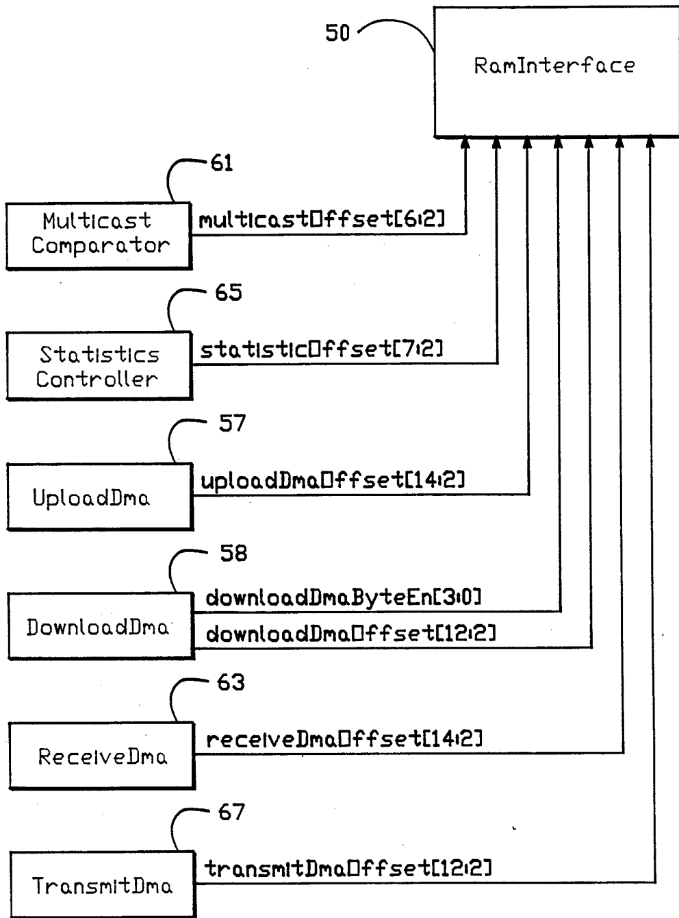
Autonomous Access Address Bus Structure
