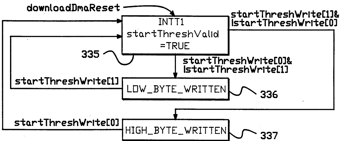
Start Thresh Valid State Diagram
