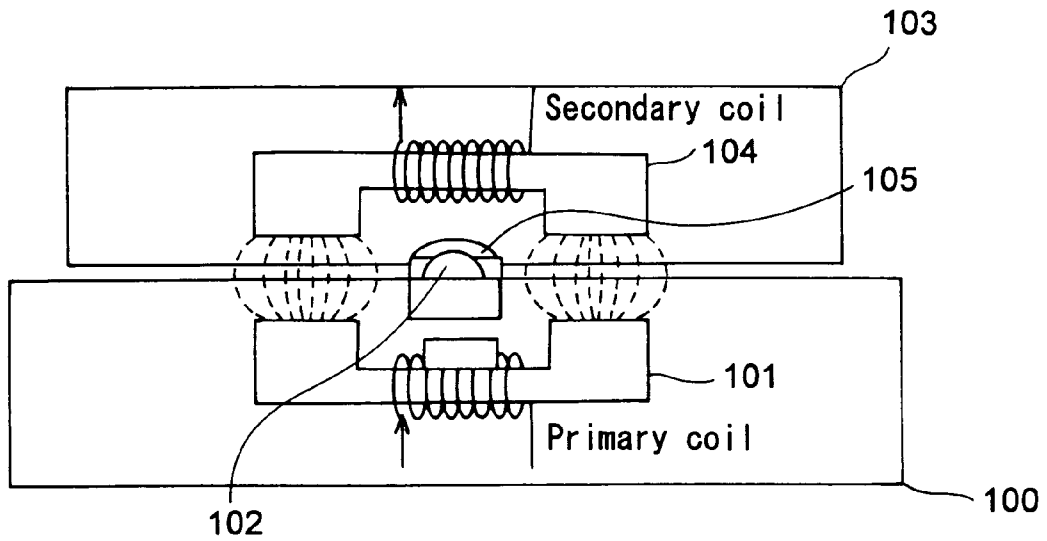
FIG. 12 PRIOR ART
