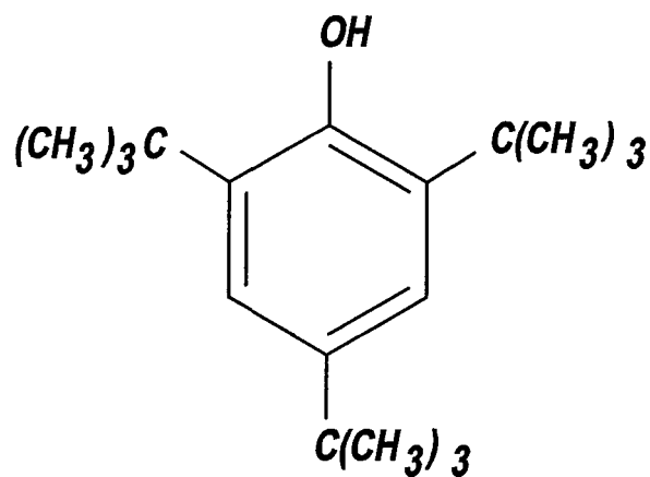
Butylated hydroxytoluene
