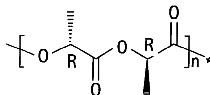
poly (D-lactide)
